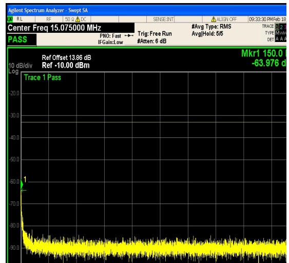
1-N25-PC3-15-20-M-14-DFT-256QAM-Edge _1RB_Right-1@105-0.15-30-Ant1--63.98--33 -PASS
