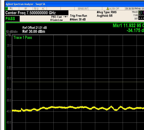
1-N25-PC3-15-20-M-16-CP-QPSK-Edge_1R B_Left-1@0-3000-12000-Ant1--34.17--13-PASS
