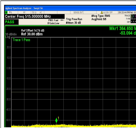
1-N25-PC3-15-20-M-14-DFT-256QAM-Edge _1RB_Right-1@105-30-1000-Ant1--53.09--2 3-PASS
