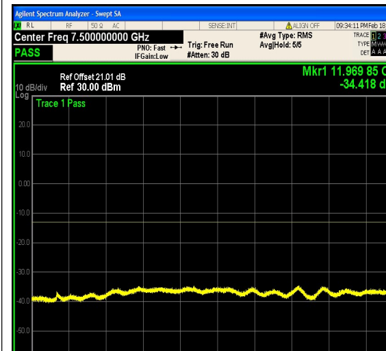
1-N25-PC3-15-20-M-14-DFT-256QAM-Edge _1RB_Right-1@105-3000-12000-Ant1--34.42 --13-PASS
