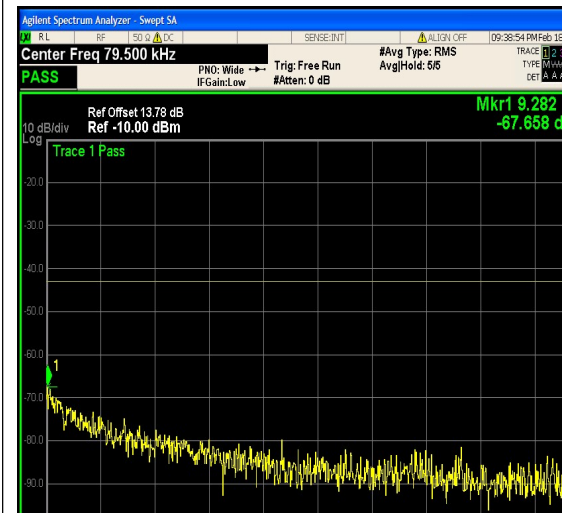
1-N25-PC3-15-20-M-18-CP-QPSK-Outer_Ful l-106@0-0.009-0.15-Ant1--67.66--43-PASS
