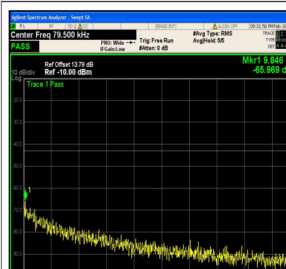
1-N25-PC3-15-20-M-13-DFT-256QAM-Edge _1RB_Left-1@0-0.009-0.15-Ant1--65.97--43- PASS
