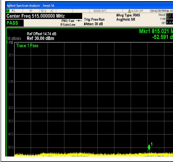
1-N25-PC3-15-20-M-20-CP-16QAM-Edge_1 RB_Right-1@105-30-1000-Ant1--52.59--23-P ASS
