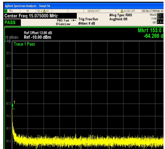
1-N25-PC3-15-20-M-15-DFT-256QAM-Outer _Full-100@0-12000-20000-Ant1--25.86--13- PASS
