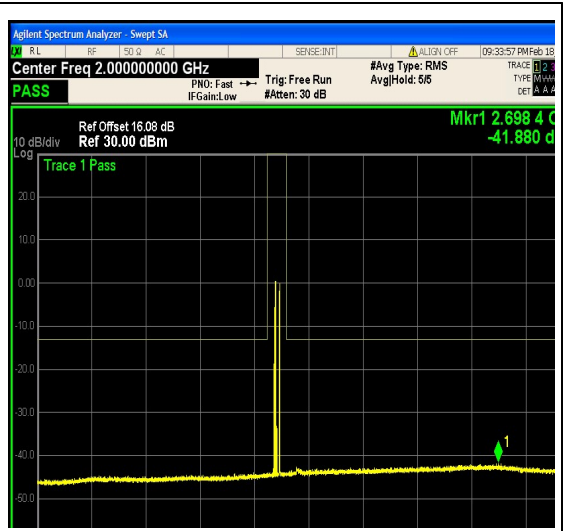
1-N25-PC3-15-20-M-14-DFT-256QAM-Edge _1RB_Right-1@105-1000-3000-Ant1--41.88- -13-PASS
