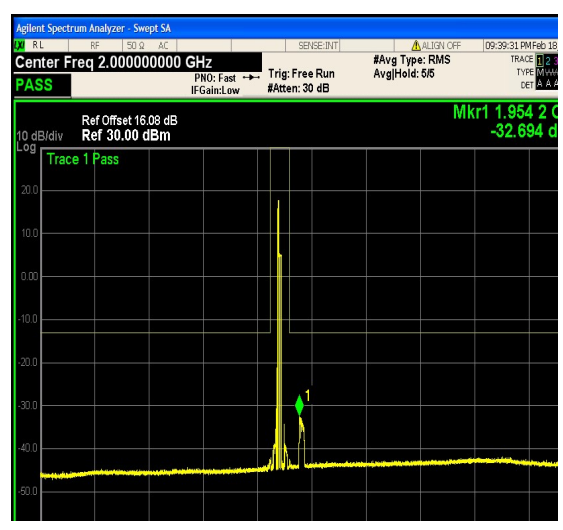
1-N25-PC3-15-20-M-18-CP-QPSK-Outer_Ful l-106@0-0.15-30-Ant1--32.69--33-PASS
