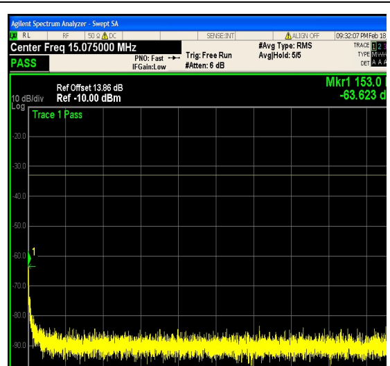
1-N25-PC3-15-20-M-13-DFT-256QAM-Edge _1RB_Left-1@0-0.15-30-Ant1--63.62--33-PA SS
