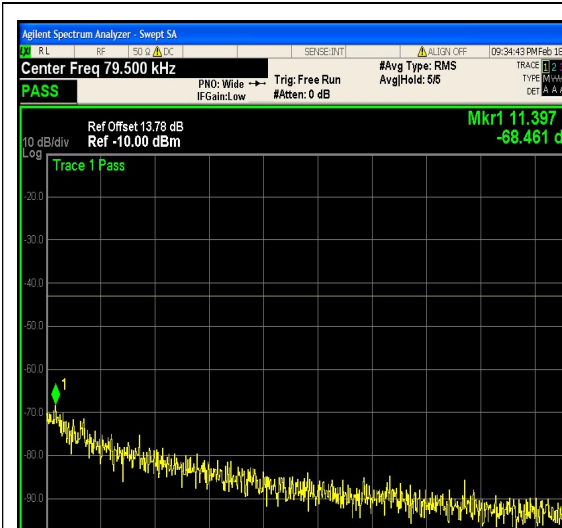
1-N25-PC3-15-20-M-15-DFT-256QAM-Outer _Full-100@0-0.009-0.15-Ant1--68.46--43-PA SS
