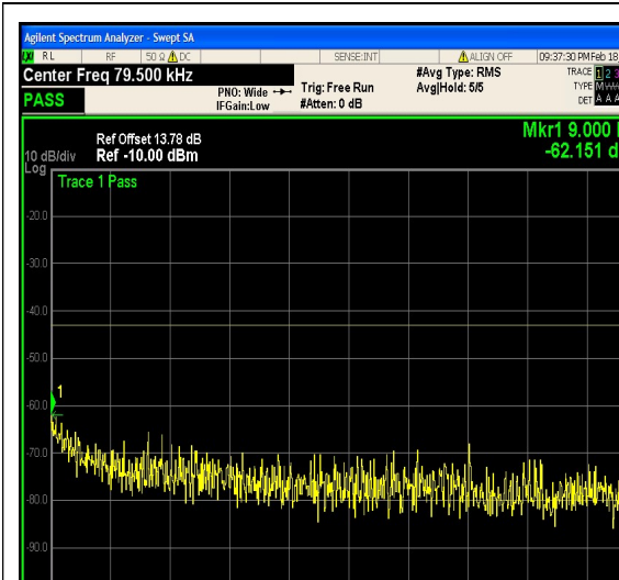
1-N25-PC3-15-20-M-17-CP-QPSK-Edge_1R B_Right-1@105-0.009-0.15-Ant1--62.15--43- PASS
