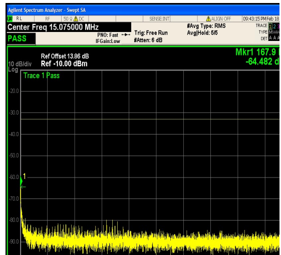
1-N25-PC3-15-20-M-21-CP-16QAM-Outer_F ull-106@0-0.15-30-Ant1--64.48--33-PASS
