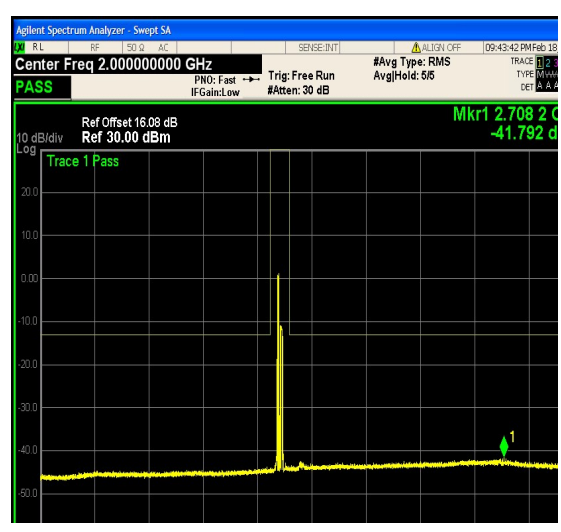
1-N25-PC3-15-20-M-21-CP-16QAM-Outer_F ull-106@0-0.15-30-Ant1--64.48--33-PASS
