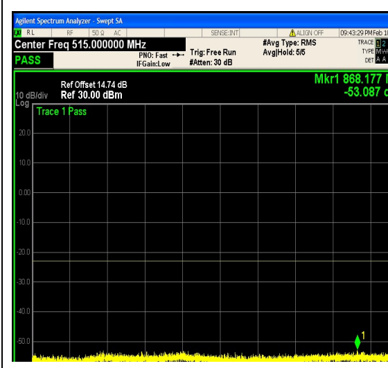
1-N25-PC3-15-20-M-21-CP-16QAM-Outer_F ull-106@0-0.009-0.15-Ant1--68.27--43-PASS
