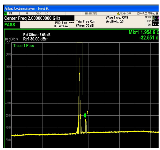
1-N25-PC3-15-20-M-24-CP-64QAM-Outer_F ull-106@0-0.15-30-Ant1--65.06--33-PASS
