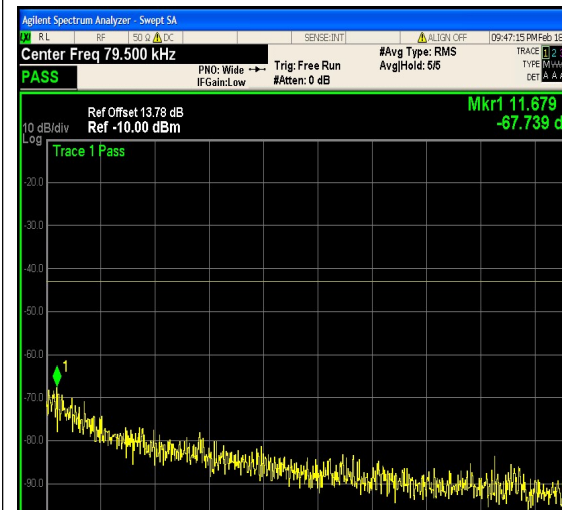
1-N25-PC3-15-20-M-24-CP-64QAM-Outer_F ull-106@0-0.009-0.15-Ant1--67.74--43-PASS
