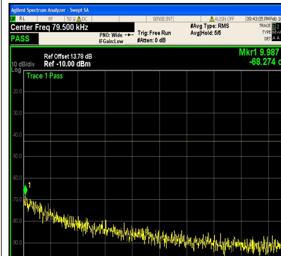
1-N25-PC3-15-20-M-21-CP-16QAM-Outer_F ull-106@0-0.009-0.15-Ant1--68.27--43-PASS
