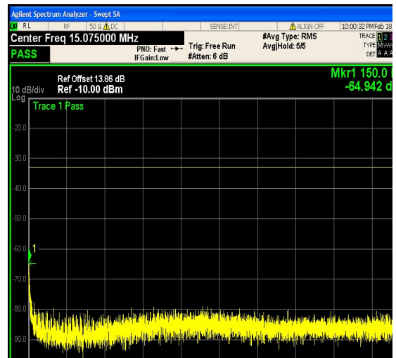
1-N25-PC3-15-20-H-6-DFT-QPSK-Outer_Full -100@0-0.15-30-Ant1--64.94--33-PASS
