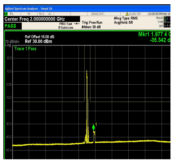
1-N25-PC3-15-20-H-6-DFT-QPSK-Outer_Full -100@0-0.15-30-Ant1--64.94--33-PASS
