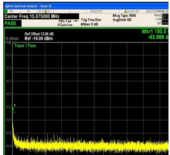
1-N25-PC3-15-20-H-18-CP-QPSK-Outer_Ful l-106@0-0.15-30-Ant1--64.00--33-PASS
