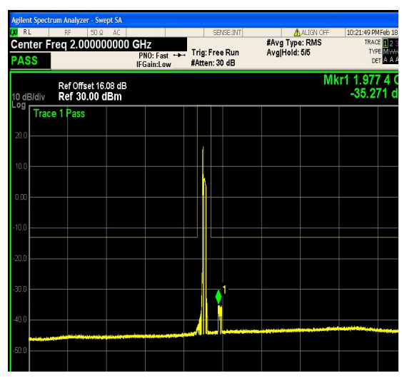
1-N25-PC3-15-20-H-21-CP-16QAM-Outer_F ull-106@0-0.15-30-Ant1--66.00--33-PASS
