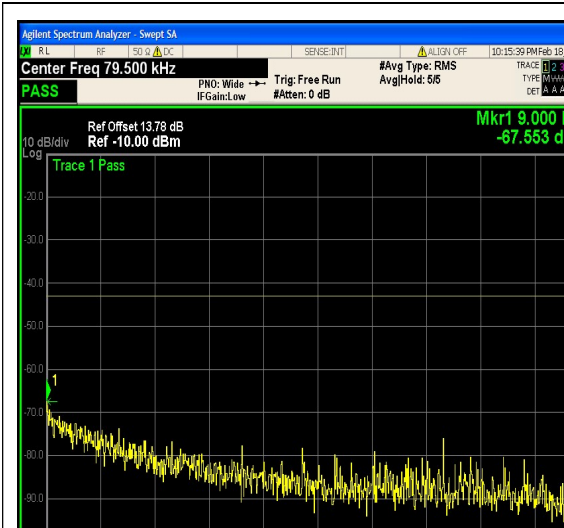
1-N25-PC3-15-20-H-17-CP-QPSK-Edge_1R B_Right-1@105-0.009-0.15-Ant1--67.55--43- PASS
