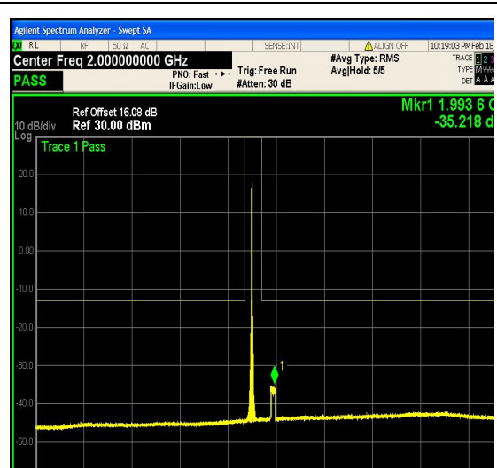
1-N25-PC3-15-20-H-19-CP-16QAM-Edge_1 RB_Left-1@0-1000-3000-Ant1--35.22--13-PA SS
