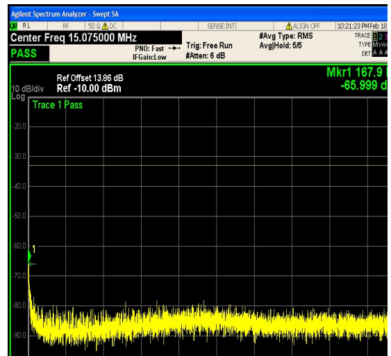
1-N25-PC3-15-20-H-21-CP-16QAM-Outer_F ull-106@0-0.15-30-Ant1--66.00--33-PASS
