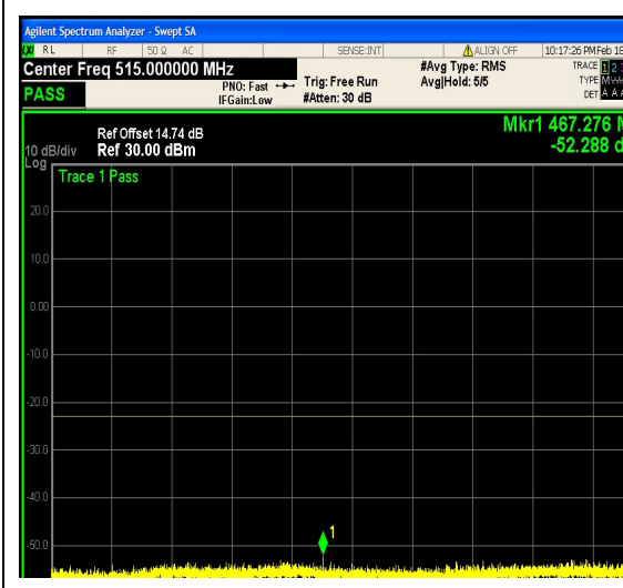
1-N25-PC3-15-20-H-18-CP-QPSK-Outer_Ful l-106@0-0.009-0.15-Ant1--67.48--43-PASS
