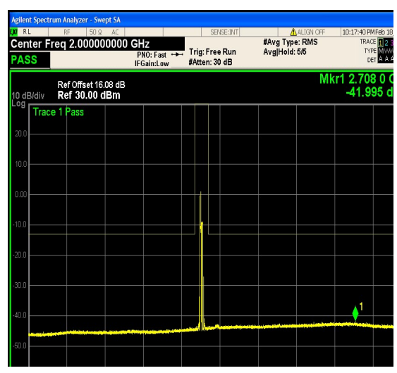
1-N25-PC3-15-20-H-18-CP-QPSK-Outer_Ful l-106@0-0.15-30-Ant1--64.00--33-PASS
