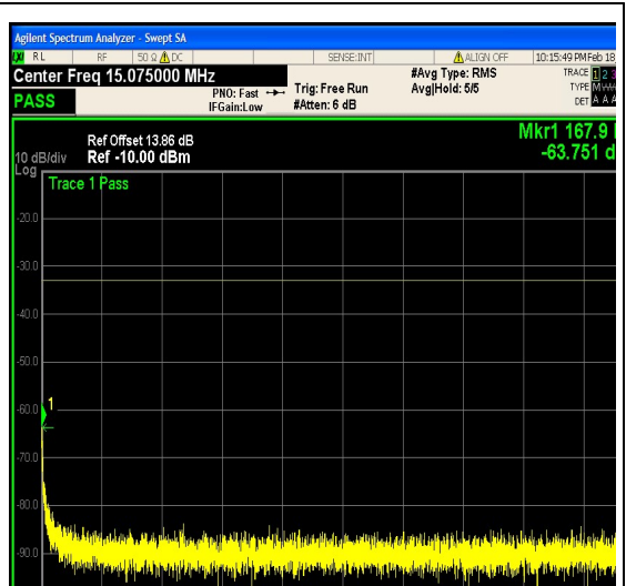
1-N25-PC3-15-20-H-17-CP-QPSK-Edge_1R B_Right-1@105-0.15-30-Ant1--63.75--33-PA SS
