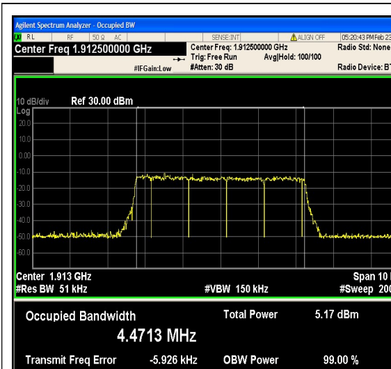
1-N25-PC3-15-5-H-5-CP-QPSK-Outer_Full-2 5@0-Ant1-4.4713-4.867-≤5-PASS
