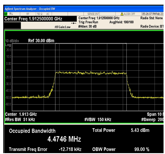
1-N25-PC3-15-5-H-8-CP-256QAM-Outer_Full-125@0-Ant1-4.4746-4.845-≤5-PASS
