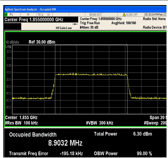
1-N25-PC3-15-10-L-2-DFT-PI2BPSK-Outer_Full
