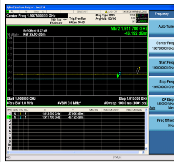
1-N2-PC3-15-5-H-1-DFT-PI2BPSK-Outer_Fu
