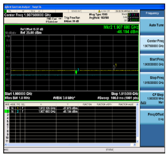
1-N2-PC3-15-5-H-2-DFT-QPSK-Outer_Full-2
