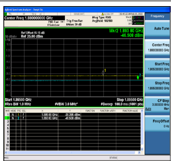
1-N2-PC3-15-10-M-8-CP-64QAM-Outer_Full-52@0-Ant1-8.11-1%-20.00--11.89-PASS-≤13
