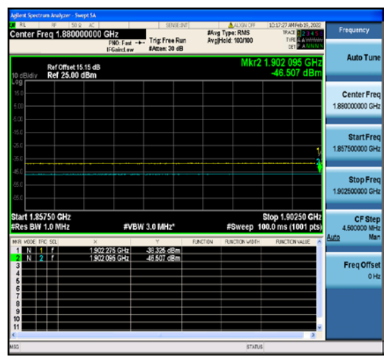
1-N2-PC3-15-15-M-1-DFT-PI2BPSK-Outer_Full-75@0-Ant1-8.18-1%-20.00--11.82-PASS-≤
