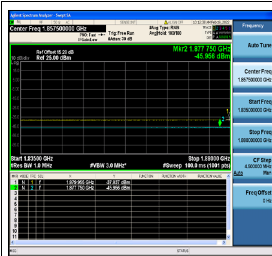
1-N2-PC3-15-15-L-7-CP-16QAM-Outer_Full-79@0-Ant1-8.12-1%-20.00--11.88-PASS-≤13
