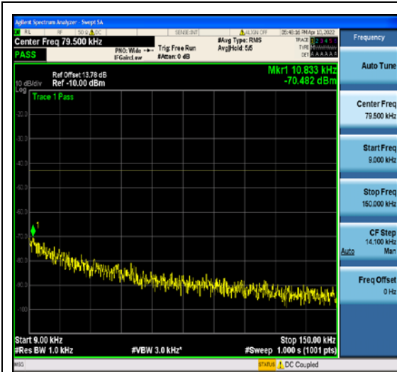
1-N2-PC3-15-5-H-4-DFT-QPSK-Edge_1RB_ Left-1@0-0.009-0.15-Ant1--70.48--43-PASS
