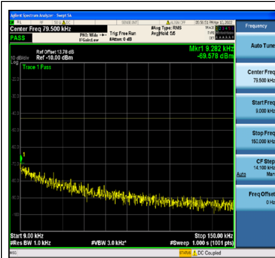
1-N2-PC3-15-10-M-4-DFT-QPSK-Edge_1RB _Left-1@0-0.009-0.15-Ant1--69.58--43-PASS
