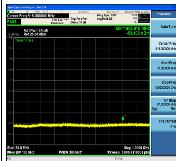
1-N2-PC3-15-5-L-4-DFT-QPSK-Edge_1RB_L eft-1@0-30-1000-Ant1--53.11--23-PASS
