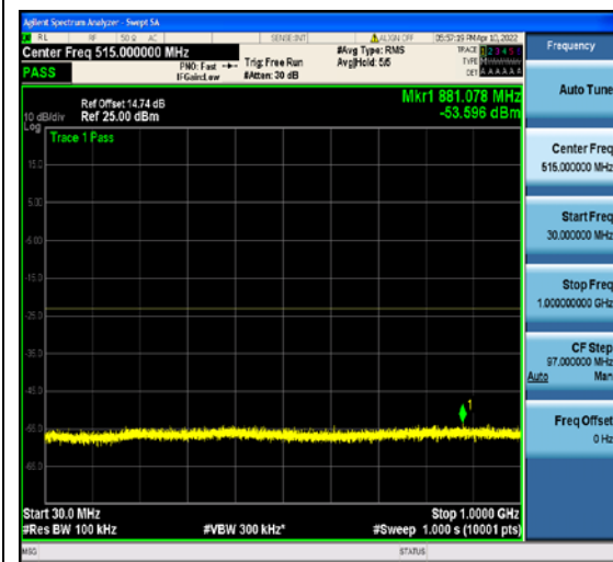
1-N2-PC3-15-10-M-4-DFT-QPSK-Edge_1RB _Left-1@0-30-1000-Ant1--53.60--23-PASS
