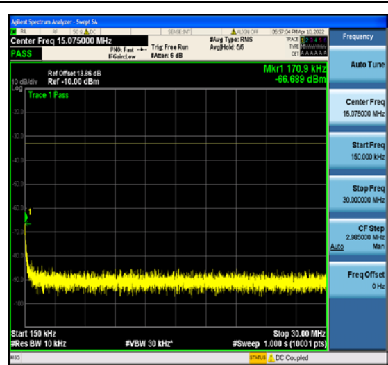
1-N2-PC3-15-10-M-4-DFT-QPSK-Edge_1RB _Left-1@0-0.15-30-Ant1--66.69--33-PASS
