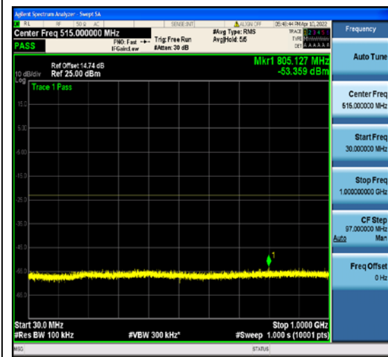
1-N2-PC3-15-5-H-4-DFT-QPSK-Edge_1RB_ Left-1@0-30-1000-Ant1--53.36--23-PASS
