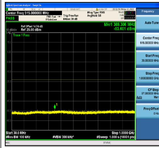
1-N2-PC3-15-10-L-4-DFT-QPSK-Edge_1RB_ Left-1@0-0.009-0.15-Ant1--62.73--43-PASS
