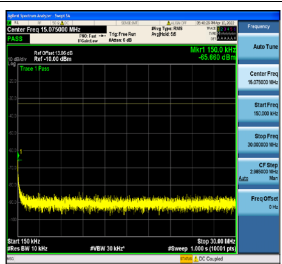
1-N2-PC3-15-5-H-4-DFT-QPSK-Edge_1RB_ Left-1@0-0.15-30-Ant1--65.66--33-PASS
