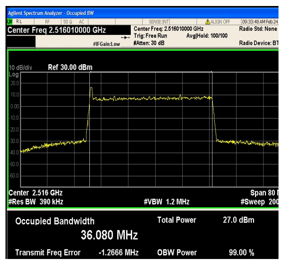
1-N41-PC2-30-40-L-2-DFT-PI2BPSK-Outer_Full
