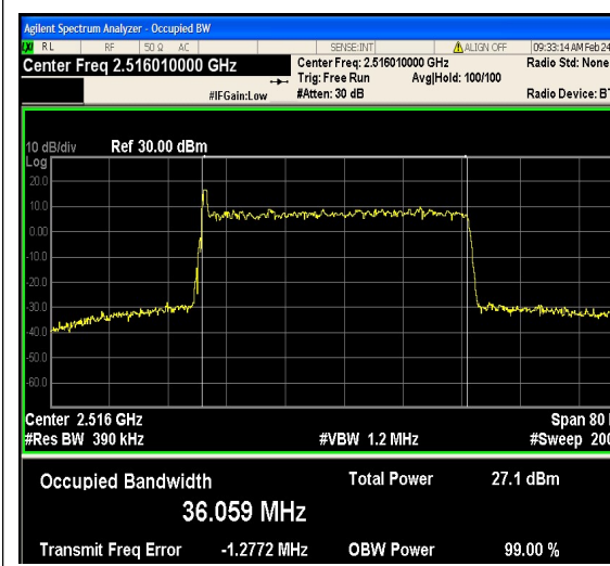
1-N41-PC2-30-40-L-1-DFT-QPSK-Outer_Full
