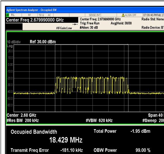
1-N41-PC2-30-20-H-5-CP-QPSK-Outer_Full-51@0-Ant1-18.429-39.98-<20-PASS
