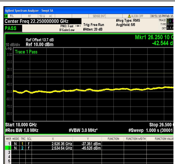
1-N41-PC2-30-20-L-11-DFT-64QAM-Edge_1 RB_Right-1@50-18000-26500-Ant1--42.54-- 25-PASS
