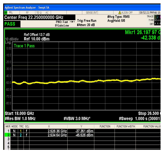
1-N41-PC2-30-20-L-12-DFT-64QAM-Outer_F ull-50@0-1000-3000-Ant1--41.92--25-PASS
