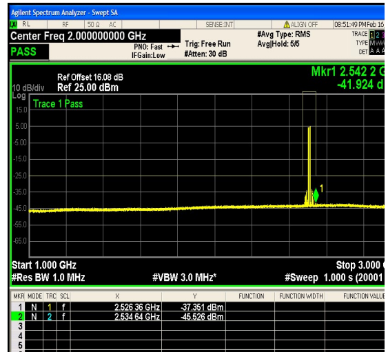
1-N41-PC2-30-20-L-12-DFT-64QAM-Outer_F ull-50@0-1000-3000-Ant1--41.92--25-PASS
