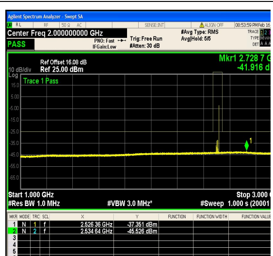
1-N41-PC2-30-20-L-14-DFT-256QAM-Edge_1RB_Right-1@50-1000-3000-Ant1--41.92--25-PASS
