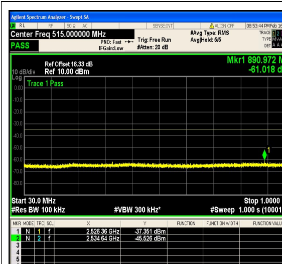
1-N41-PC2-30-20-L-14-DFT-256QAM-Edge_1RB_Right-1@50-30-1000-Ant1--61.02--35-PASS
