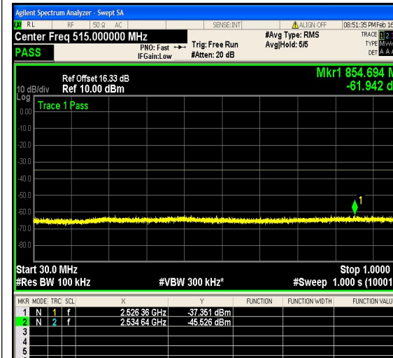
1-N41-PC2-30-20-L-12-DFT-64QAM-Outer_F ull-50@0-30-1000-Ant1--61.94--35-PASS
