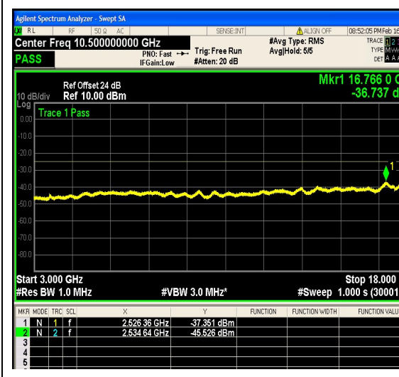
1-N41-PC2-30-20-L-12-DFT-64QAM-Outer_F ull-50@0-30-1000-Ant1--61.94--35-PASS
