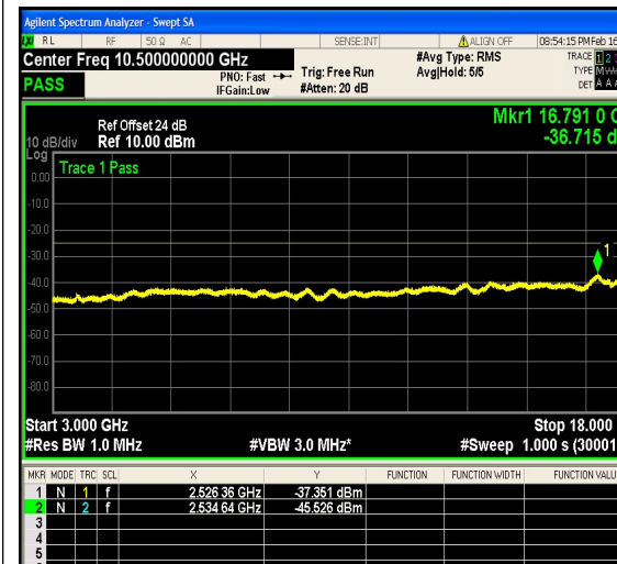
1-N41-PC2-30-20-L-14-DFT-256QAM-Edge_1RB_Right-1@50-3000-18000-Ant1--36.71--25-PASS
