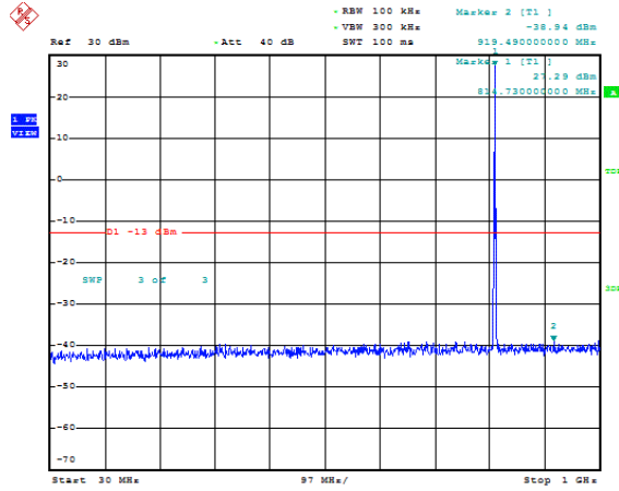
Band26-1.4MHz-QPSK-26697-1RB#0-Range1:30~1000MHz
