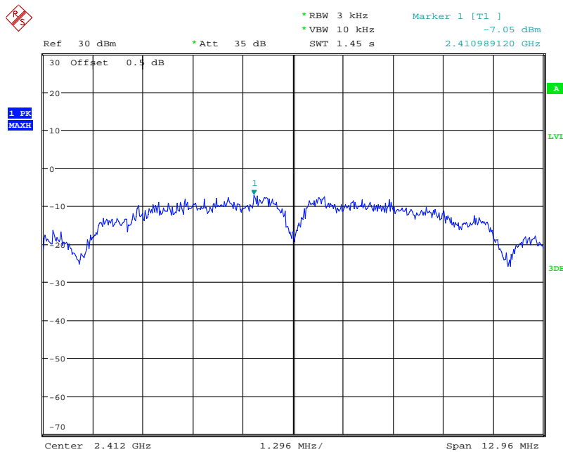
Power Spectral Density, 802.11b Low Channel
