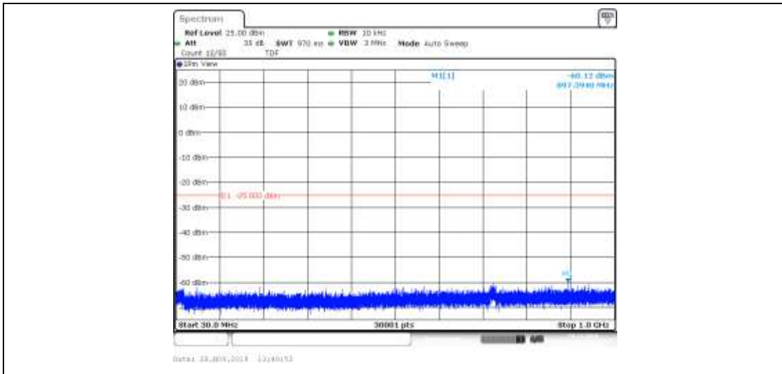
Band41_5MHz_QPSK_40265_1RB#0
