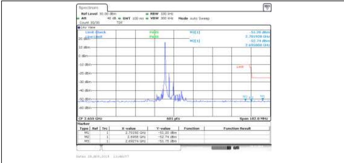
Band41_5MHz_16QAM_41215_1RB#12
