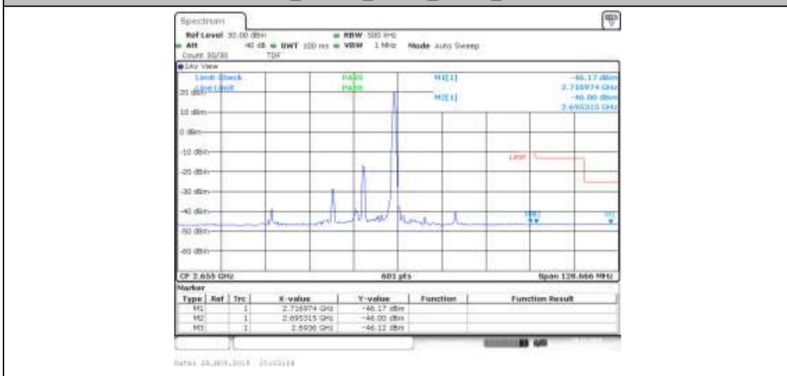
Band41_20MHz_QPSK_41140_1RB#99
