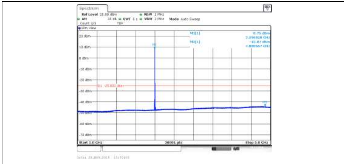
Band41_5MHz_16QAM_40690_1RB#0
