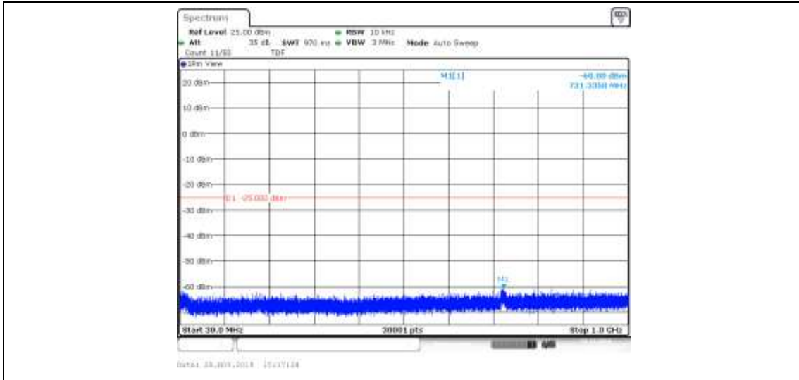
Band41_20MHz_QPSK_41140_1RB#0
