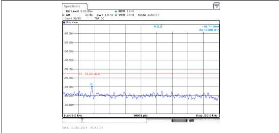
Band41_20MHz_16QAM_40690_1RB#0
