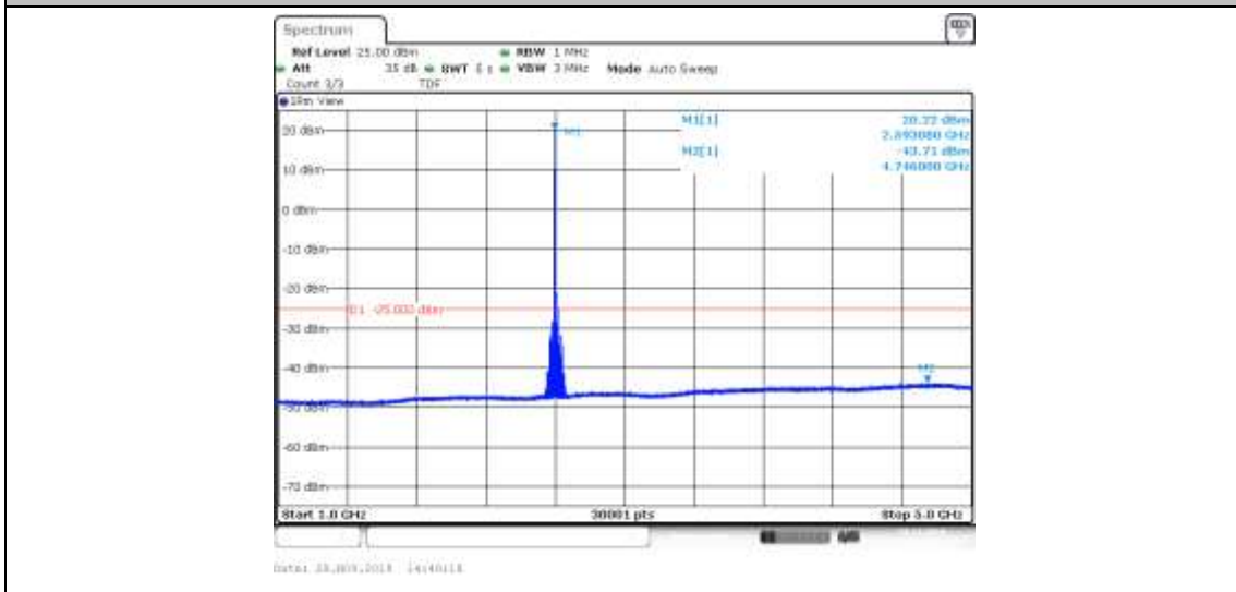
Band41_15MHz_16QAM_40690_1RB#0
