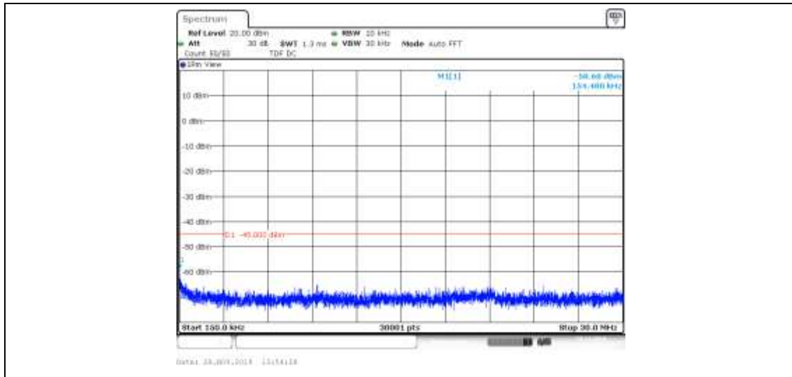
Band41_5MHz_QPSK_40690_1RB#0
