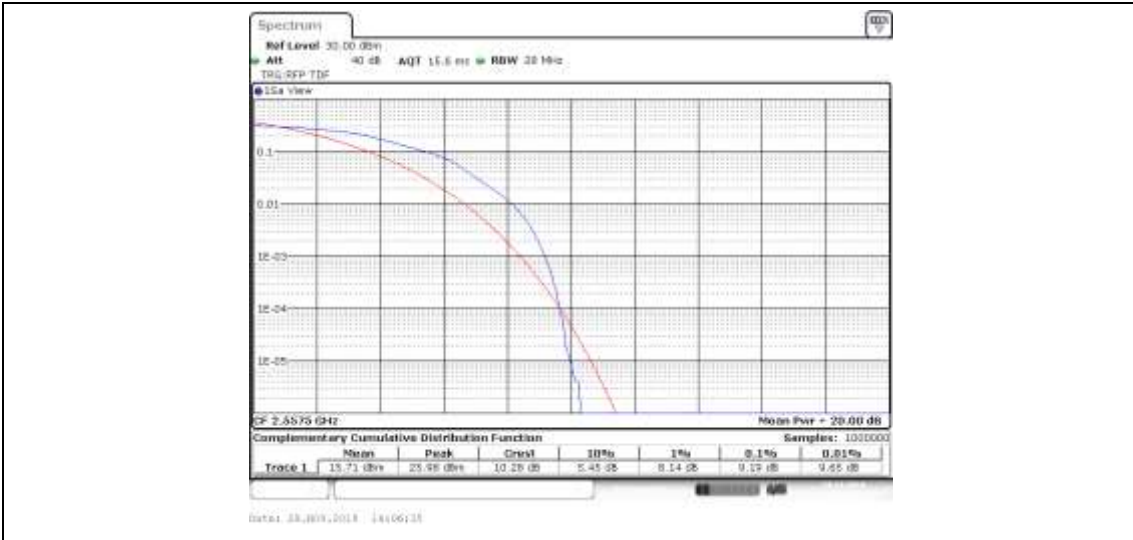
Band41_5MHz_16QAM_40690_1RB#0
