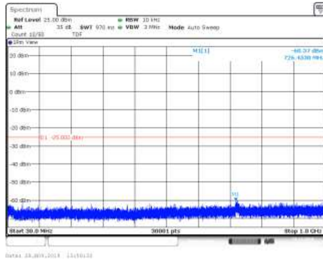
Band41_5MHz_16QAM_40690_1RB#0
