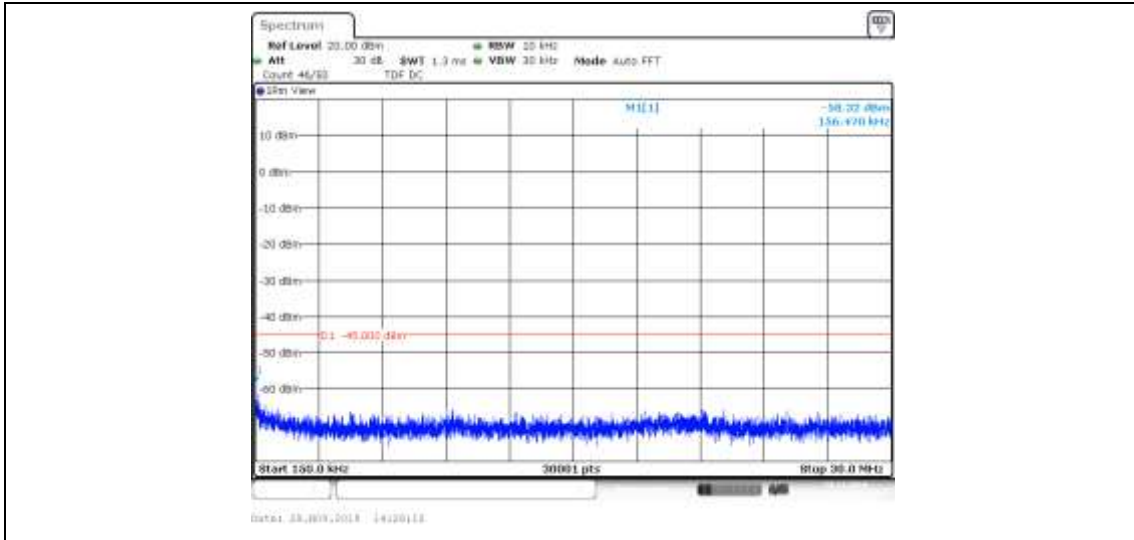
Band41_10MHz_16QAM_41190_1RB#0
