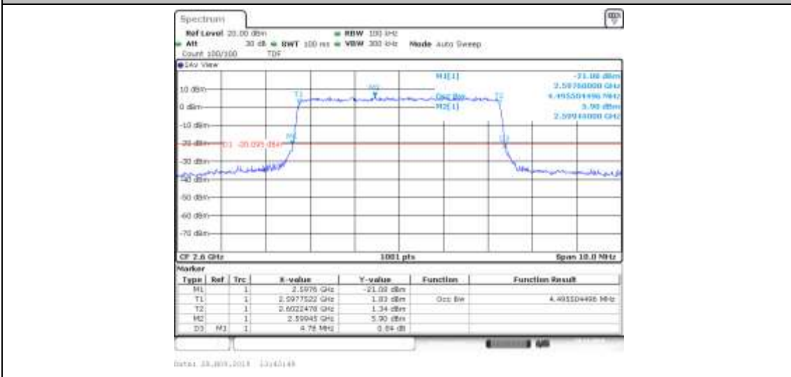
Band41_5MHz_16QAM_40690_25RB#0
