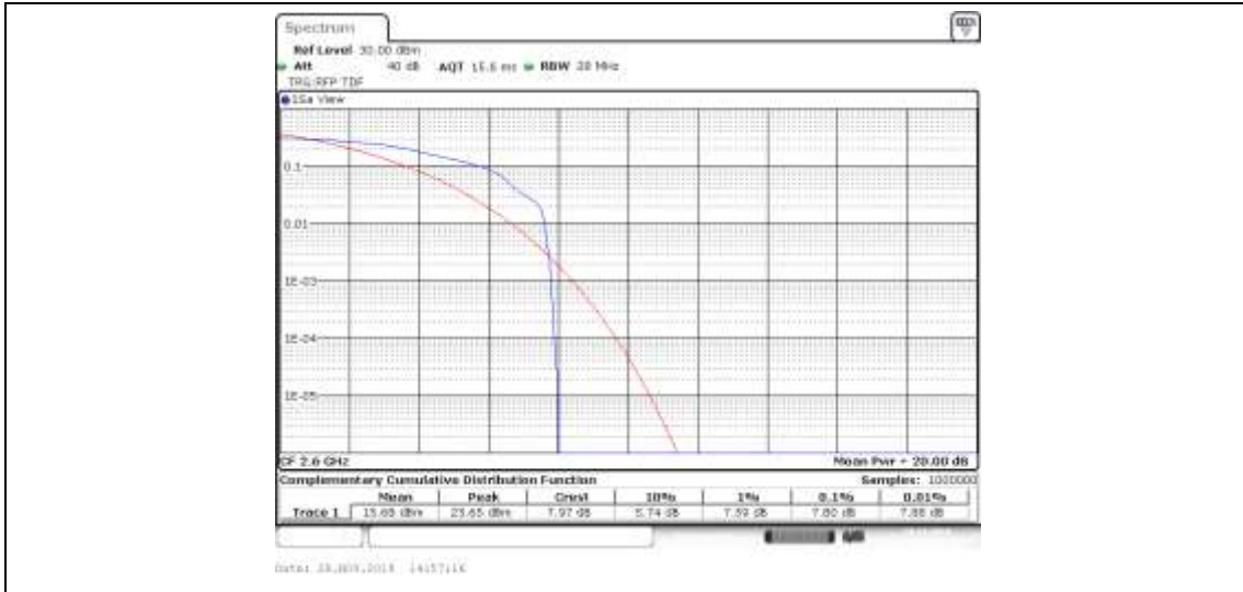
Band41_15MHz_16QAM_40690_75RB#0
