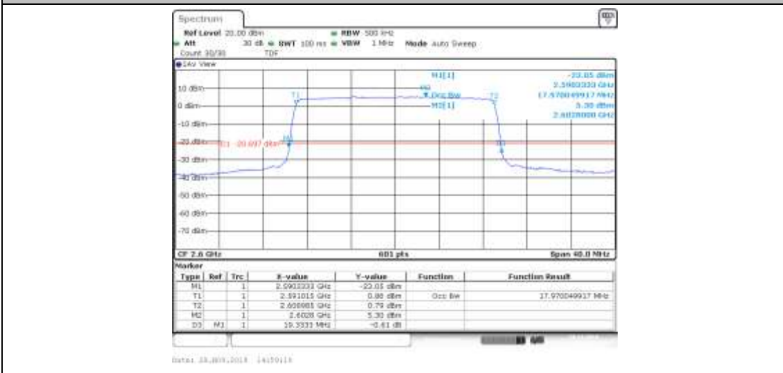
Band41_20MHz_QPSK_40690_100RB#0
