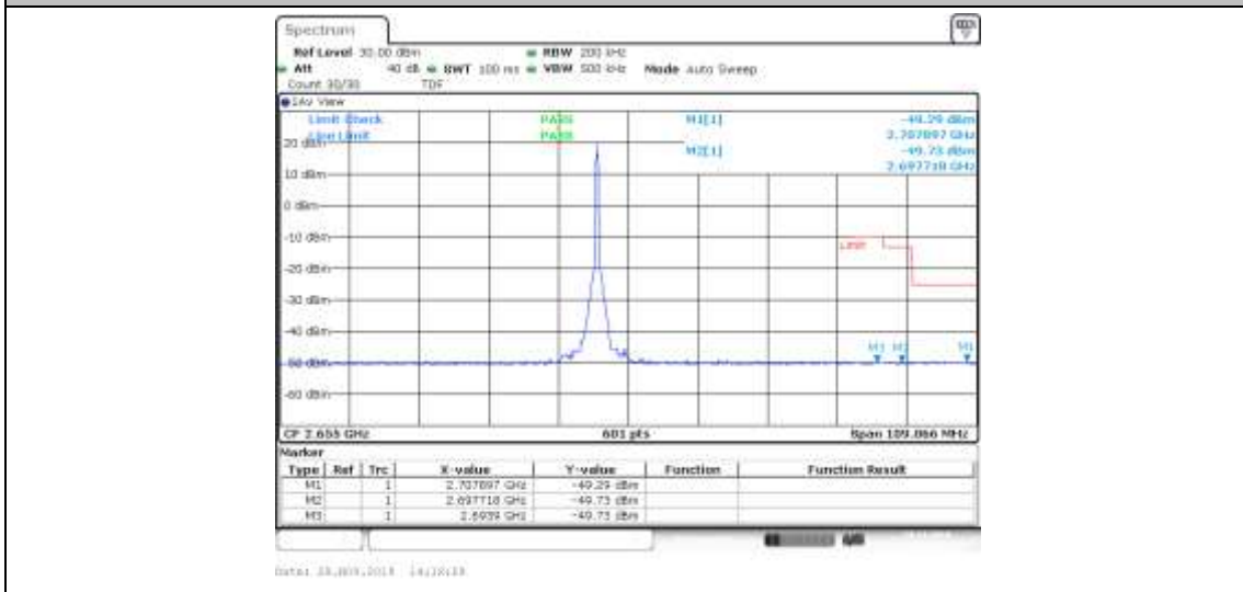
Band41_10MHz_16QAM_41190_1RB#24
