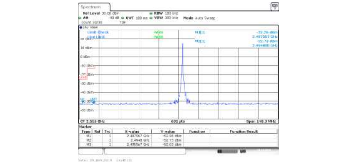
Band41_5MHz_QPSK_40265_1RB#24
