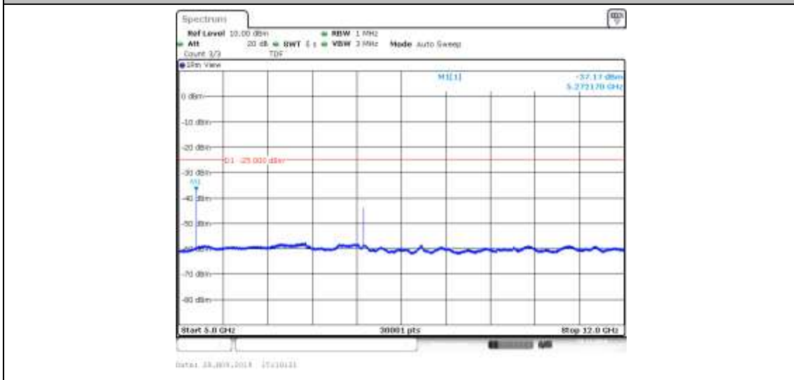
Band41_20MHz_QPSK_41140_1RB#0
