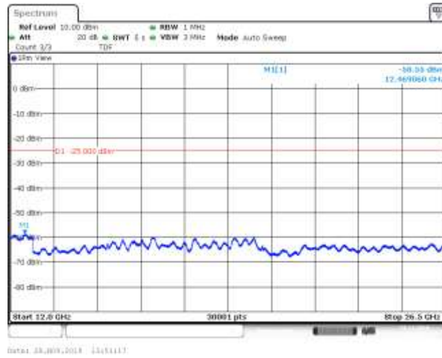
Band41_5MHz_QPSK_40690_1RB#0
