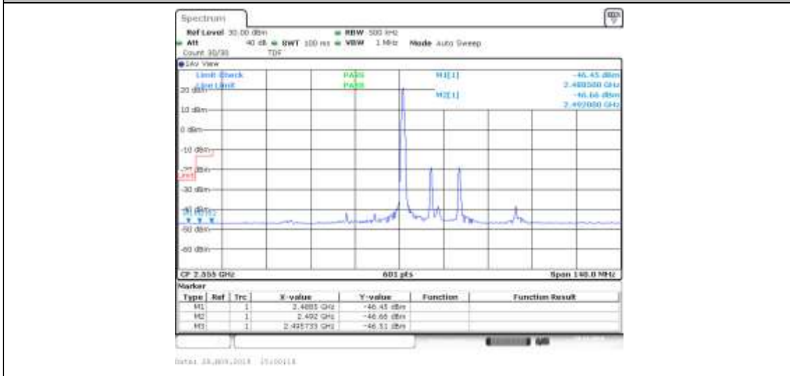
Band41_20MHz_QPSK_40340_1RB#49
