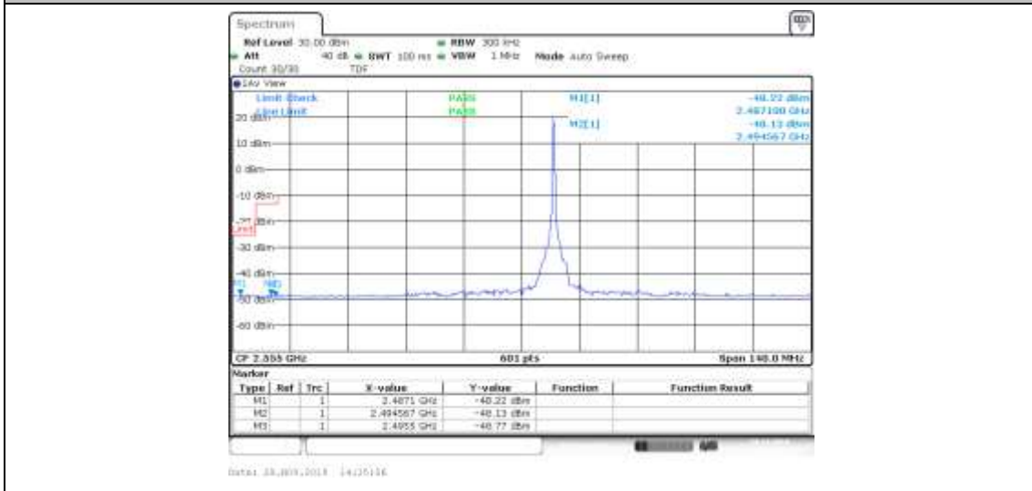
Band41_15MHz_QPSK_40315_1RB#74
