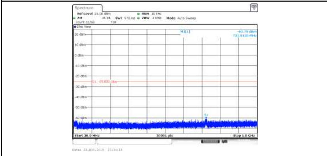
Band41_20MHz_16QAM_40690_1RB#0
