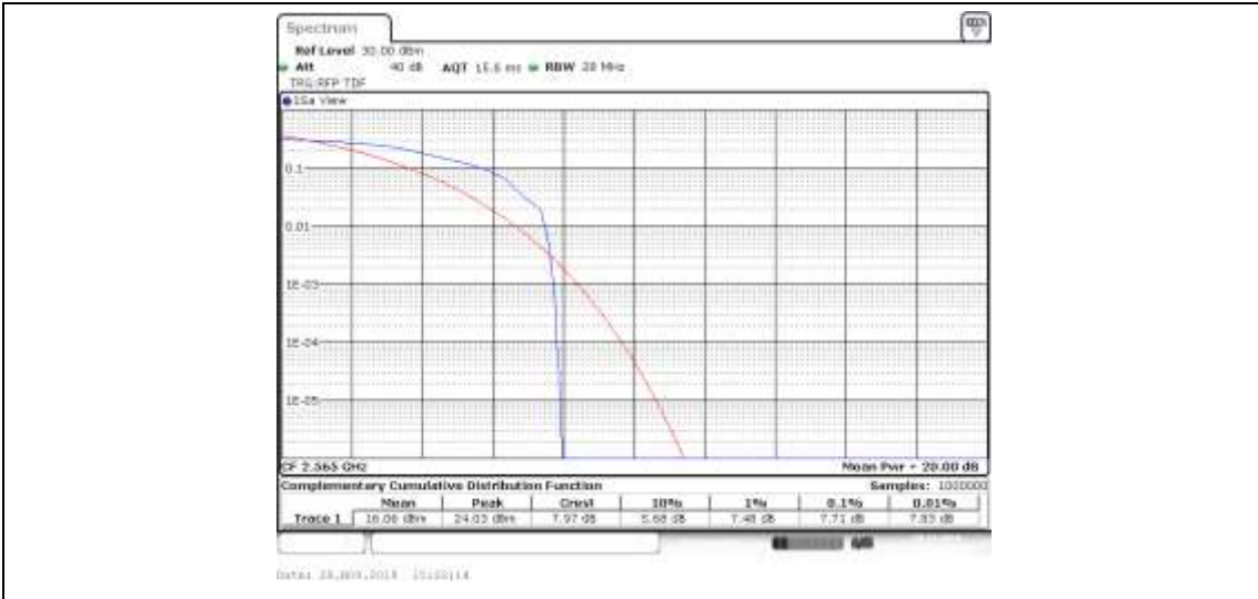
Band41_20MHz_16QAM_40340_100RB#0
