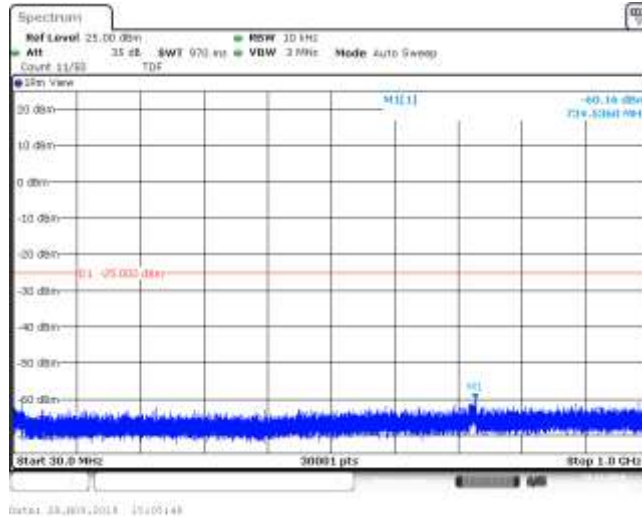
Band41_20MHz_QPSK_40340_1RB#0
