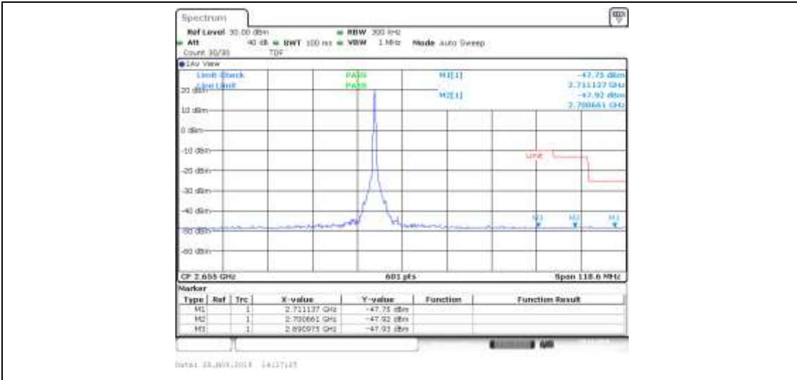
Band41_15MHz_QPSK_41165_1RB#74
