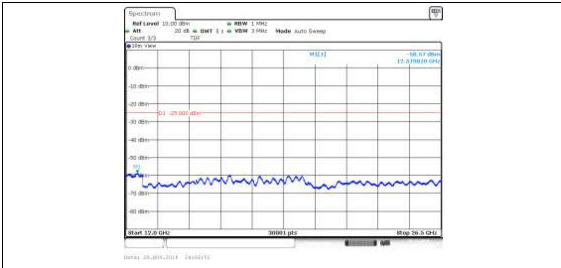
Band41_5MHz_16QAM_40265_1RB#0
