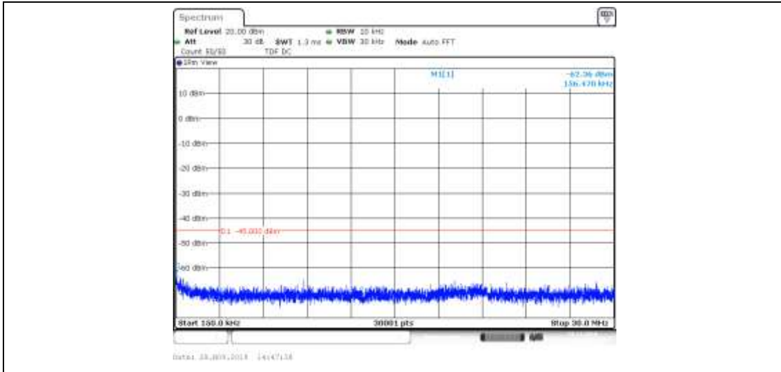
Band41_15MHz_16QAM_40690_1RB#0
