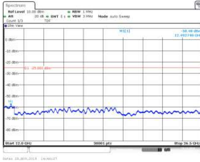
Band41_15MHz_16QAM_40690_1RB#0
