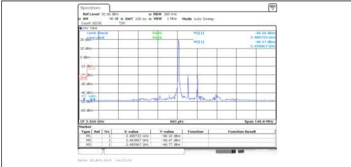
Band41_15MHz_QPSK_40315_1RB#38
