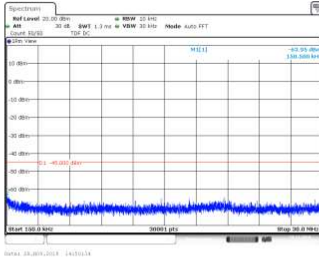
Band41_15MHz_QPSK_41165_1RB#0
