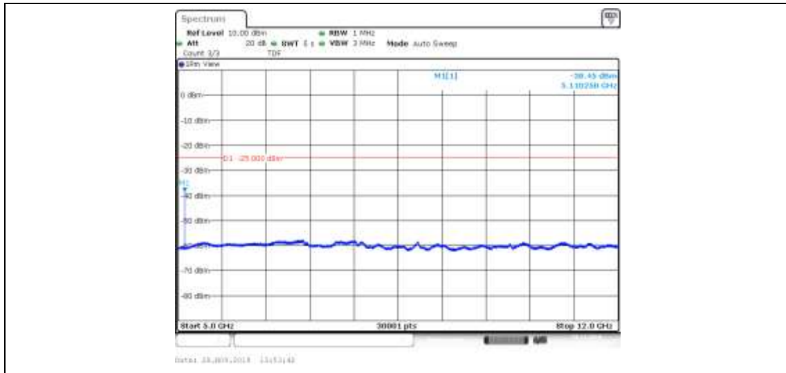
Band41_5MHz_16QAM_40265_1RB#0
