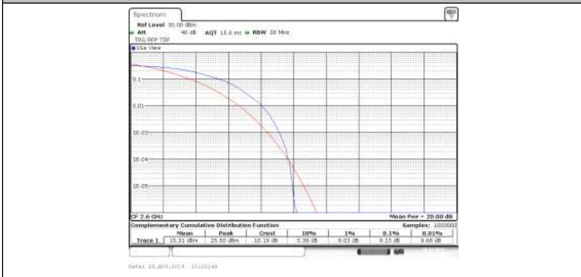
Band41_20MHz_QPSK_40690_100RB#0
