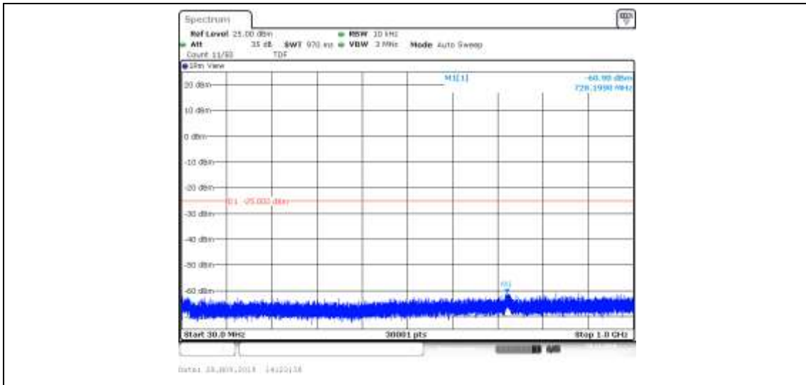
Band41_10MHz_16QAM_40690_1RB#0
