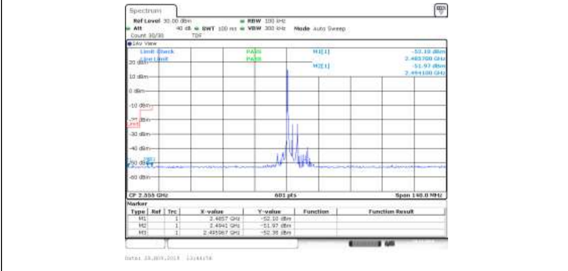
Band41_5MHz_QPSK_40265_1RB#12
