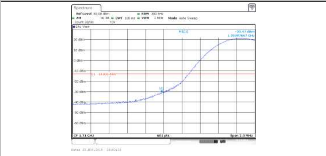
Band4_15MHz_QPSK_20025_1RB#38
