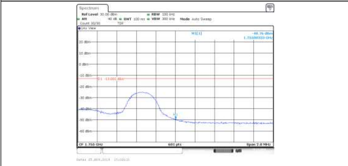
Band4_5MHz_QPSK_20375_1RB#12
