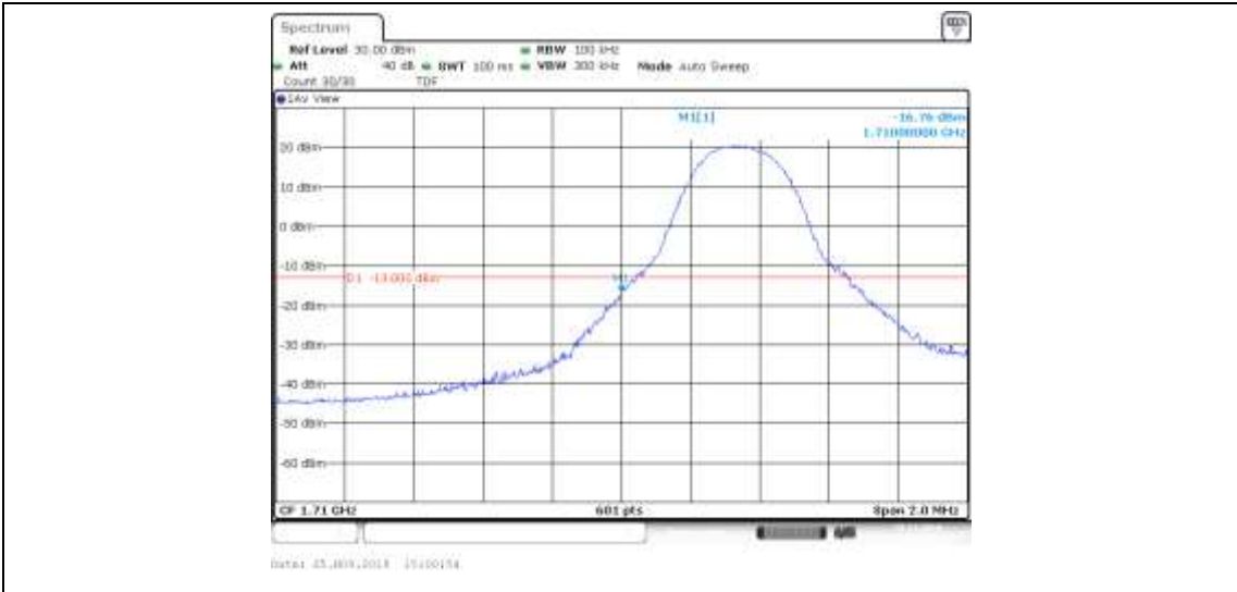
Band4_5MHz_QPSK_19975_1RB#12
