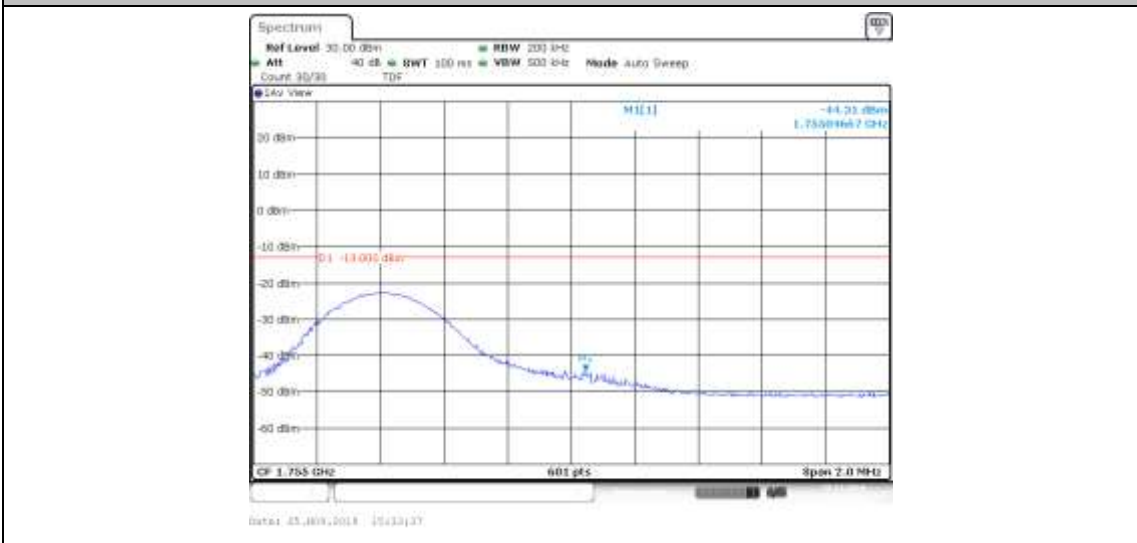
Band4_10MHz_QPSK_20350_1RB#24
