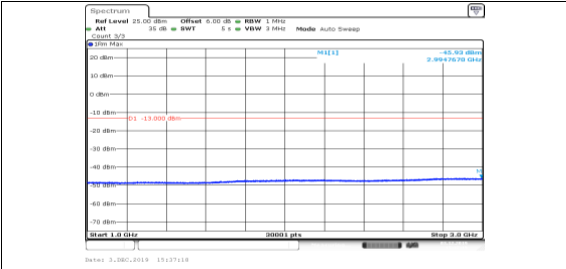
Band V-4182-HSDPA_Sub4-1000~3000
