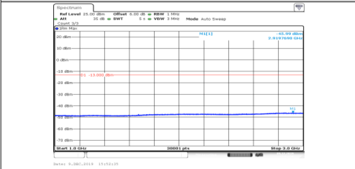
Band V-4182-HSUPA_Sub2-1000~3000
