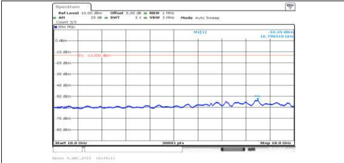
Band V-4182-HSUPA_Sub5-10000~18000
