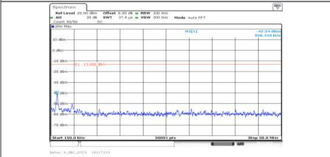
Band V-4233-HSUPA_Sub3-0.15~30
