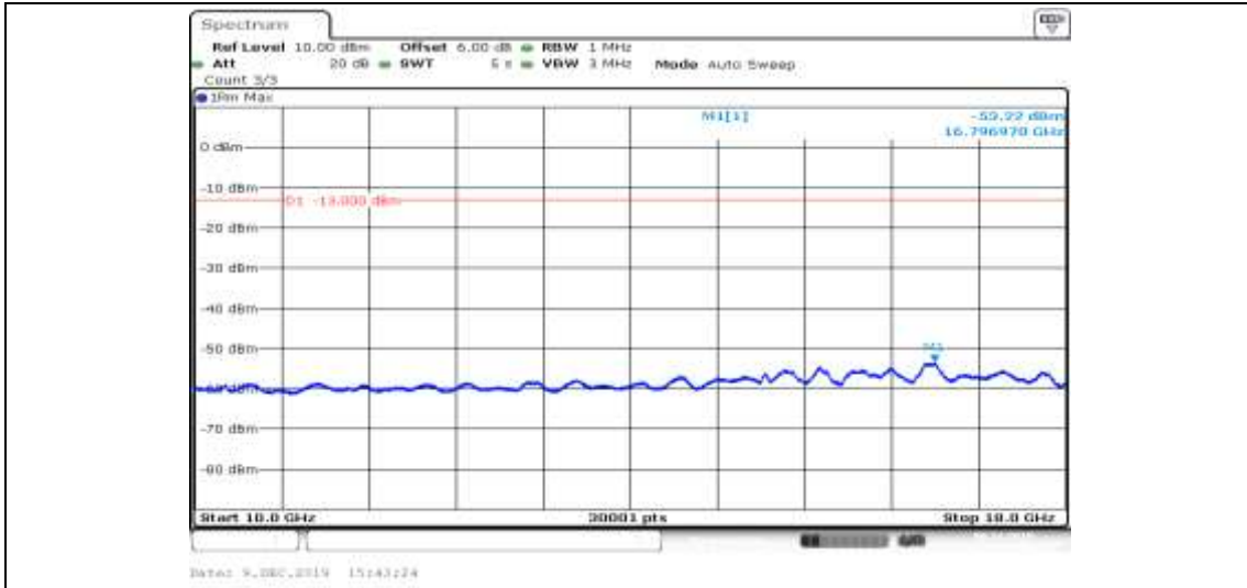
Band V-4132-HSUPA_Sub5-10000~18000
