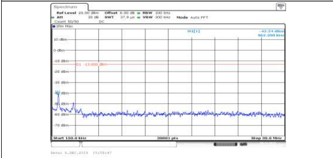
Band V-4182-HSUPA_Sub5-0.15~30
