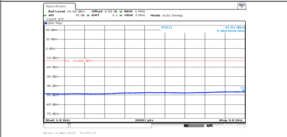
Band V-4132-HSUPA_Sub2-1000~3000
