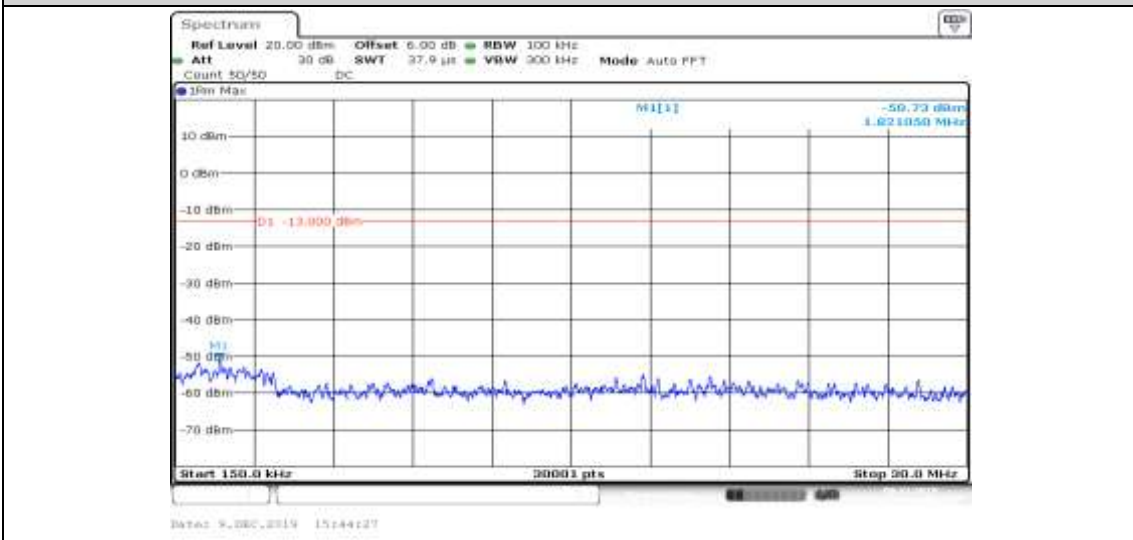
Band V-4132-HSUPA_Sub3-0.15~30
