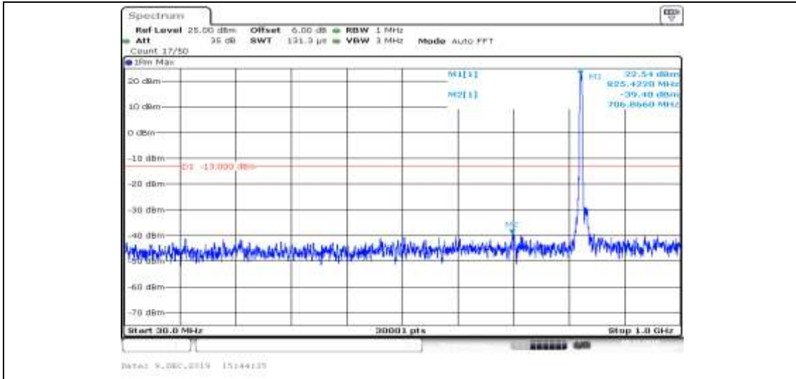
Band V-4132-HSUPA_Sub2-30~1000
