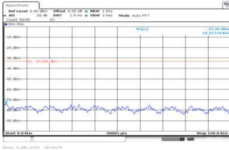
Band V-4233-HSUPA_Sub4-0.009~0.15
