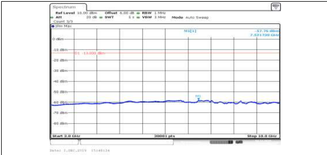
Band V-4233-HSDPA_Sub3-3000~10000
