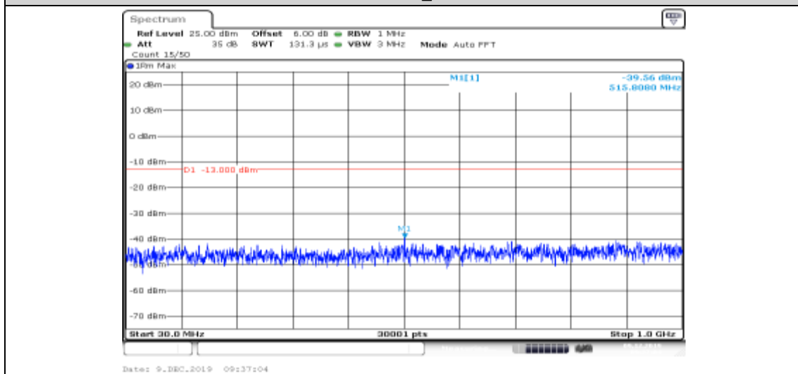
Band II-9538-HSUPA_Sub3-30~1000
