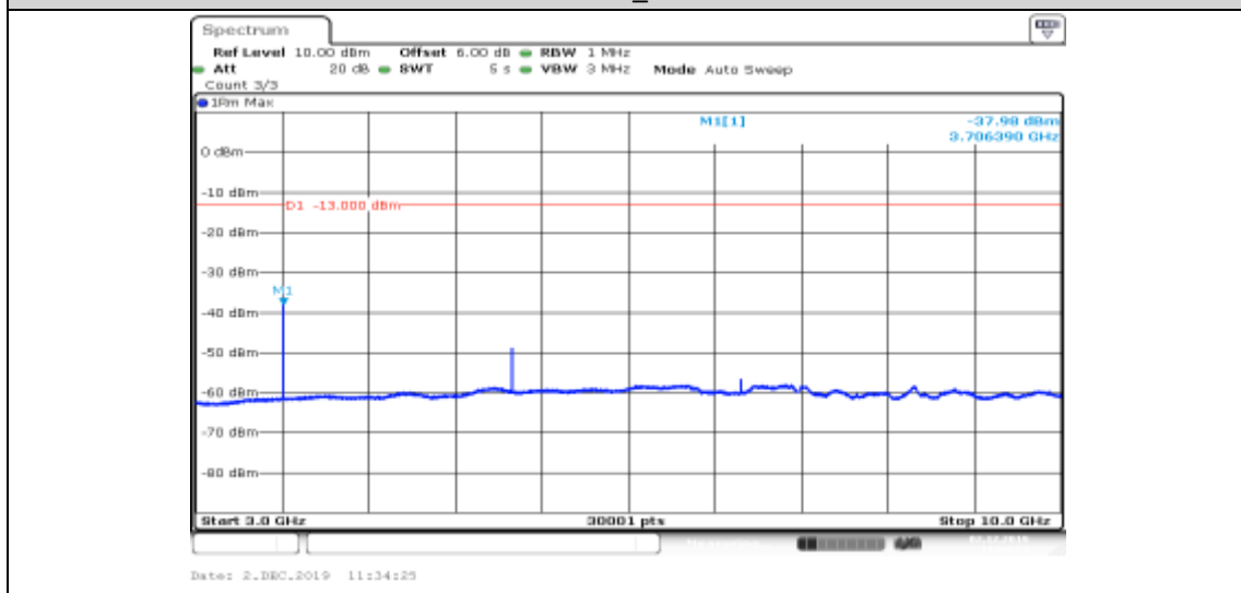
Band II-9262-HSDPA_Sub4-3000~10000
