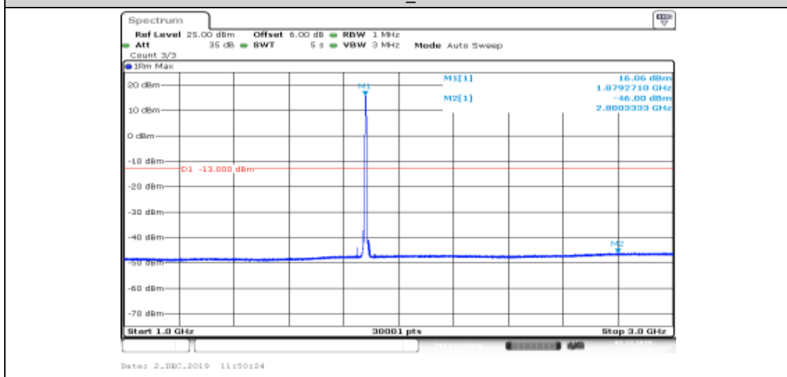
Band II-9400-HSDPA_Sub4-1000~3000
