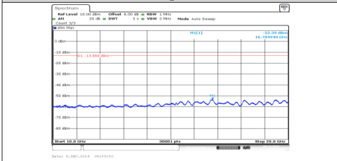
Band II-9262-HSUPA_Sub3-10000~20000
