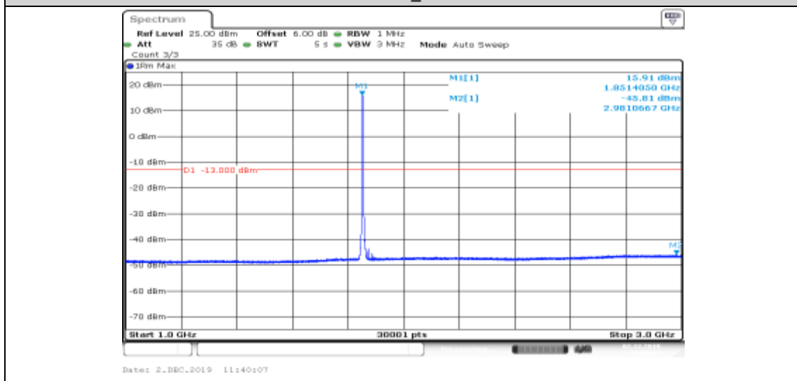
Band II-9262-HSDPA_Sub3-1000~3000
