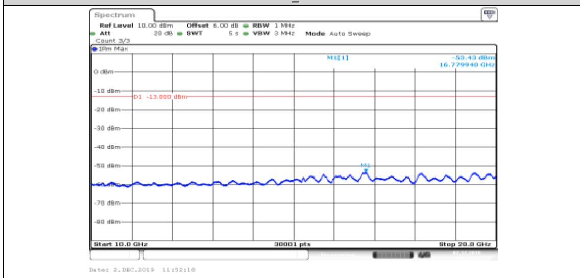
Band II-9400-HSDPA_Sub1-10000~20000
