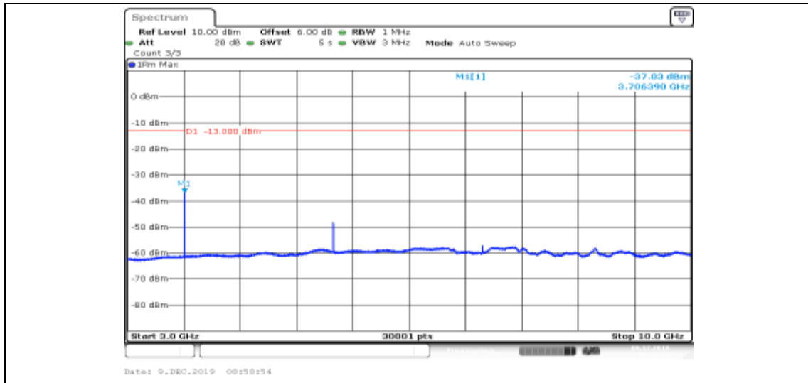
Band II-9262-HSUPA_Sub2-3000~10000
