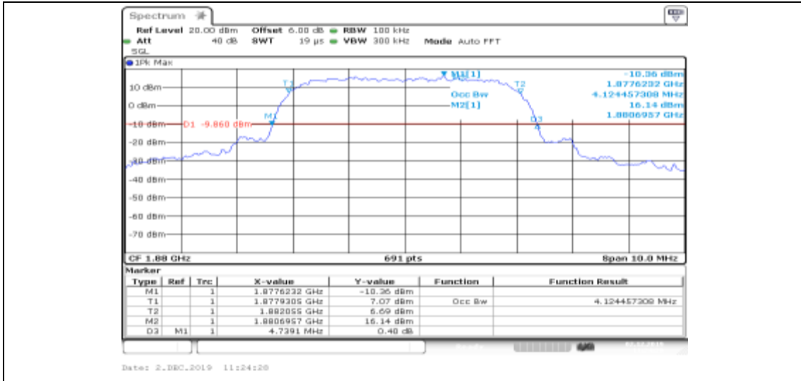
Band II-9538-HSDPA_Sub1
