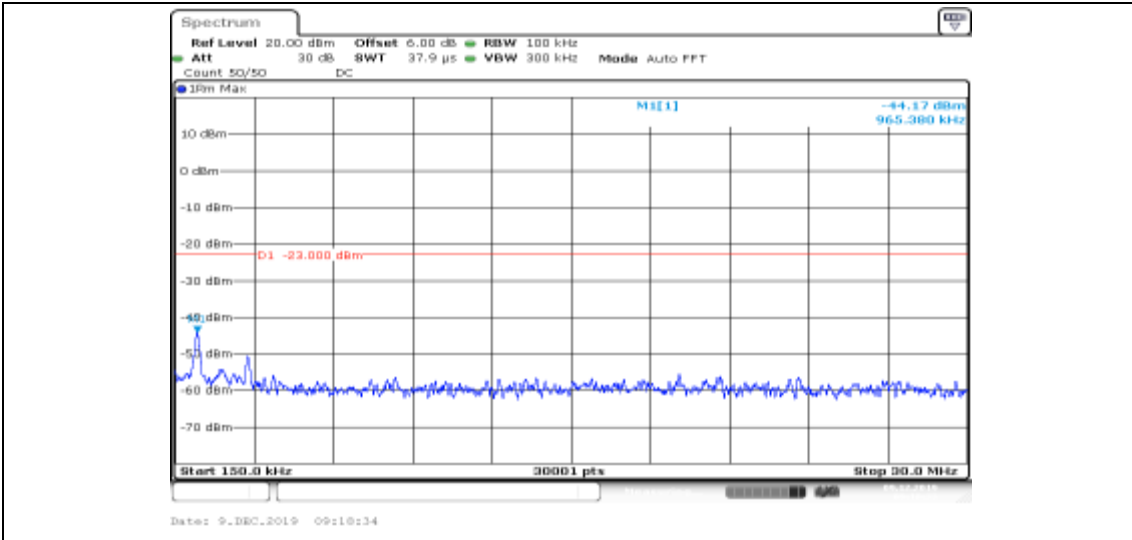
Band II-9400-HSUPA_Sub2-0.15~30
