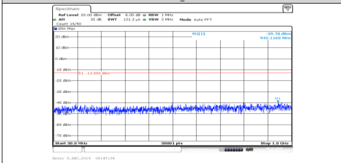
Band II-9262-HSUPA_Sub3-30~1000
