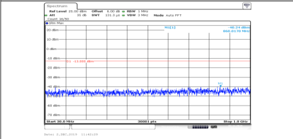
Band II-9262-HSDPA_Sub2-30~1000
