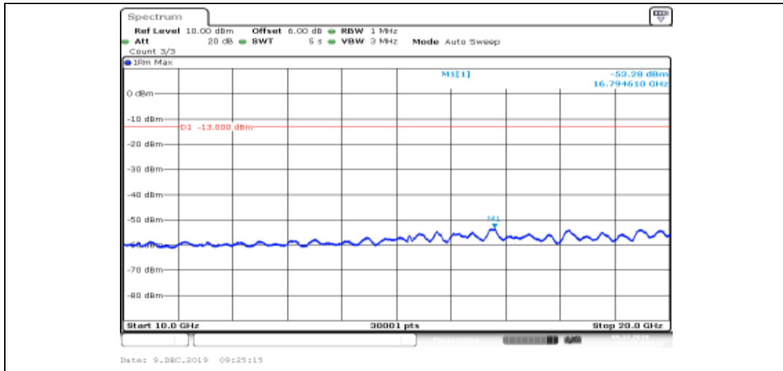
Band II-9538-HSUPA_Sub2-10000~20000
