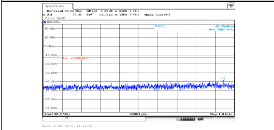
Band II-9400-HSDPA_Sub3-30~1000
