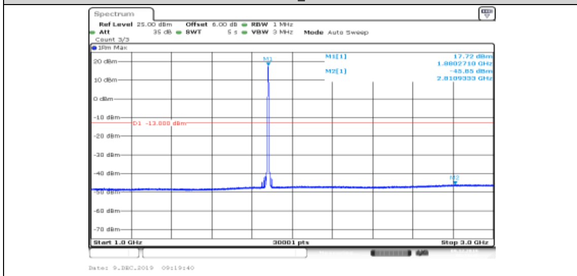
Band II-9400-HSUPA_Sub3-1000~3000
