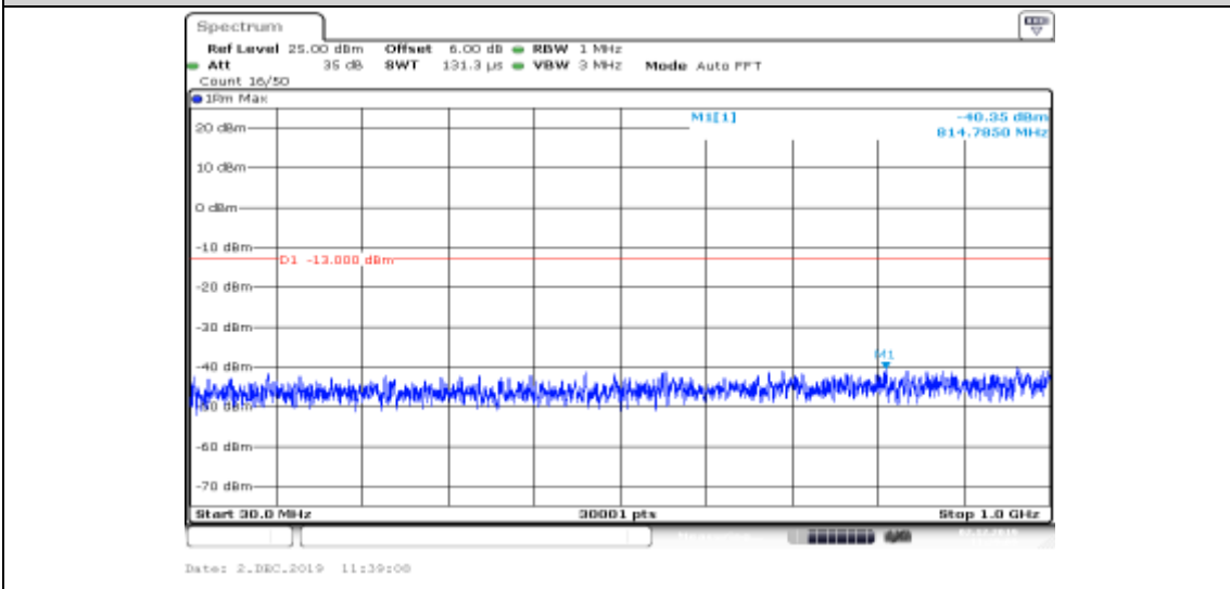
Band II-9262-HSDPA_Sub2-30~1000
