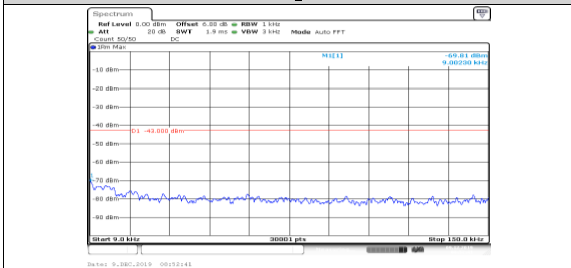
Band II-9262-HSUPA_Sub3-0.009~0.15
