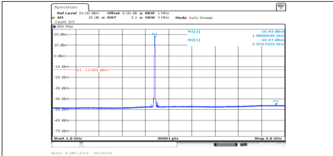
Band II-9400-HSUPA_Sub2-1000~3000
