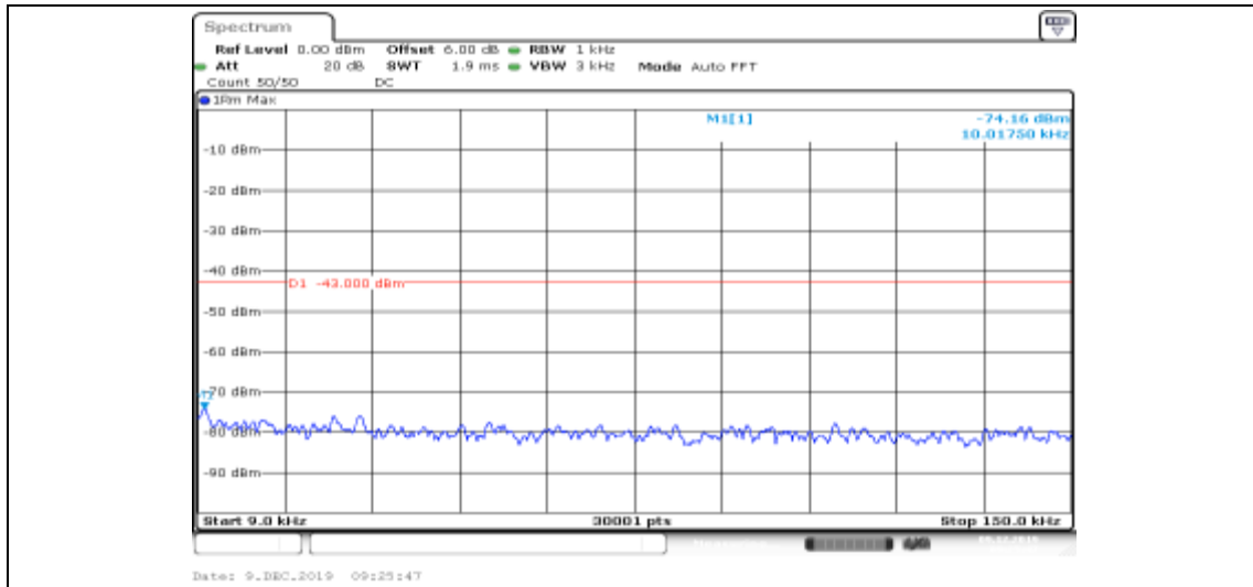
Band II-9538-HSUPA_Sub2-0.009~0.15
