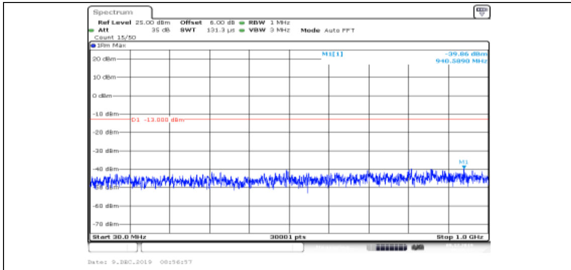
Band II-9262-HSUPA_Sub2-30~1000
