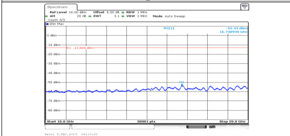
Band II-9400-HSUPA_Sub3-10000~20000
