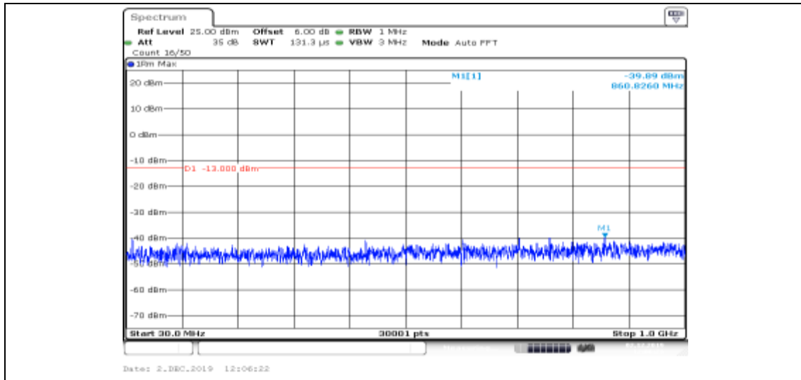
Band II-9538-HSDPA_Sub3-30~1000
