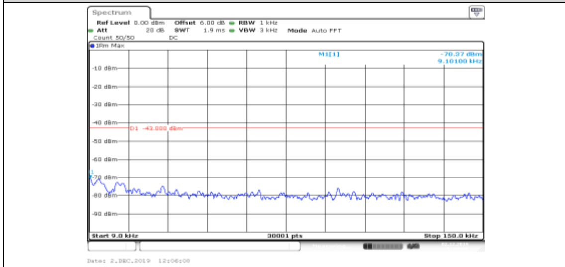
Band II-9538-HSDPA_Sub2-0.009~0.15
