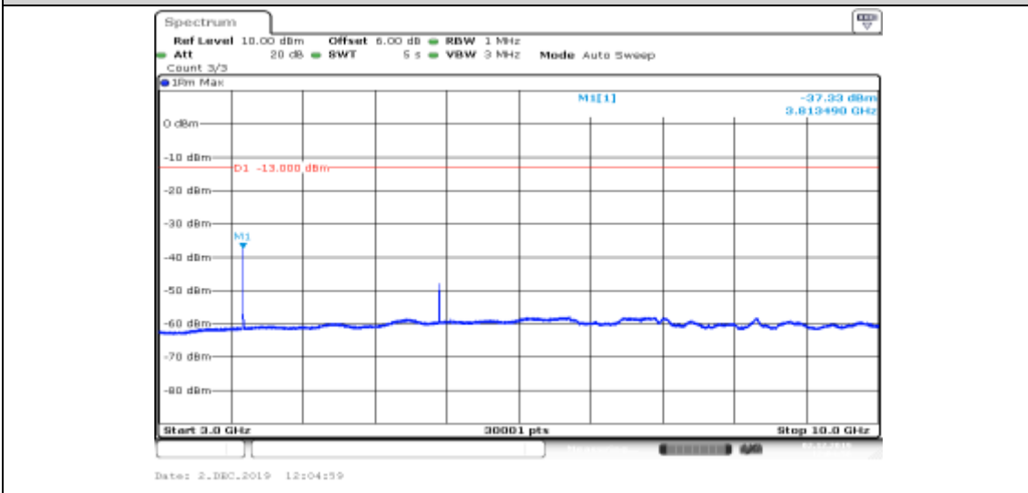
Band II-9538-HSDPA_Sub1-3000~10000
