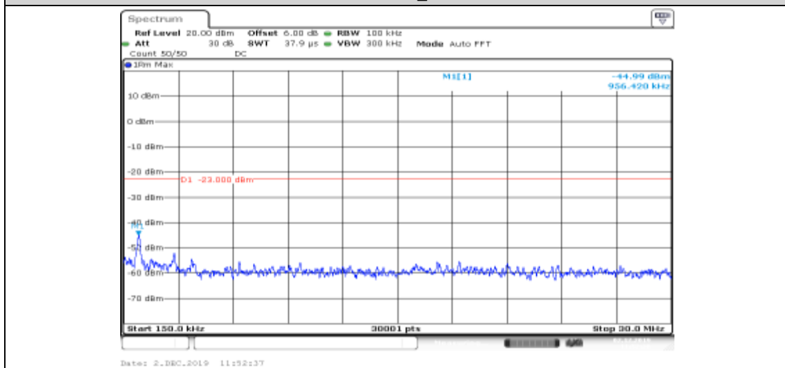
Band II-9400-HSDPA_Sub2-0.15~30
