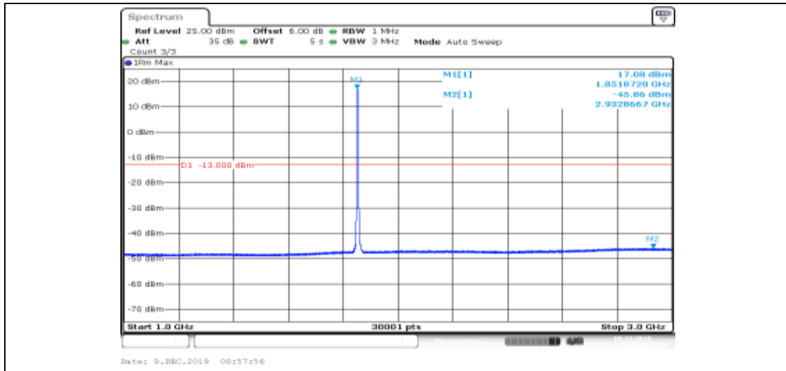
Band II-9262-HSUPA_Sub2-1000~3000
