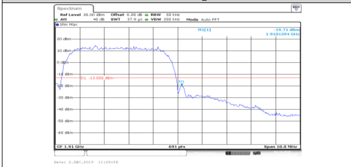
Band II-9538-HSDPA_Sub0
