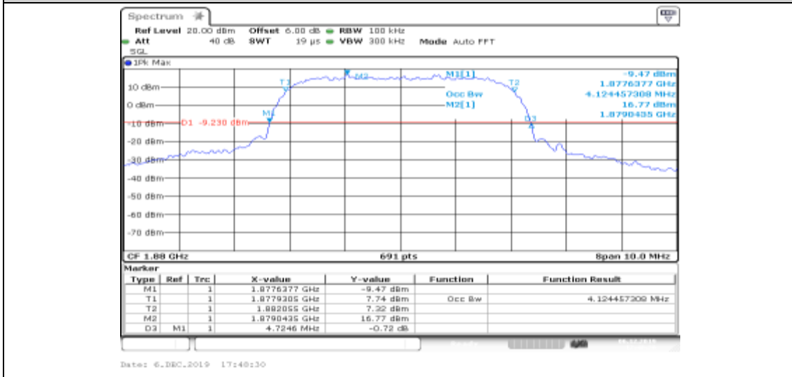
Band II-9400-HSUPA_Sub3
