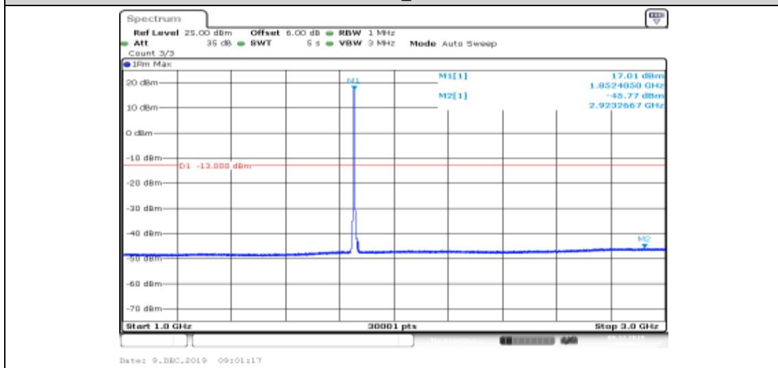
Band II-9262-HSUPA_Sub3-1000~3000
