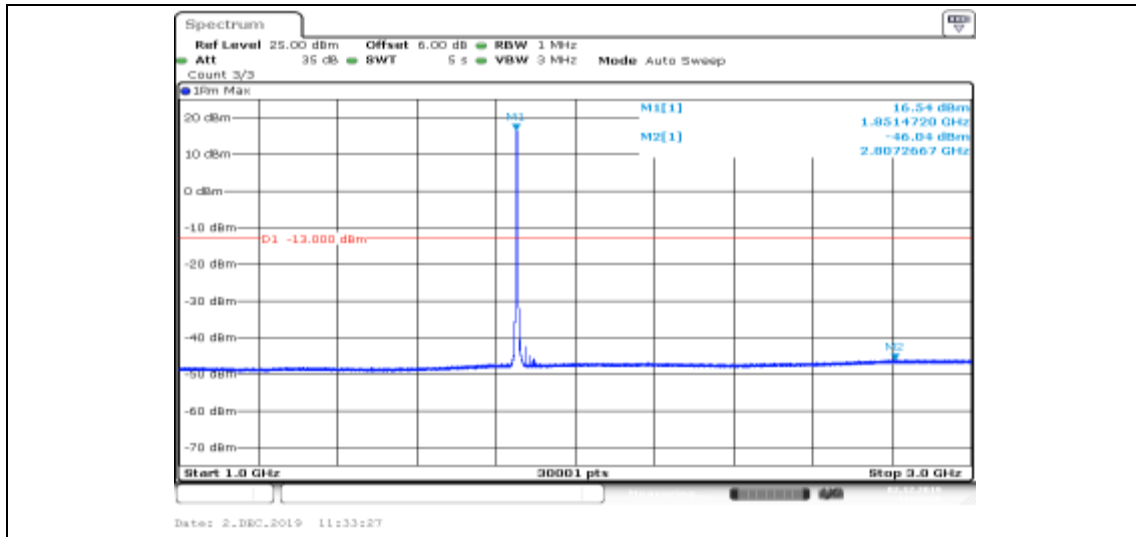
Band II-9262-HSDPA_Sub2-1000~3000
