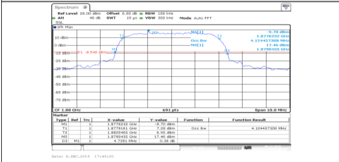
Band II-9400-HSUPA_Sub3
