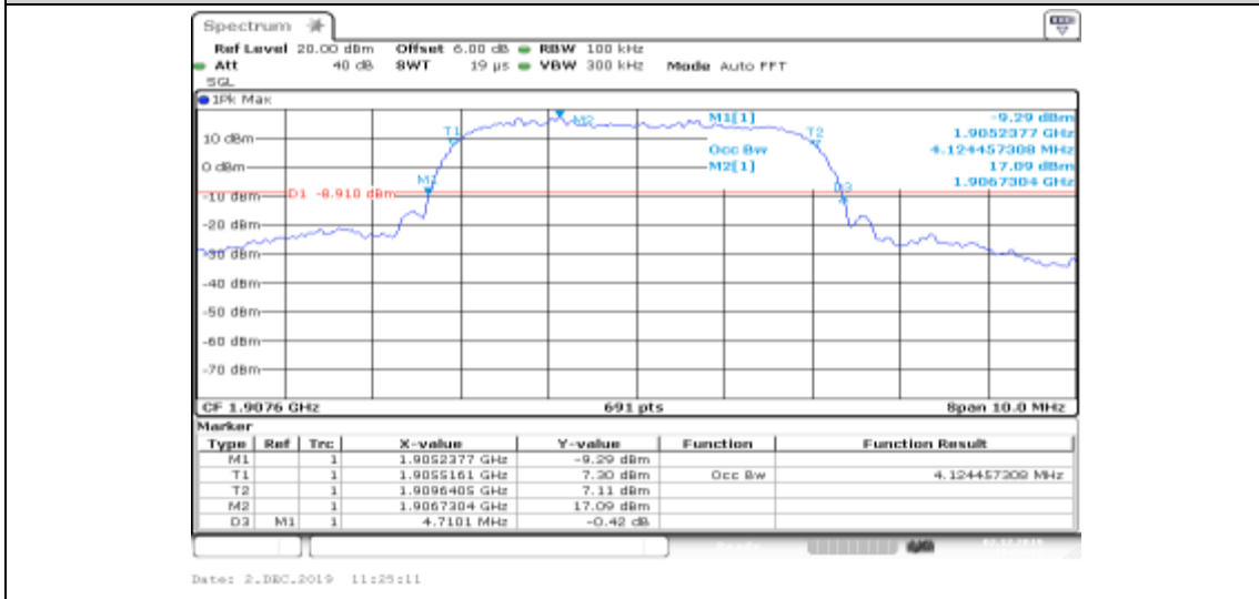
Band II-9538-HSDPA_Sub2
