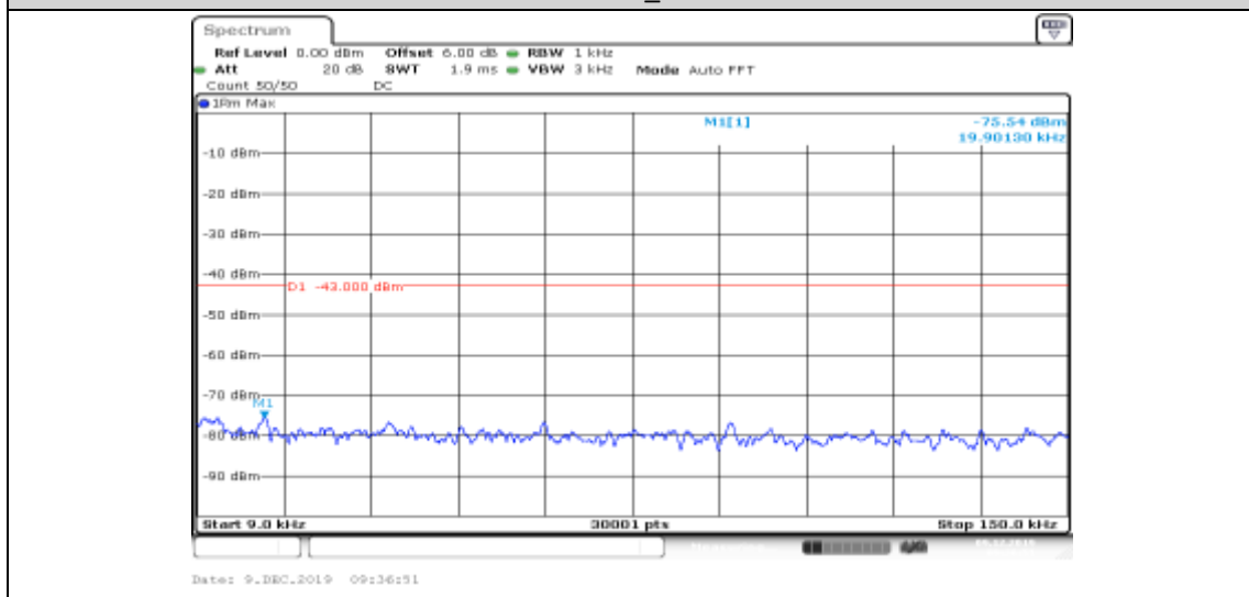
Band II-9538-HSUPA_Sub3-0.009~0.15
