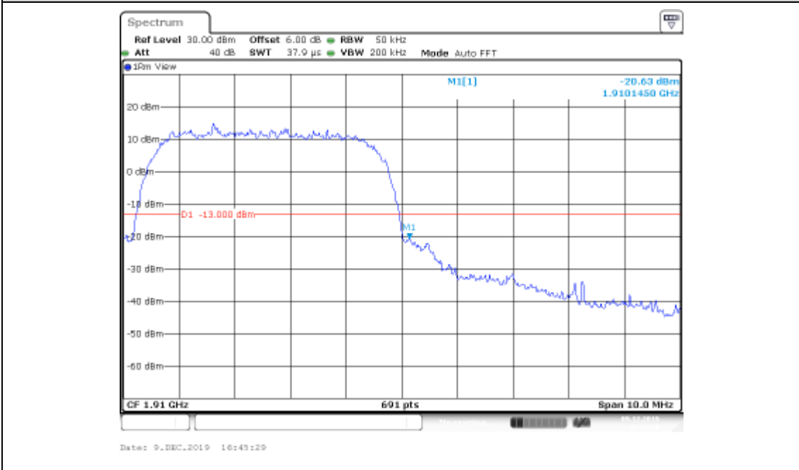
Band II-9538-HSUPA_Sub3
