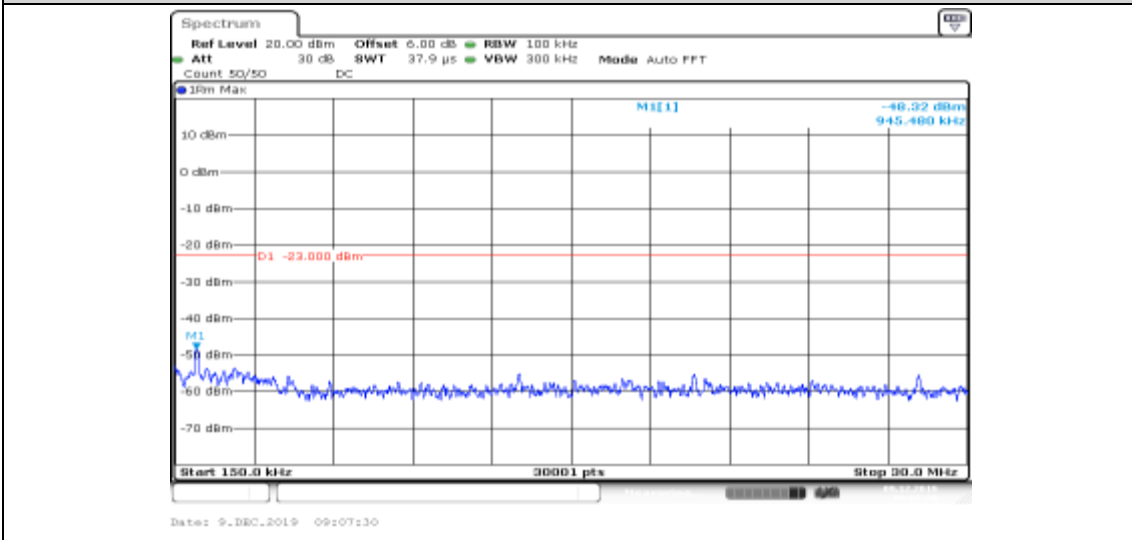
Band II-9400-HSUPA_Sub3-0.15~30
