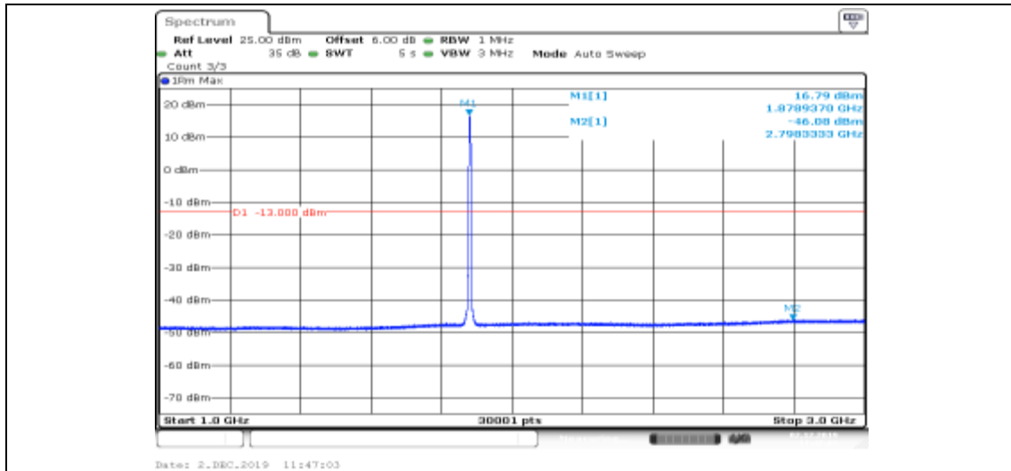
Band II-9400-HSDPA_Sub3-1000~3000
