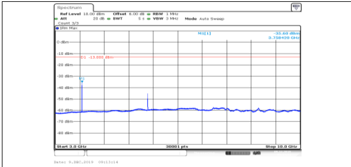
Band II-9400-HSUPA_Sub2-3000~10000
