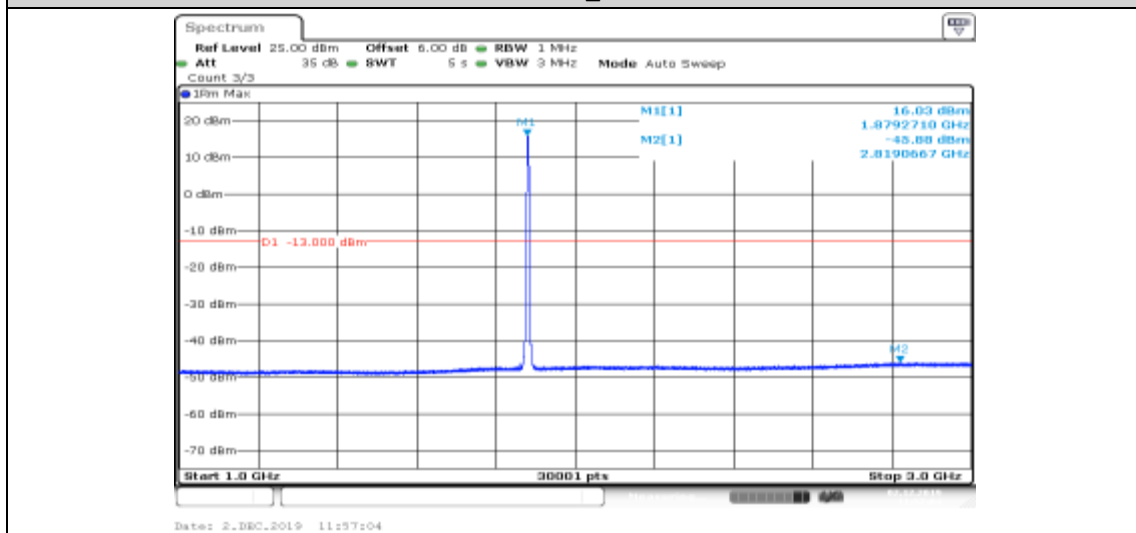
Band II-9400-HSDPA_Sub4-1000~3000
