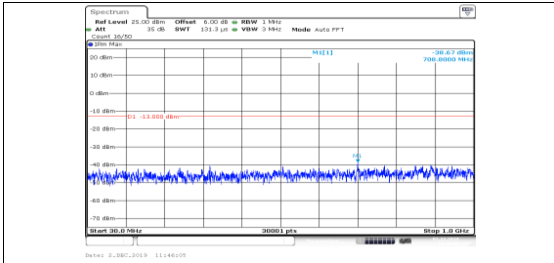
Band II-9400-HSDPA_Sub2-30~1000
