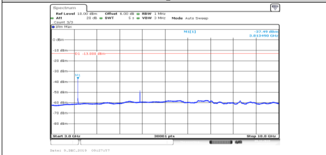
Band II-9538-HSUPA_Sub3-3000~10000
