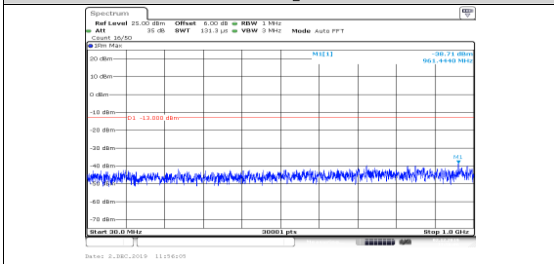
Band II-9400-HSDPA_Sub3-30~1000
