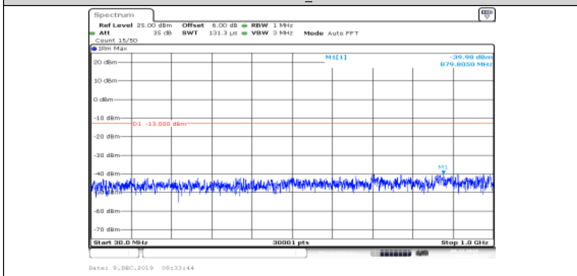
Band II-9538-HSUPA_Sub3-30~1000
