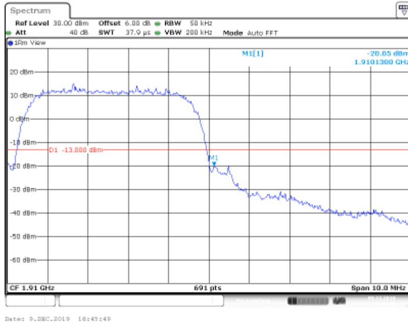
Band II-9538-HSUPA_Sub4
