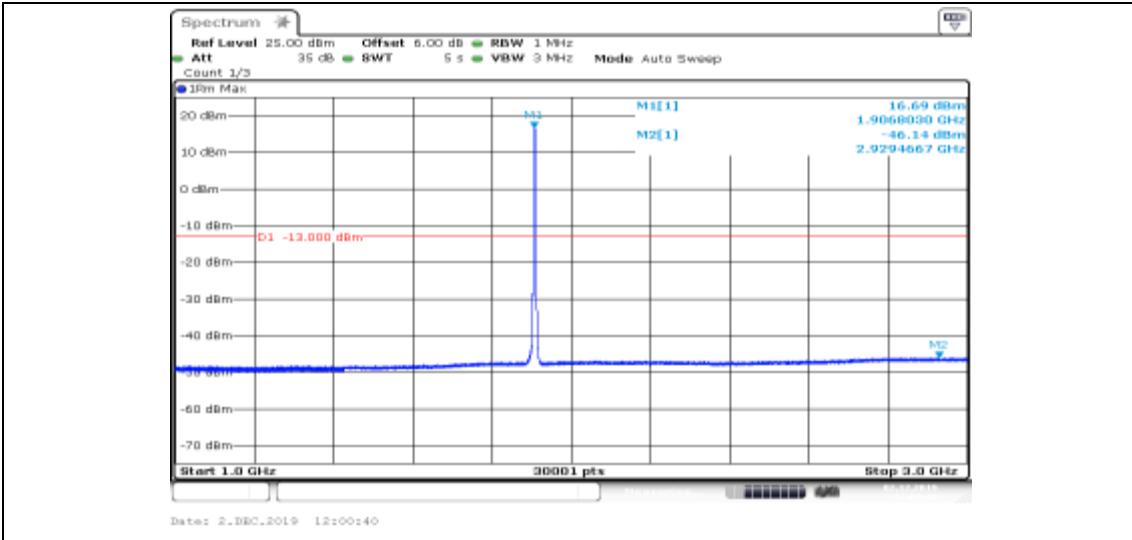
Band II-9538-HSDPA_Sub4-1000~3000
