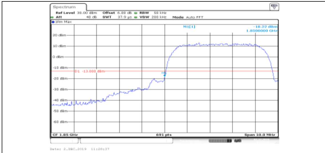
Band II-9262-HSDPA_Sub3
