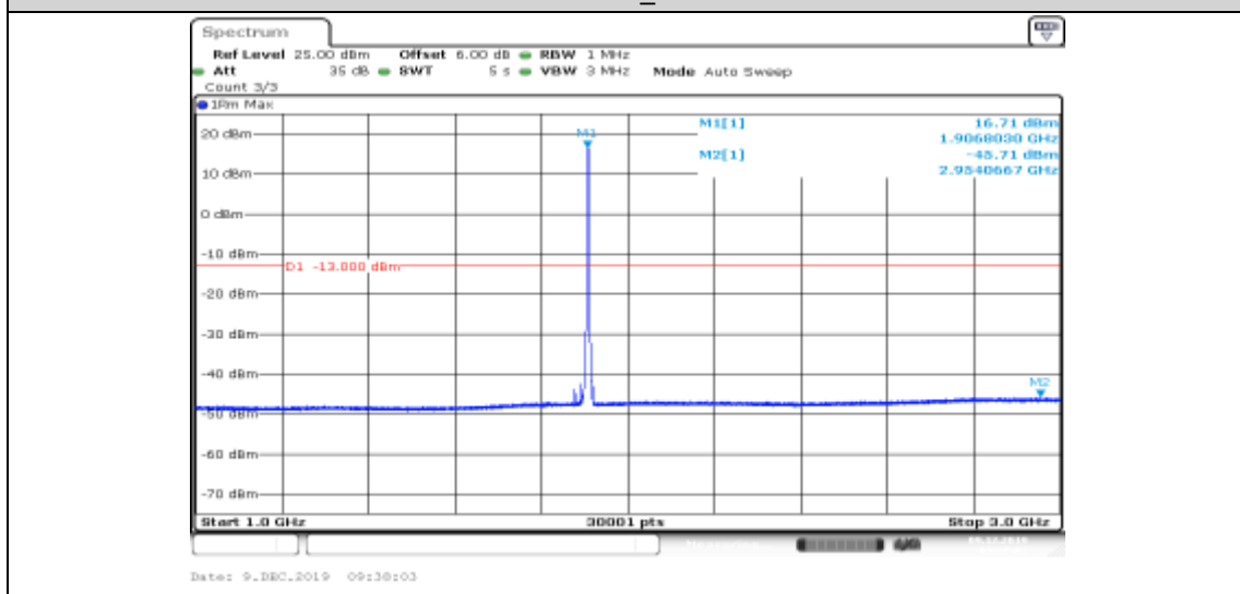
Band II-9538-HSUPA_Sub3-1000~3000
