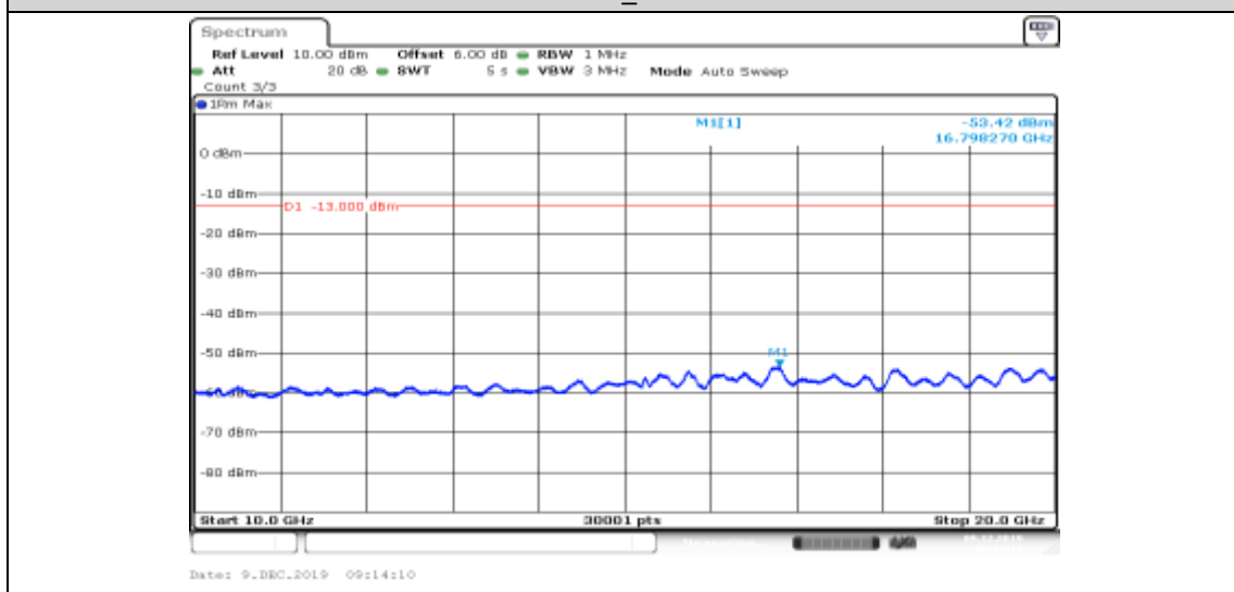
Band II-9400-HSUPA_Sub3-10000~20000
