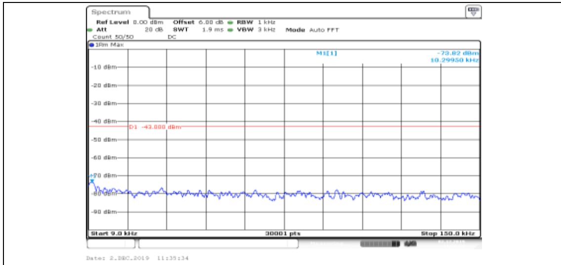
Band II-9262-HSDPA_Sub4-0.009~0.15
