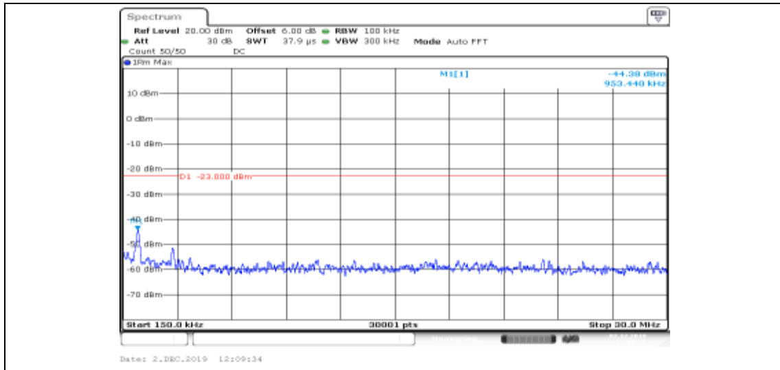
Band II-9538-HSDPA_Sub2-0.15~30
