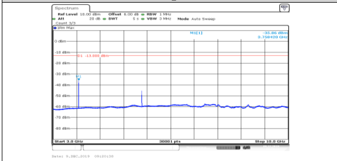
Band II-9400-HSUPA_Sub3-3000~10000
