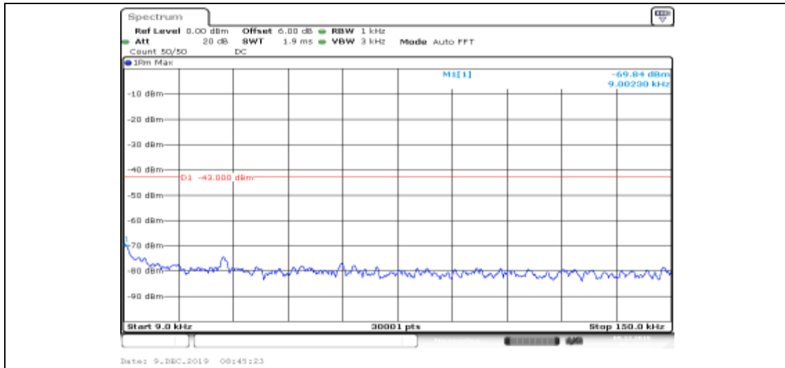
Band II-9262-HSUPA_Sub2-0.009~0.15
