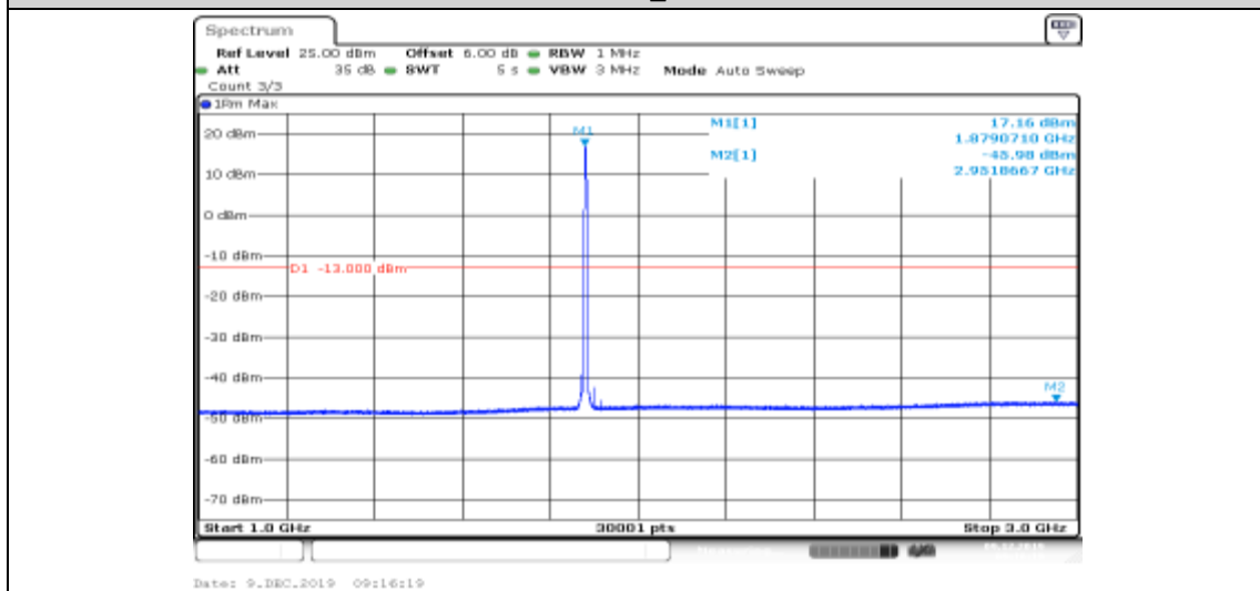
Band II-9400-HSUPA_Sub3-1000~3000
