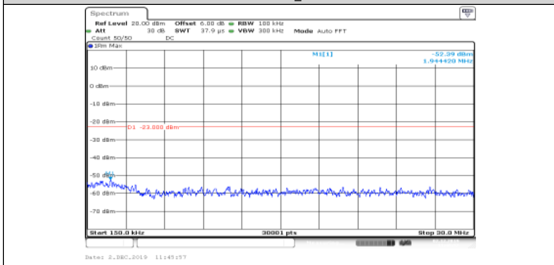
Band II-9400-HSDPA_Sub2-0.15~30
