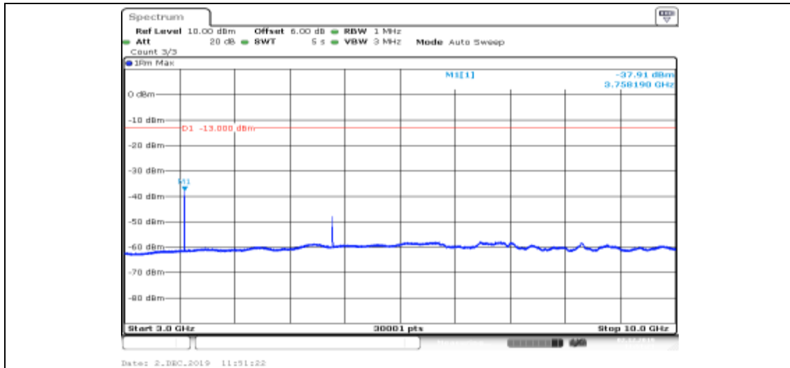
Band II-9400-HSDPA_Sub4-3000~10000
