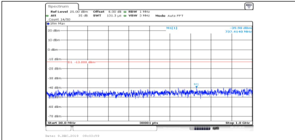
Band II-9400-HSUPA_Sub2-30~1000
