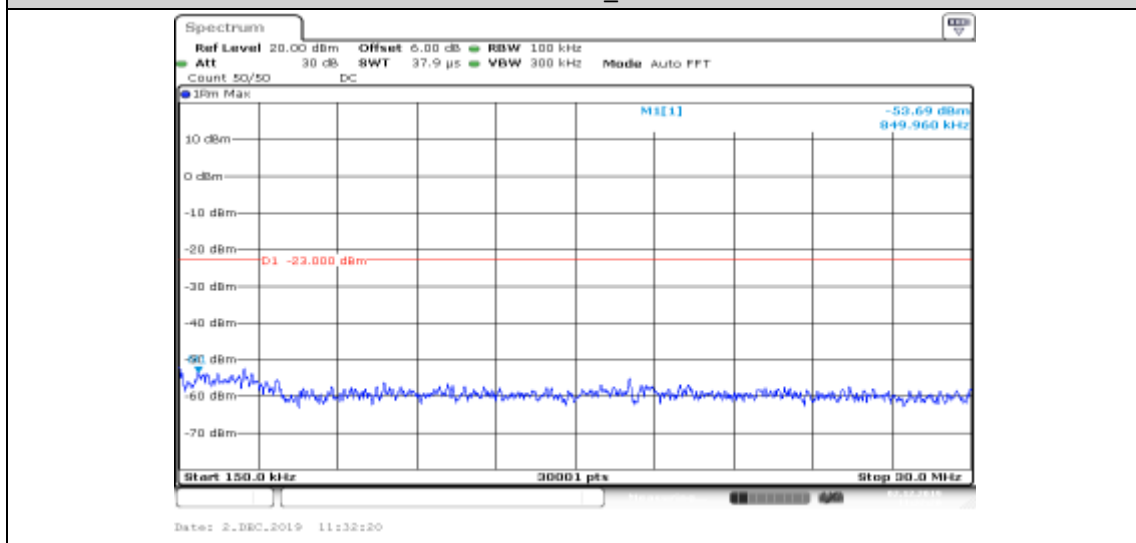
Band II-9262-HSDPA_Sub1-0.15~30
