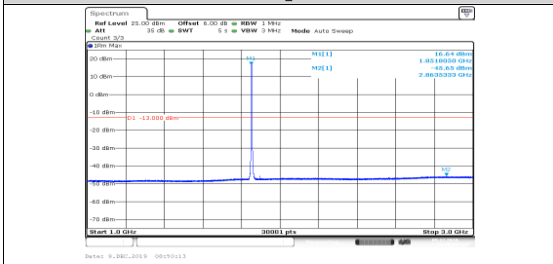
Band II-9262-HSUPA_Sub3-1000~3000
