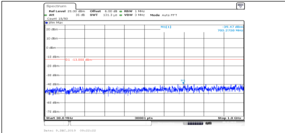
Band II-9538-HSUPA_Sub2-30~1000
