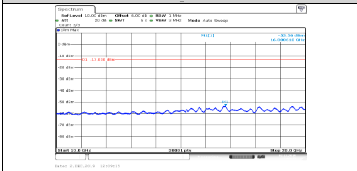
Band II-9538-HSDPA_Sub2-10000~20000
