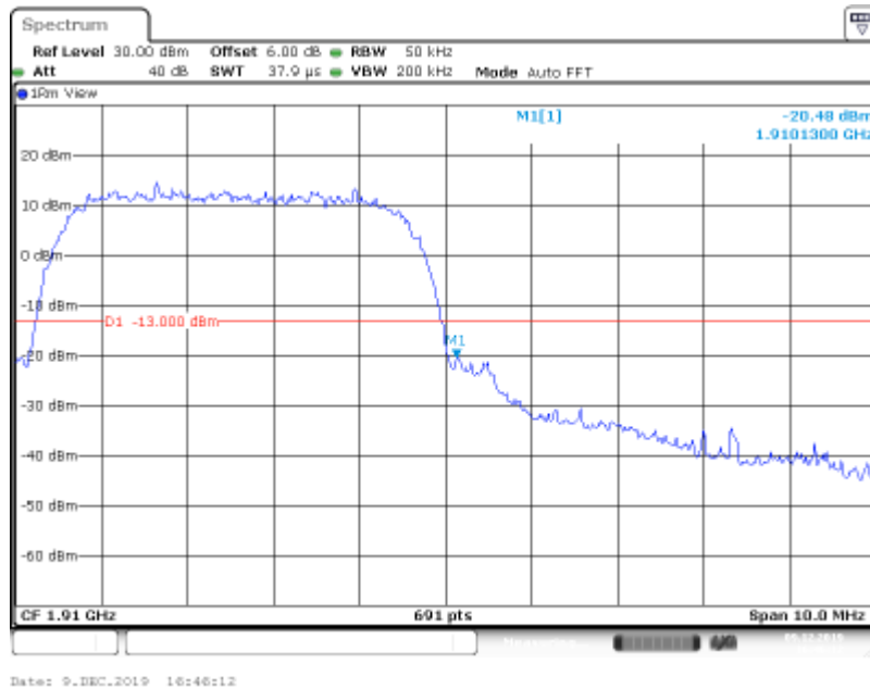
Band II-9538-HSUPA_Sub5
