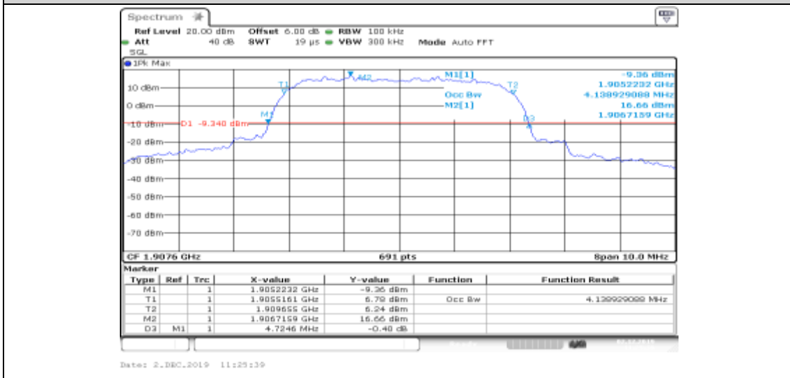
Band II-9538-HSDPA_Sub2
