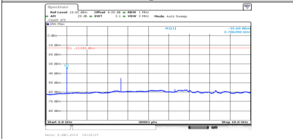
Band II-9262-HSUPA_Sub3-3000~10000
