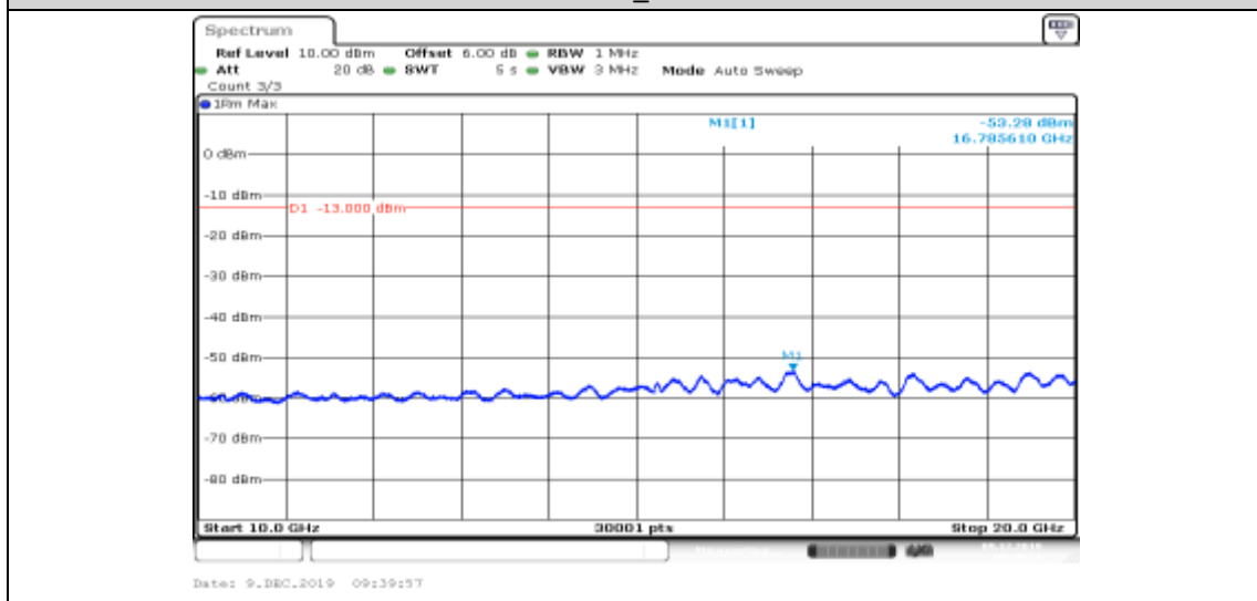
Band II-9538-HSUPA_Sub3-10000~20000
