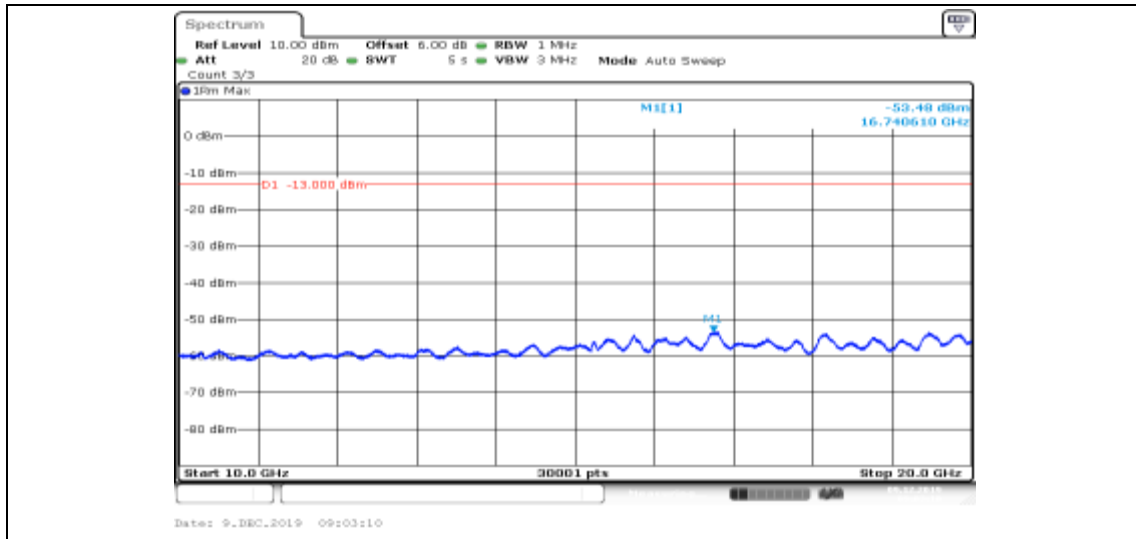
Band II-9262-HSUPA_Sub2-10000~20000
