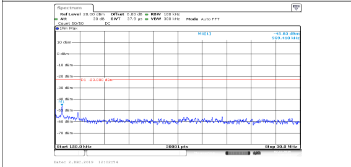
Band II-9538-HSDPA_Sub3-0.15~30
