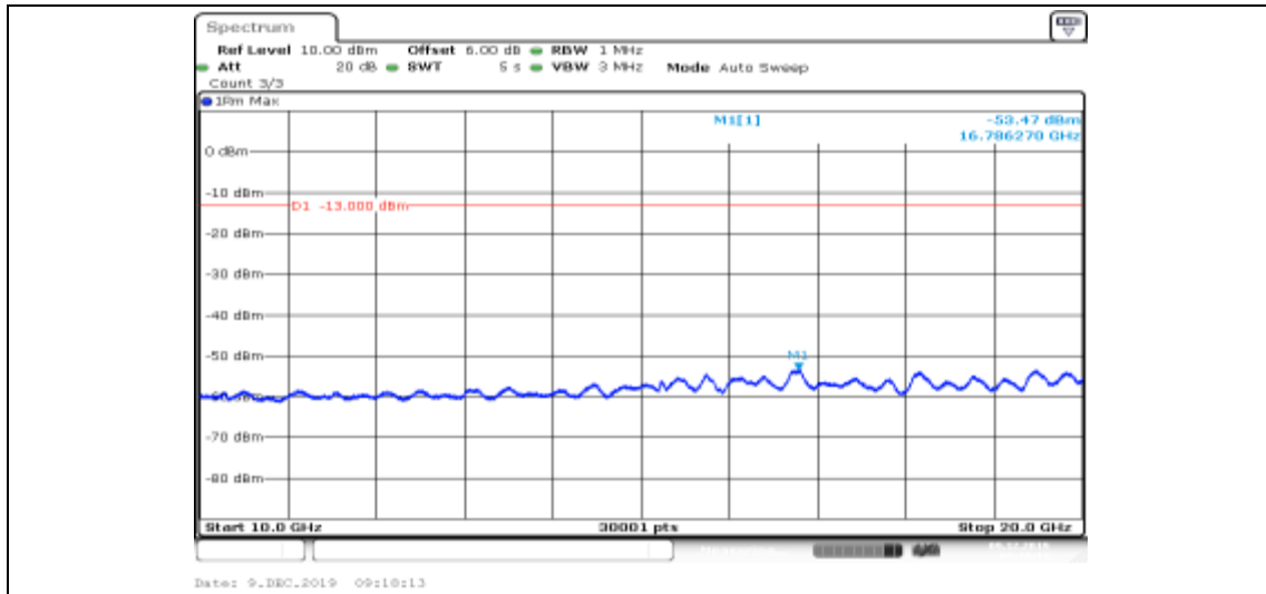
Band II-9400-HSUPA_Sub2-10000~20000
