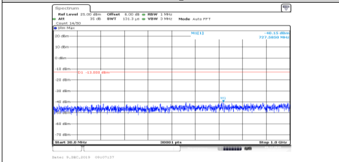
Band II-9400-HSUPA_Sub3-30~1000
