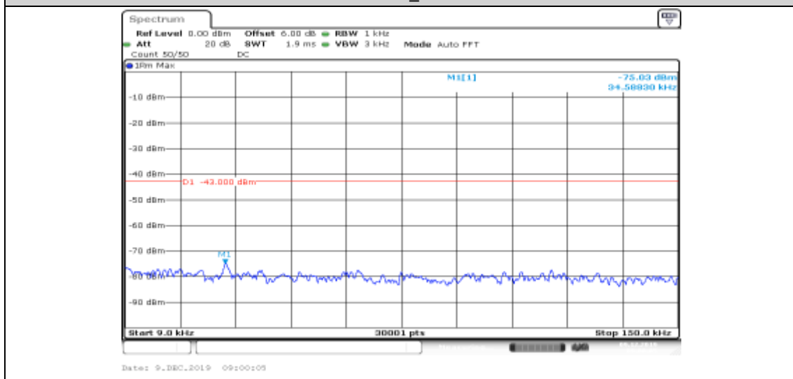
Band II-9262-HSUPA_Sub3-0.009~0.15
