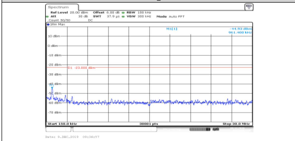
Band II-9538-HSUPA_Sub3-0.15~30
