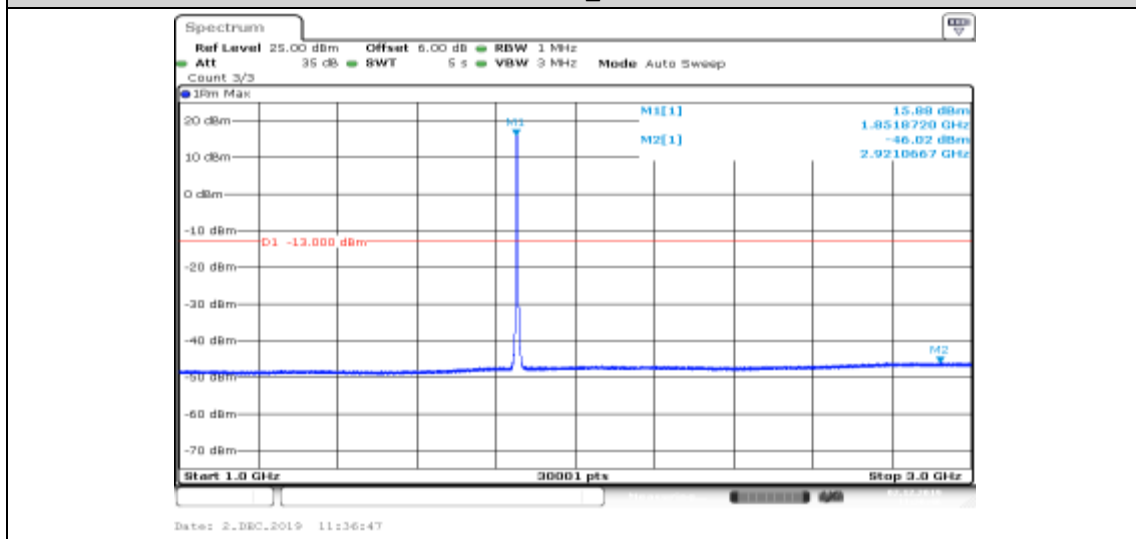
Band II-9262-HSDPA_Sub3-1000~3000
