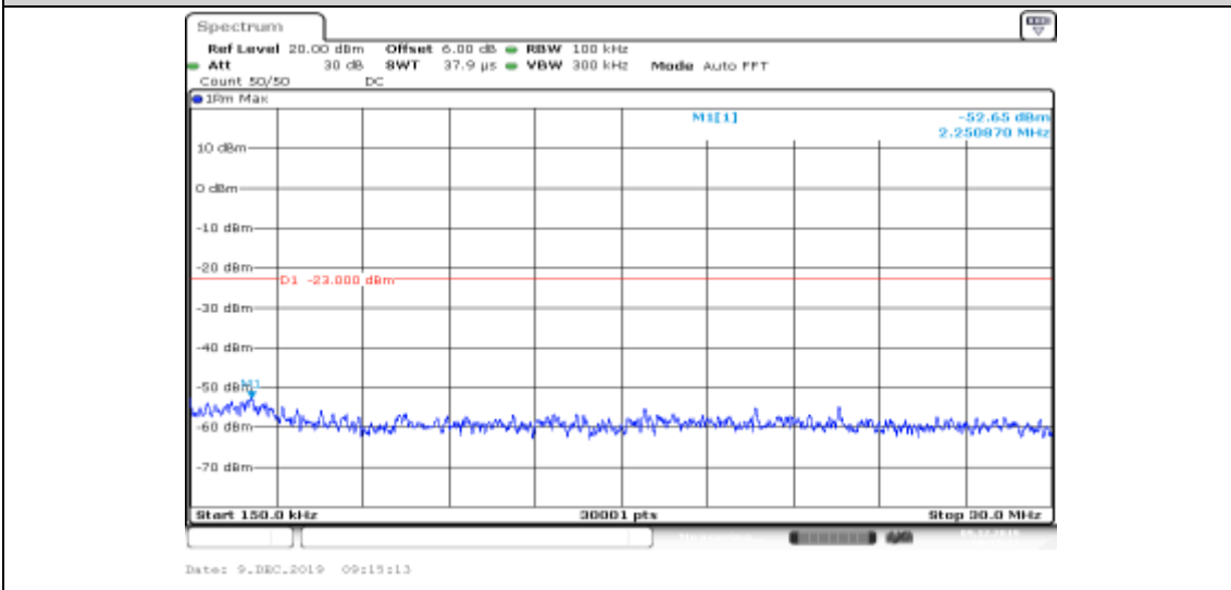
Band II-9400-HSUPA_Sub3-0.15~30
