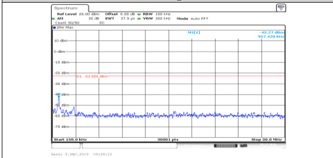
Band II-9538-HSUPA_Sub3-0.15~30
