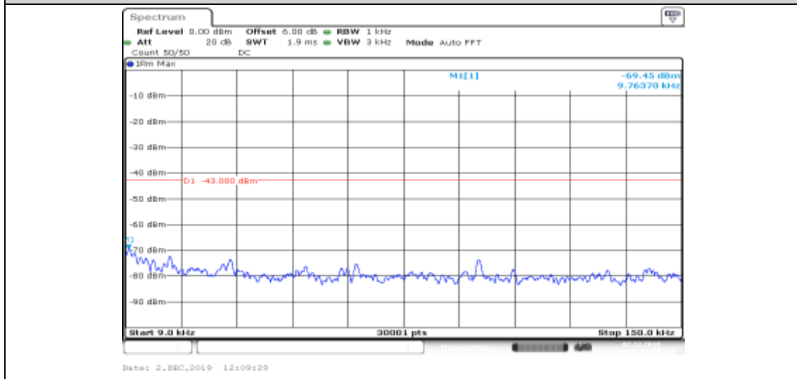
Band II-9538-HSDPA_Sub2-0.009~0.15
