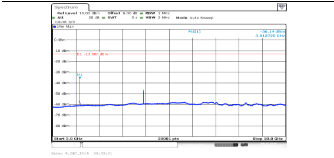
Band II-9538-HSUPA_Sub2-3000~10000
