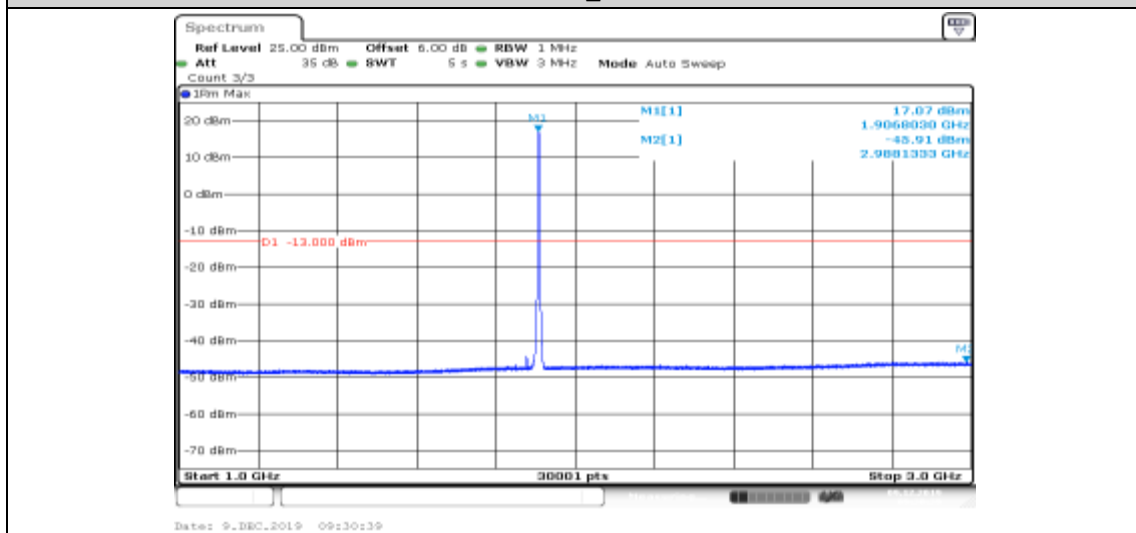
Band II-9538-HSUPA_Sub3-1000~3000
