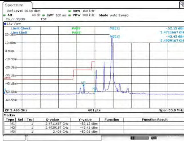
Band41-5MHz-QPSK-39675-1RB#24
