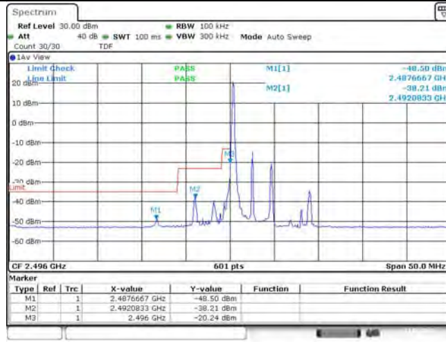
Band41-5MHz-QPSK-39675-1RB#0
