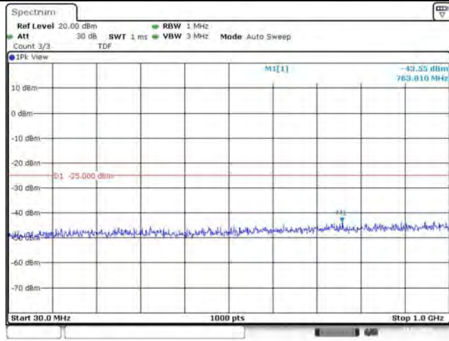
Band41-5MHz-QPSK-39675-1RB#0-Range1:30~1000MHz
