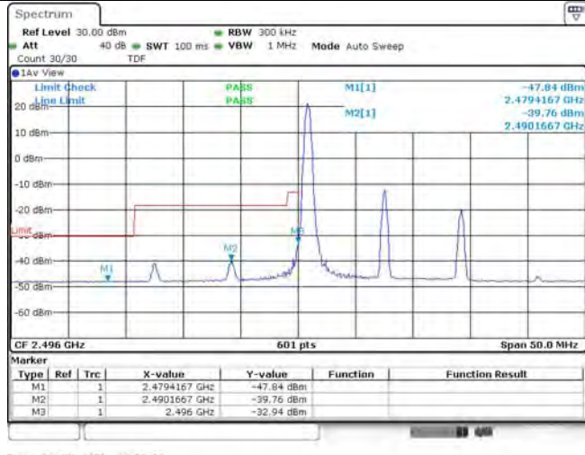
Band41-15MHz-16QAM-39725-1RB#74
