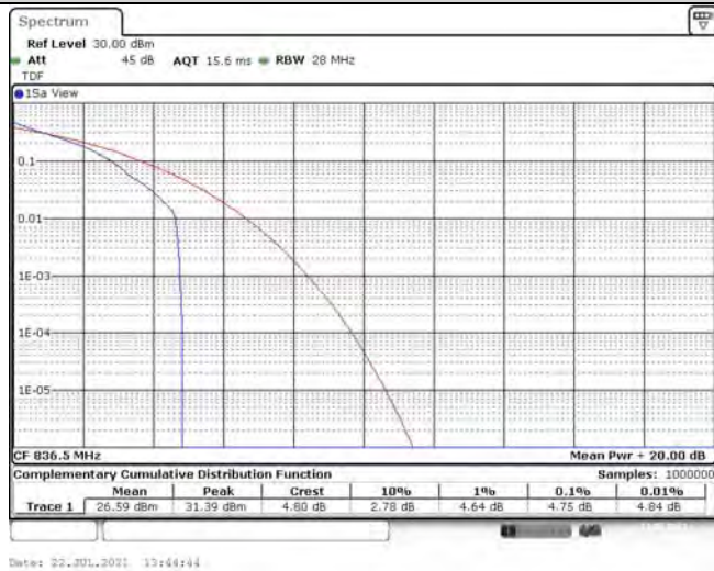
Band26-5MHz-QPSK-26915-25RB#0
