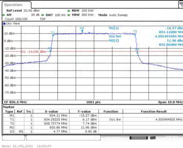
Band26-5MHz-16QAM-27015-25RB#0-4.505
