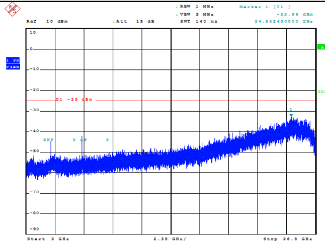
Band7-5MHz-QPSK-20775-1RB#0-Range3:3000~26500MHz
