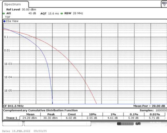
Band26-15MHz-16QAM-26865-1RB#0
