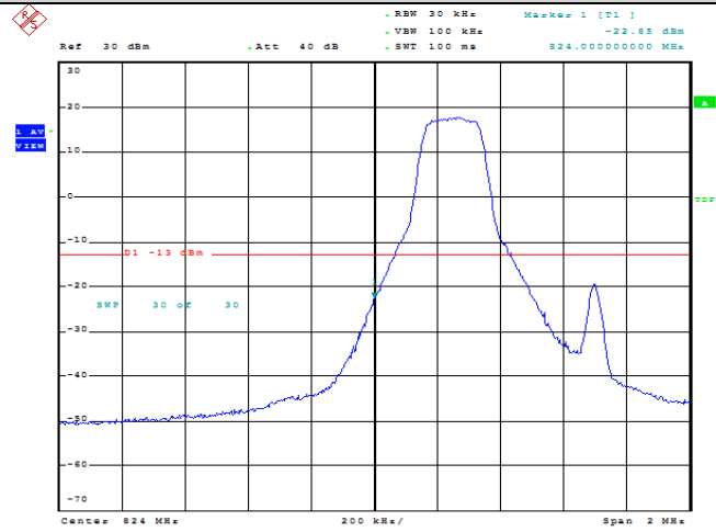
Band26-1.4MHz-QPSK-26797-1RB#0
