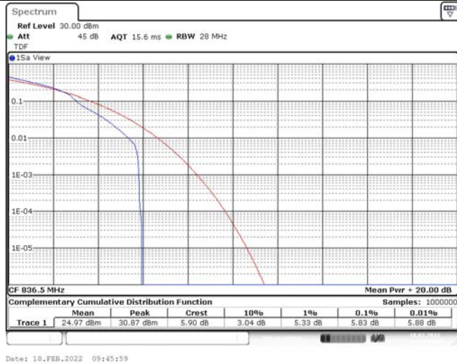
Band26-10MHz-16QAM-26915-50RB#0
