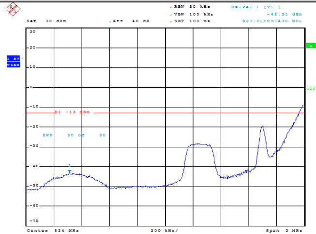
Band26-1.4MHz-QPSK-26797-1RB#5
