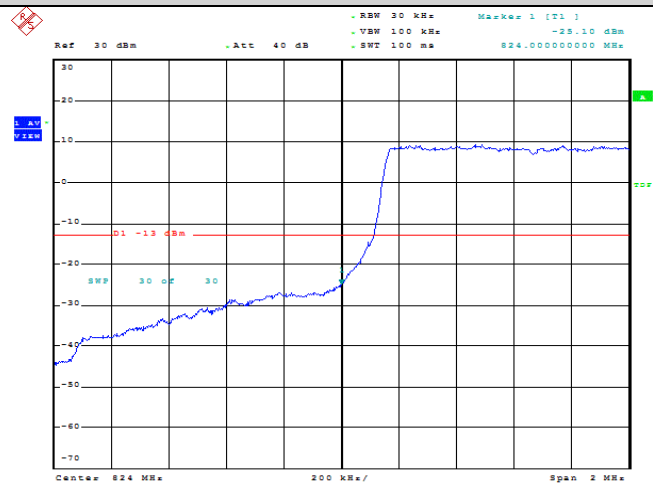
Band26-1.4MHz-QPSK-26797-6RB#0
