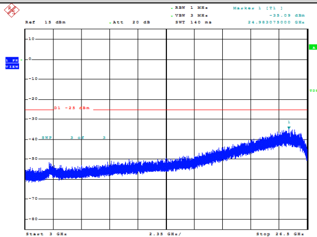
Band7-5MHz-QPSK-20775-1RB#0-Range3:3000~26500MHz
