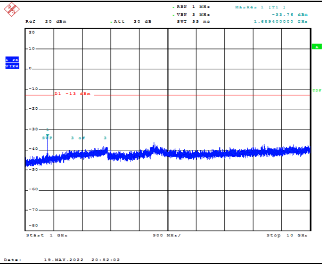
Band5-5MHz-16QAM-20625-1RB#0-Range2:1000~10000MHz
