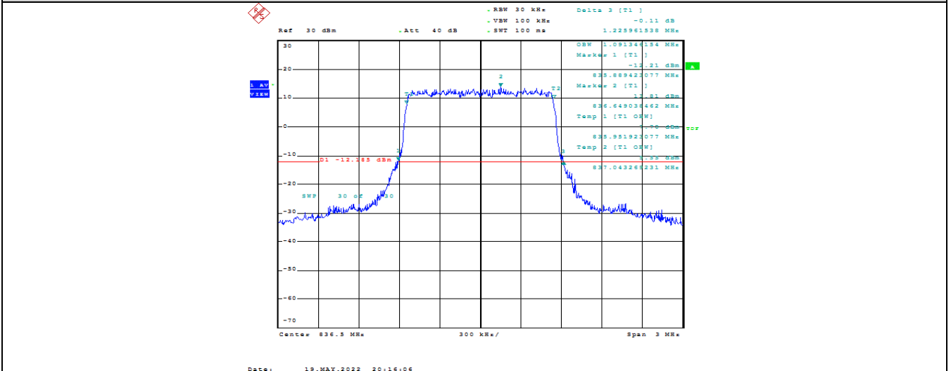
Band5-1.4MHz-QPSK-20525-6RB#0-1.091
