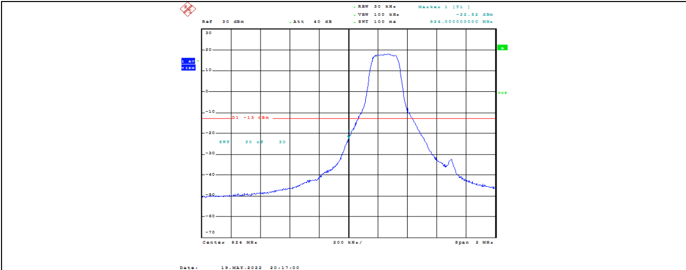
Band5-1.4MHz-QPSK-20407-1RB#0
