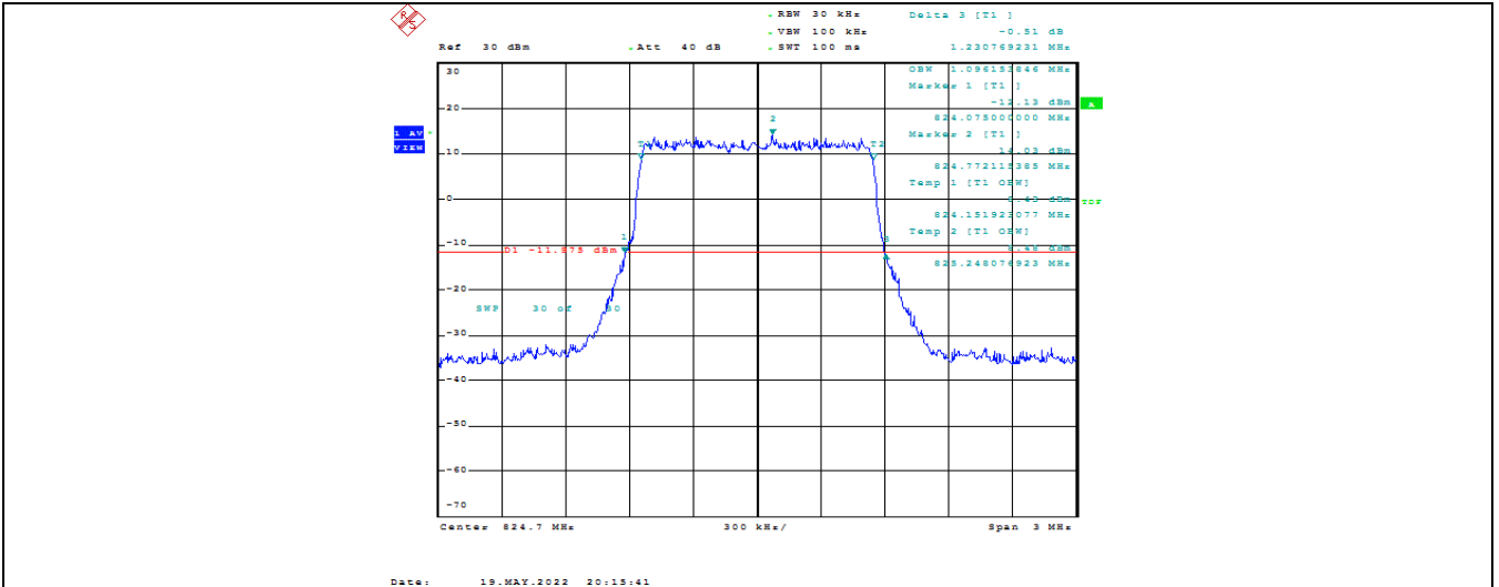
Band5-1.4MHz-QPSK-20407-6RB#0-1.096
