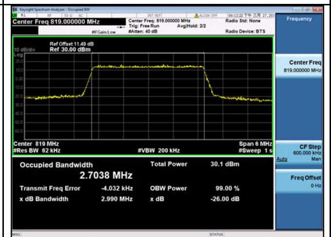
LTE band 26 - Low CH 16QAM-3
