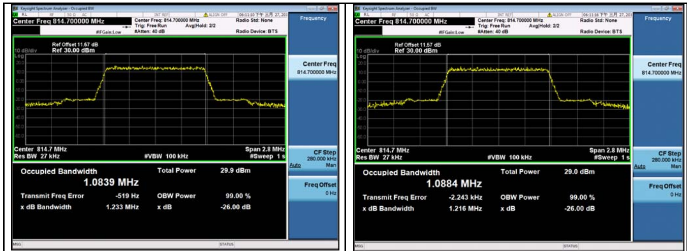
LTE band 26 - Low CH QPSK-1.4
