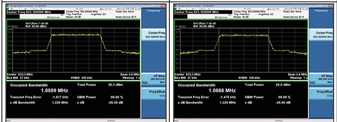
LTE band 26 - Middle CH QPSK-1.4
