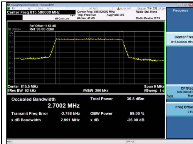
LTE band 26 - Low CH QPSK-3
