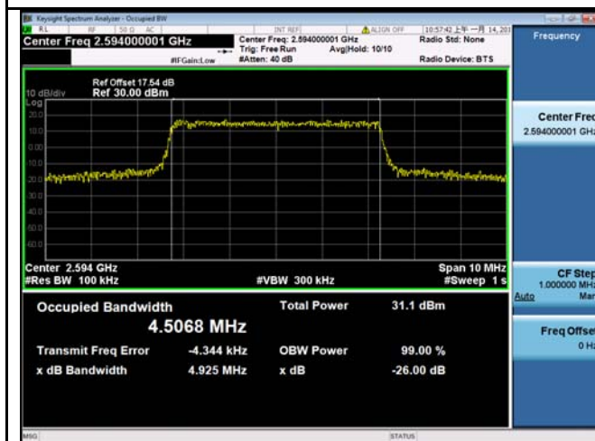
LTE band 41 - Middle CH QPSK-5
