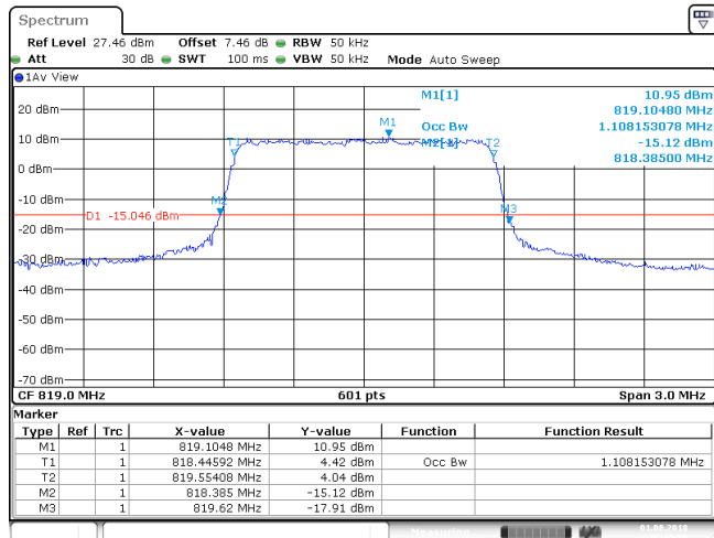
Band26_1.4MHz_QPSK_26740_6RB#0
