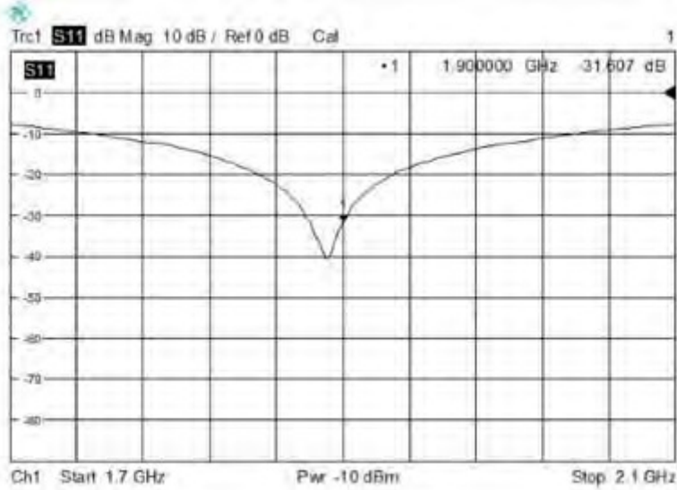
Return loss
