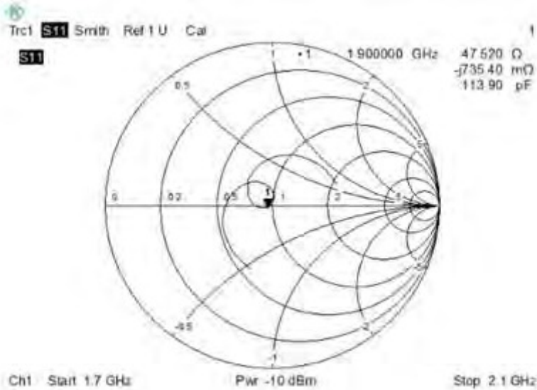
Impedance
