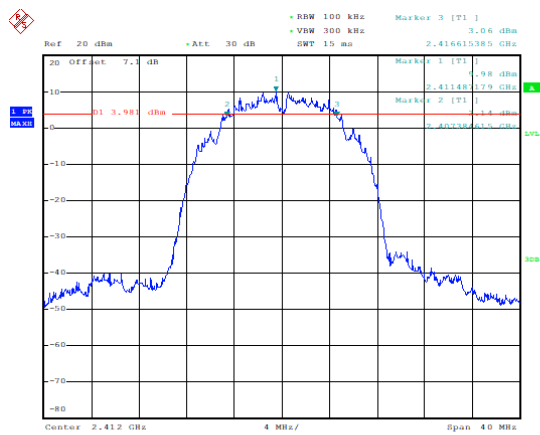
Occupied 6dB Bandwidth (MHz) (802.11b, Ch1)
