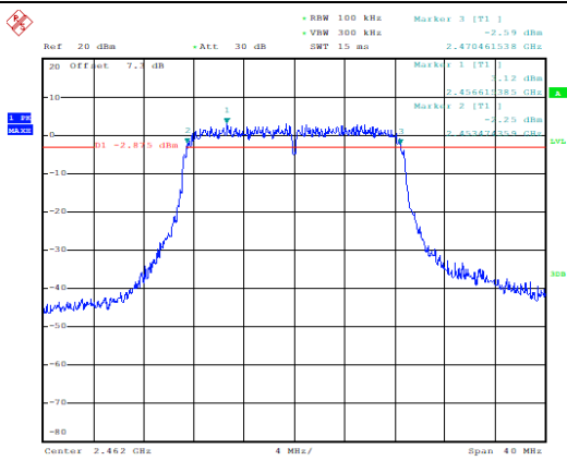
Occupied 6dB Bandwidth (MHz) (802.11n-20MHz, Ch11)
