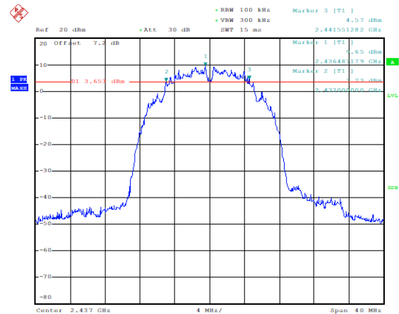
Occupied 6dB Bandwidth (MHz) (802.11b, Ch6)
