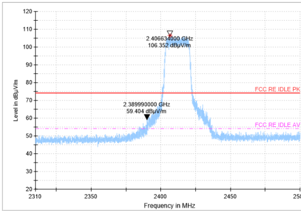
Peak detector
