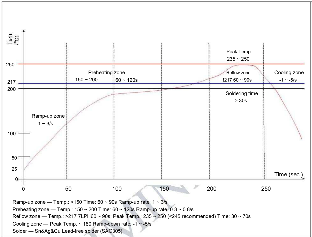
Figure 2: Reflow Profile
