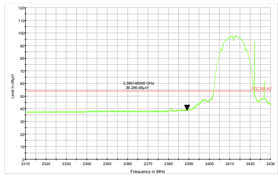
802.11b-Channel 1 Average
