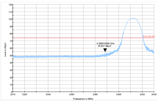
802.11b-Channel 1 Peak
