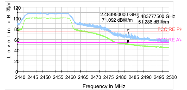
802.11n HT20 -Channel 9 Peak + Average
