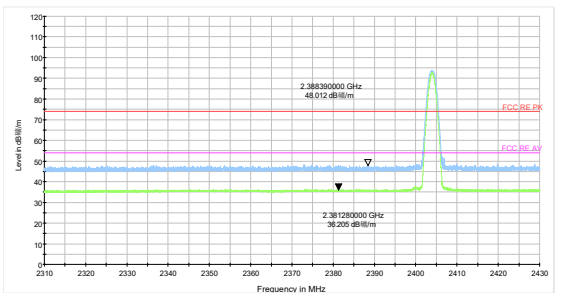
Bluetooth LE Channel 0 Peak + Average
