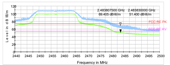
802.11g-Channel 10 Peak + Average
