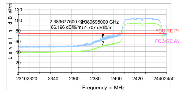
802.11n HT40 -Channel 4 Peak + Average
