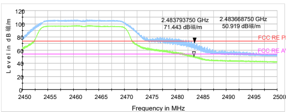
802.11g-Channel 11 Peak + Average
