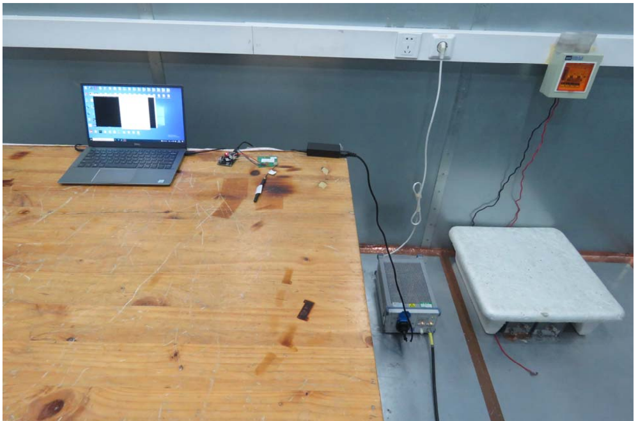
Picture 2 Conducted Emission Test Setup
