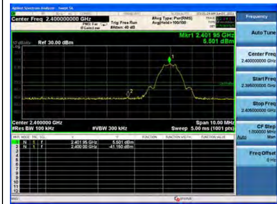
Bluetooth LE (2M), Channel No.: 0
