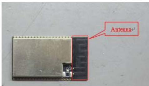
ESP32-WROVER-E
