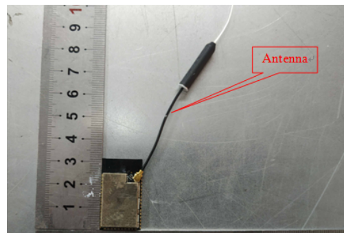
ESP32-S2-WROOM-I
