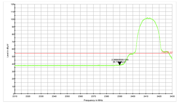
802.11b-Channel 1 Average
