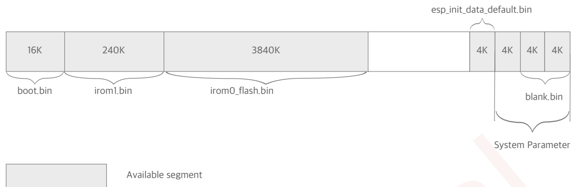
Figure 2-3. Flash Layout
