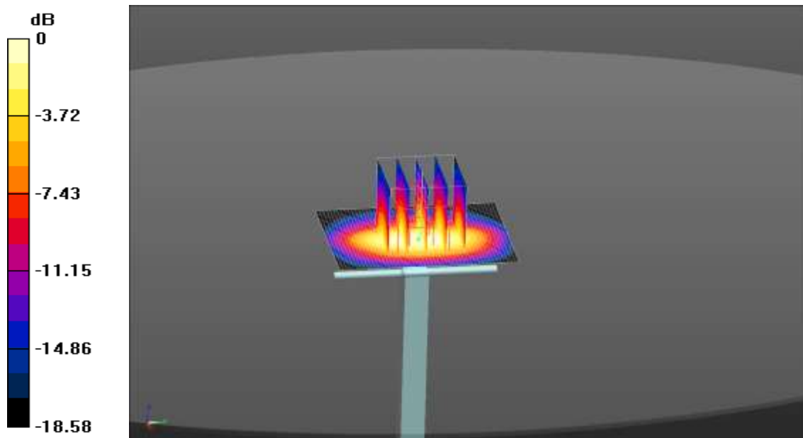
0 dB = 2.26 W/kg = 3.54 dBW/kg
