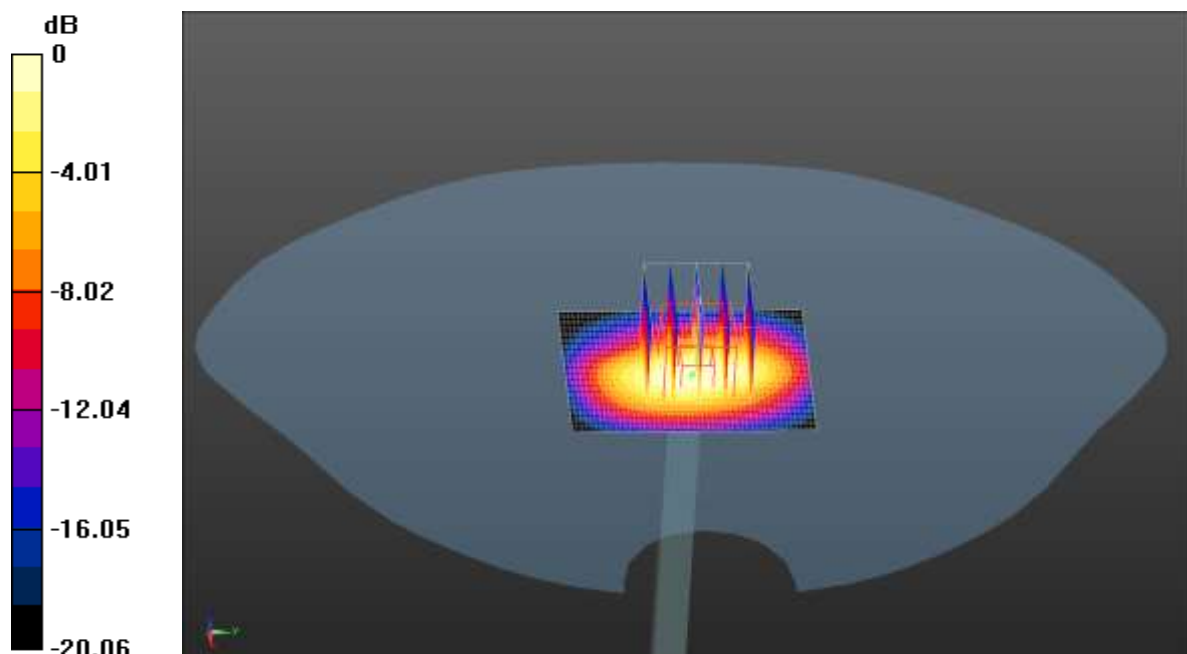
0 dB = 2.42 W/kg = 3.84 dBW/kg
