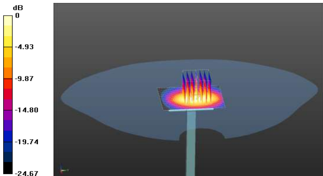
0 dB = 3.25 W/kg = 5.12 dBW/kg
