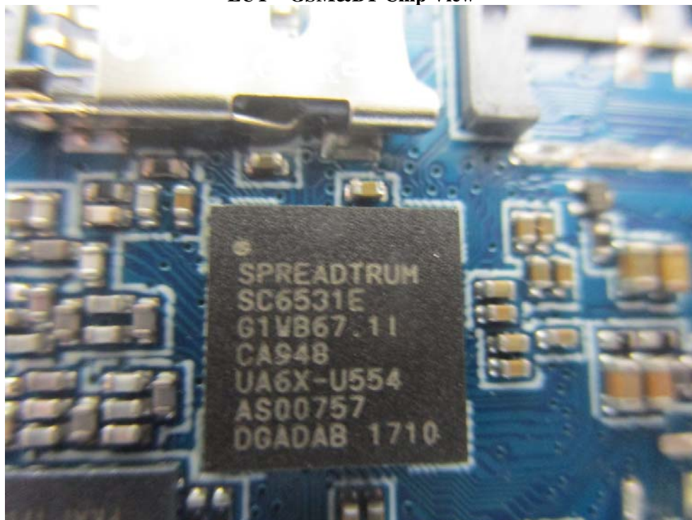
EUT – GSM&BT Chip View
