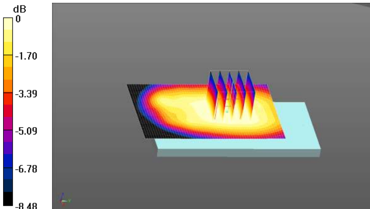
0 dB = 0.211 W/kg = -6.76 dBW/kg
