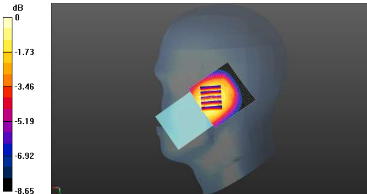
0 dB = 0.458 W/kg = -3.39 dBW/kg
