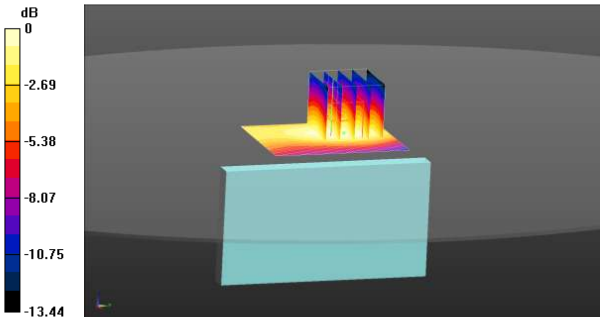
0 dB = 0.183 W/kg = -7.38 dBW/kg
