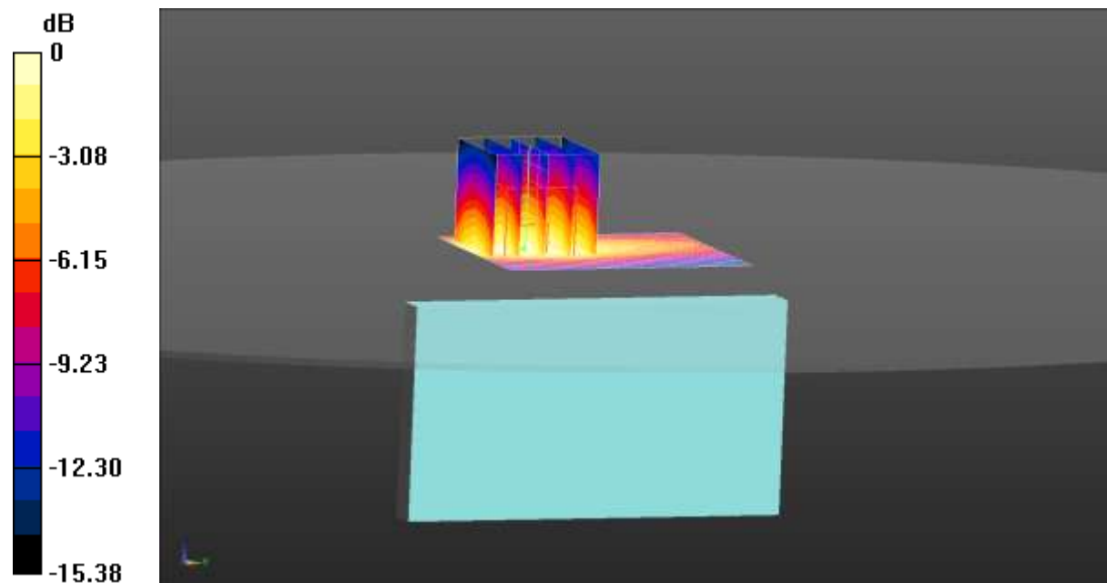
0 dB = 0.457 W/kg = -3.40 dBW/kg
