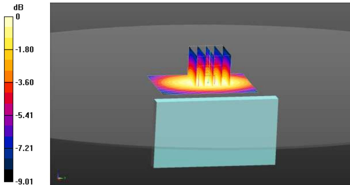
0 dB = 0.619 W/kg = -2.08 dBW/kg
