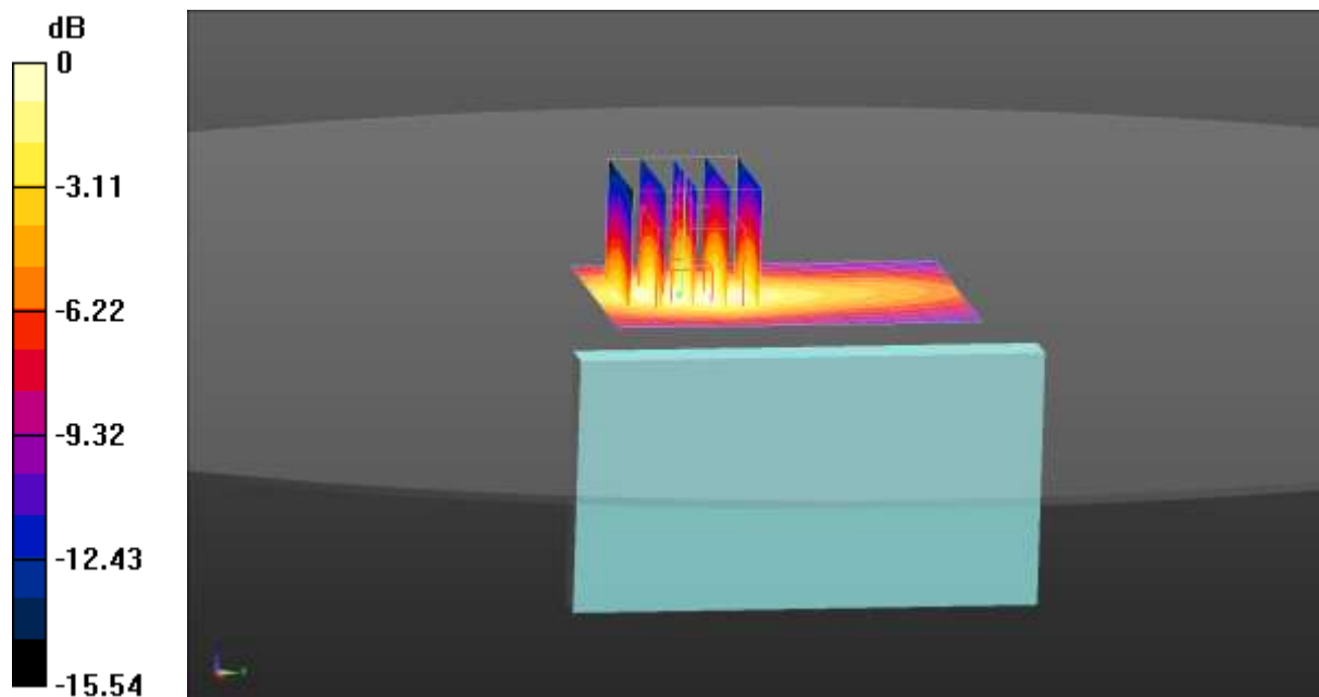
0 dB = 0.295 W/kg = -5.30 dBW/kg
