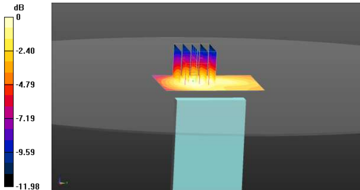
0 dB = 0.0622 W/kg = -12.06 dBW/kg
