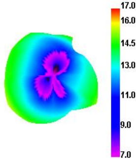
Wifi 1 TRP
