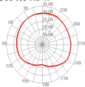
DCS 698 TRP H
