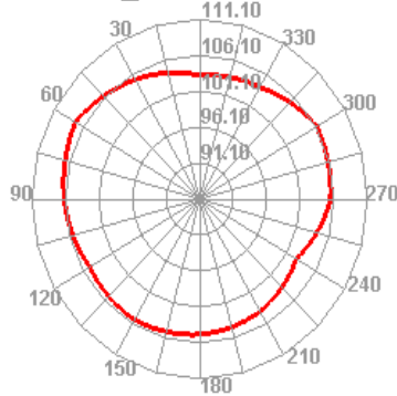
WCDMA_VIII 3088 TIS H
