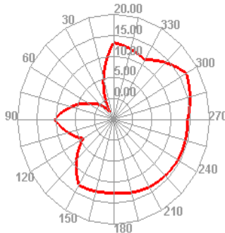
Wifi 64 TRP H
