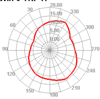
Wifi 6 TRP H
