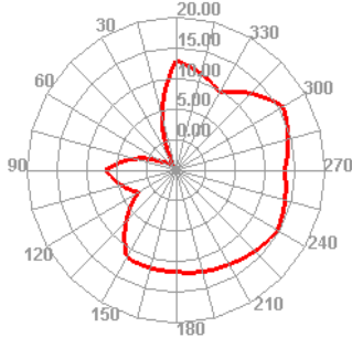
Wifi 36 TRP H
