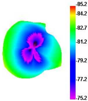
Wifi 1 TIS
