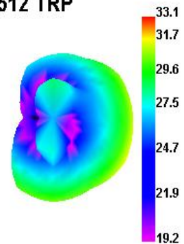
DCS 512 TRP
