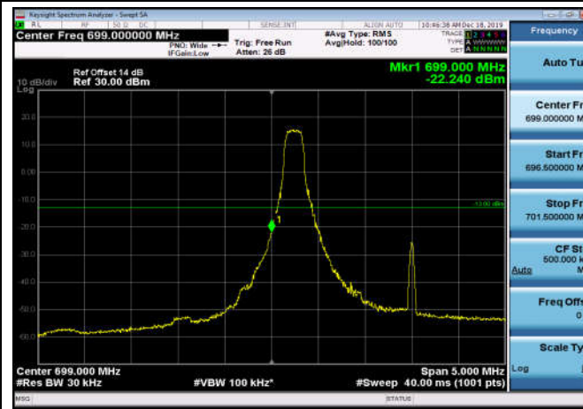
LowRange_FDD12_3MHz_700.5_fullIRB _Low_QPSK
