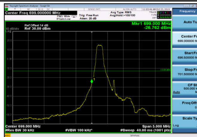
LowRange_FDD12_1.4MHz_699.7_fullIRB _Low_Q16
