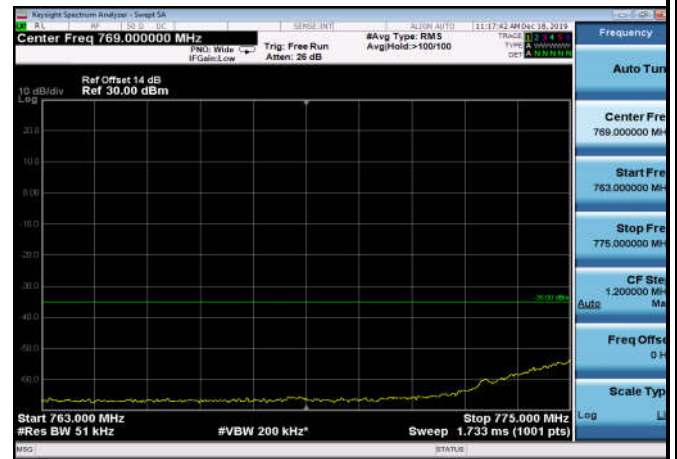
LowRange_FDD13_5MHz_779.5_fullIRB_Low_Q16
