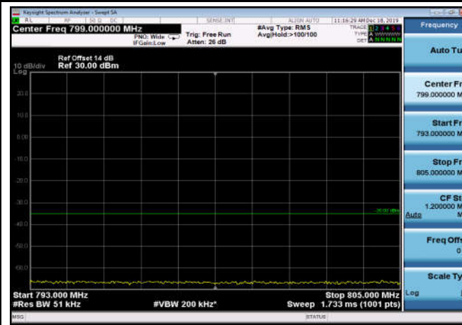
FDD13_5MHz_779.5_QPSK_OneRB_high_ExtraBands_Range_793~805
