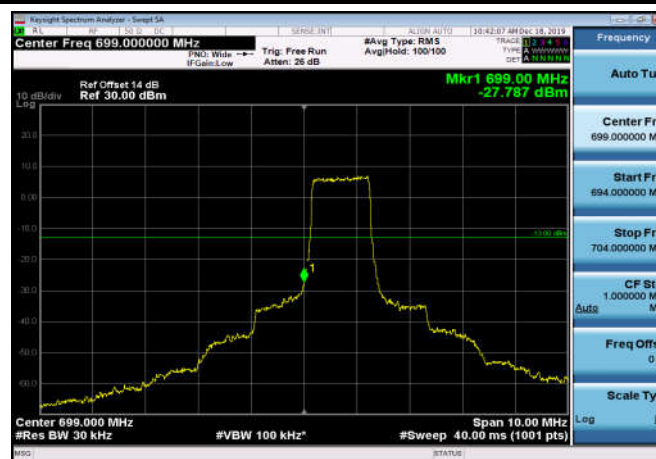
LowRange_FDD12_1.4MHz_699.7_fullIRB _Low_QPSK
