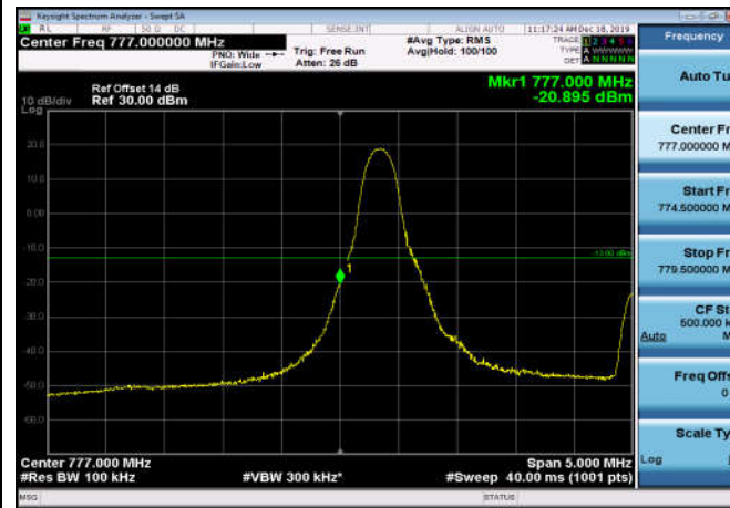
LowRange_FDD13_5MHz_779.5_fullIRB_Low_QPSK
