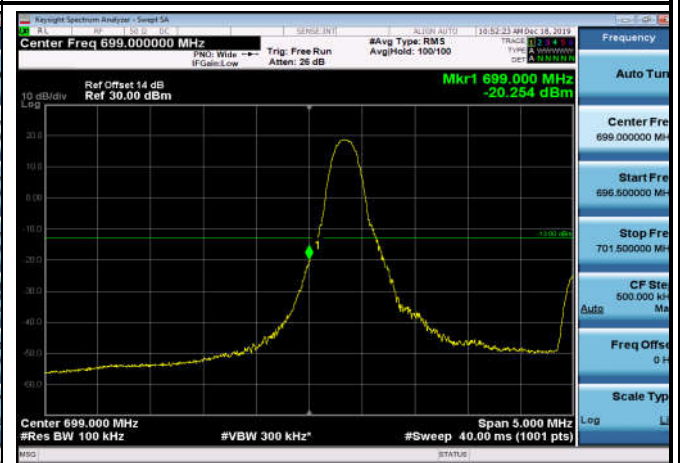
LowRange_FDD12_5MHz_701.5_OneRB _low_Q16
