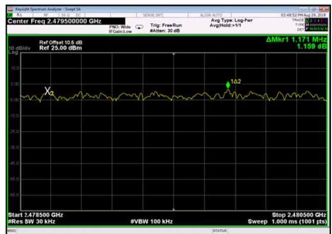
PI/4PI/4DQPSK,Hopping2DH5,2478.5~2480.5
