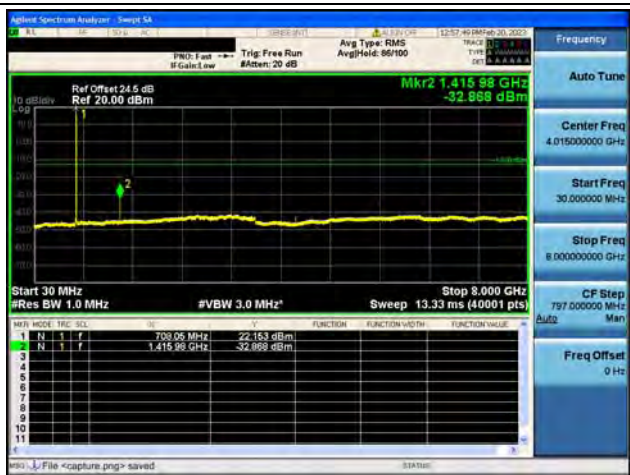
Band17 / 5MHz / Mid CH / 16QAM
