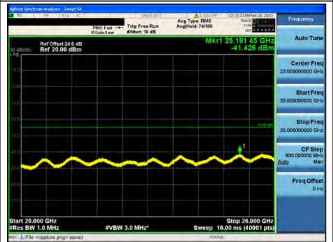
Band7-20G-26G / 5MHz / Mid CH / 16QAM
