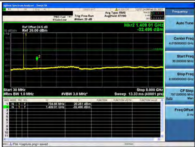
Band17 / 5MHz / Low CH / 64QAM
