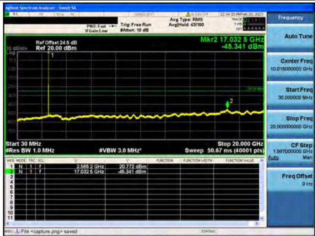
Band7-30M-20G / 5MHz / High CH / 16QAM
