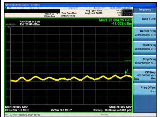
Band7-20G-26G / 10MHz / High CH / 64QAM
