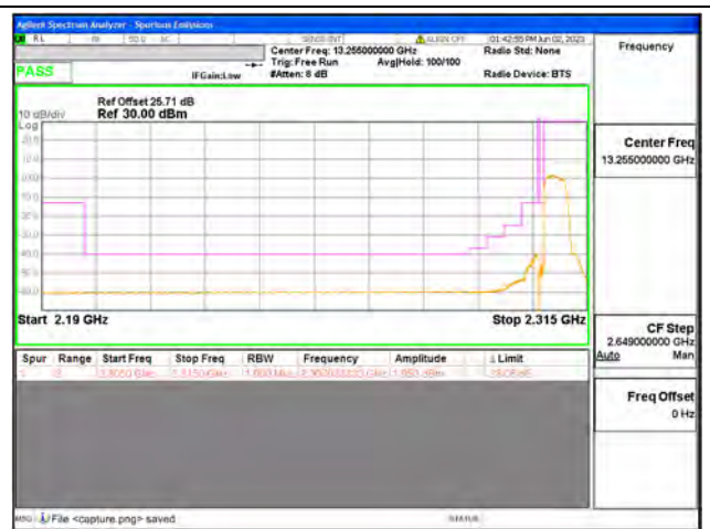
Band40-1 / 5MHz / Low CH / QPSK / FULL RB
