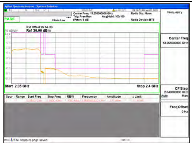
Band40-2 / 10MHz / High CH / QPSK / FULL RB
