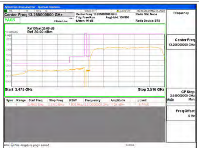
Band41 / 20MHz / Low CH / QPSK / FULL RB
