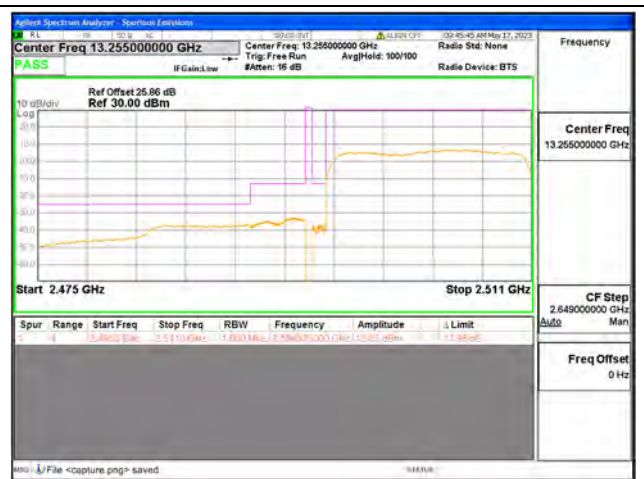
Band41 / 15MHz / Low CH / QPSK / FULL RB
