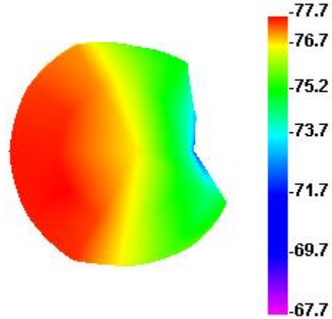
Wifi 165 TIS
