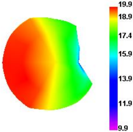
Wifi 165 TRP
