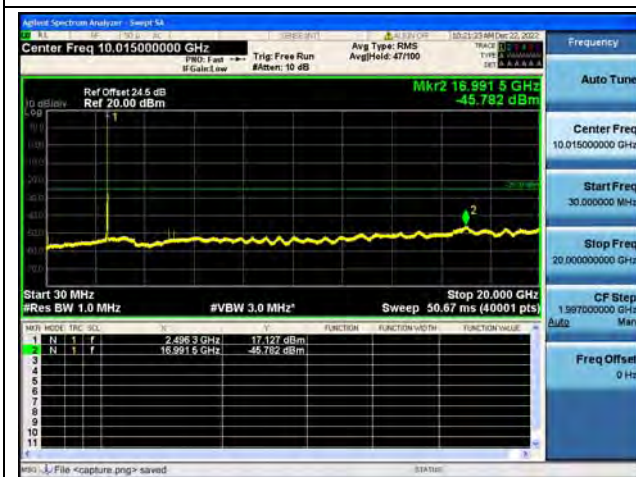
Band41-30M-20G / 15MHz / Low CH / 16QAM
