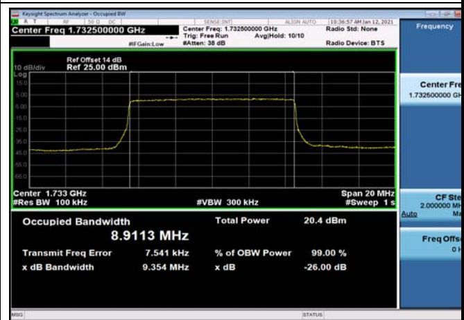
FDD04_MidRange_10_1732.5_QPSK
