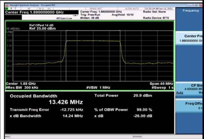
FDD02_MidRange_20_1880_QPSK
