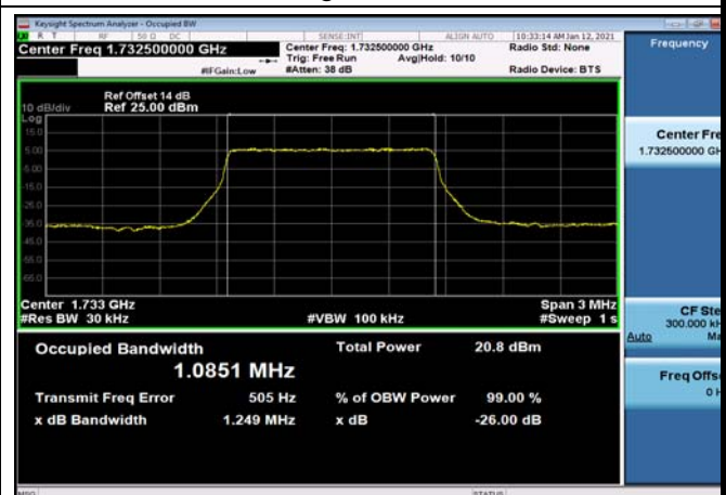
FDD04_MidRange_1.4_1732.5_QPSK
