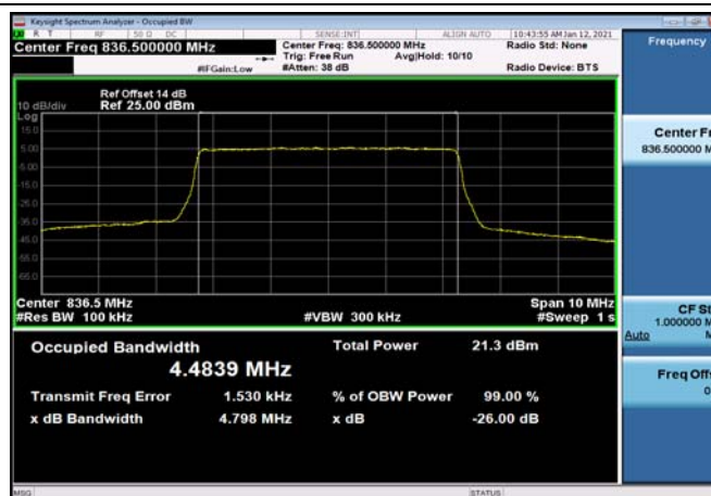
FDD05_MidRange_5_836.5_Q16
