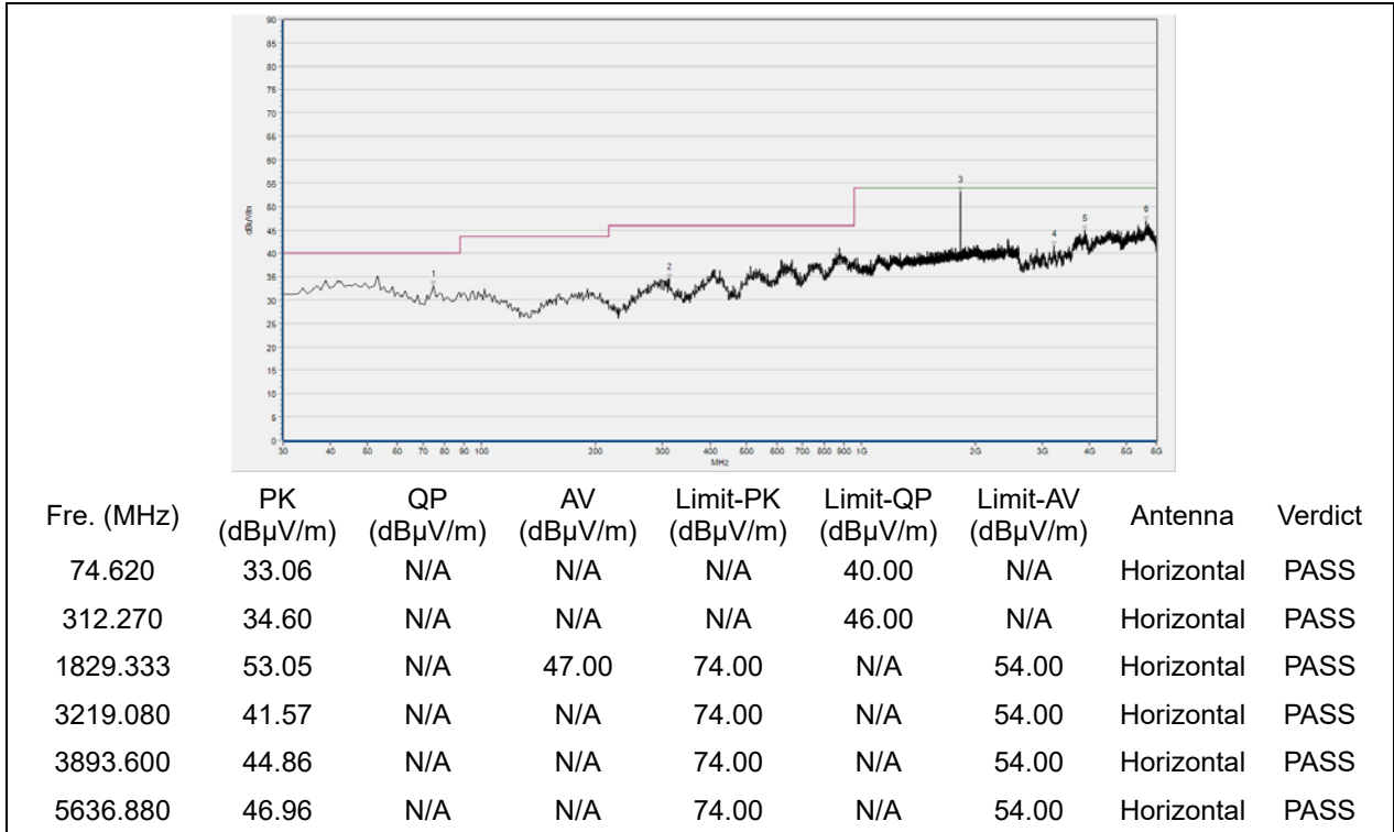
(Antenna Horizontal, 30MHz to 6GHz)
