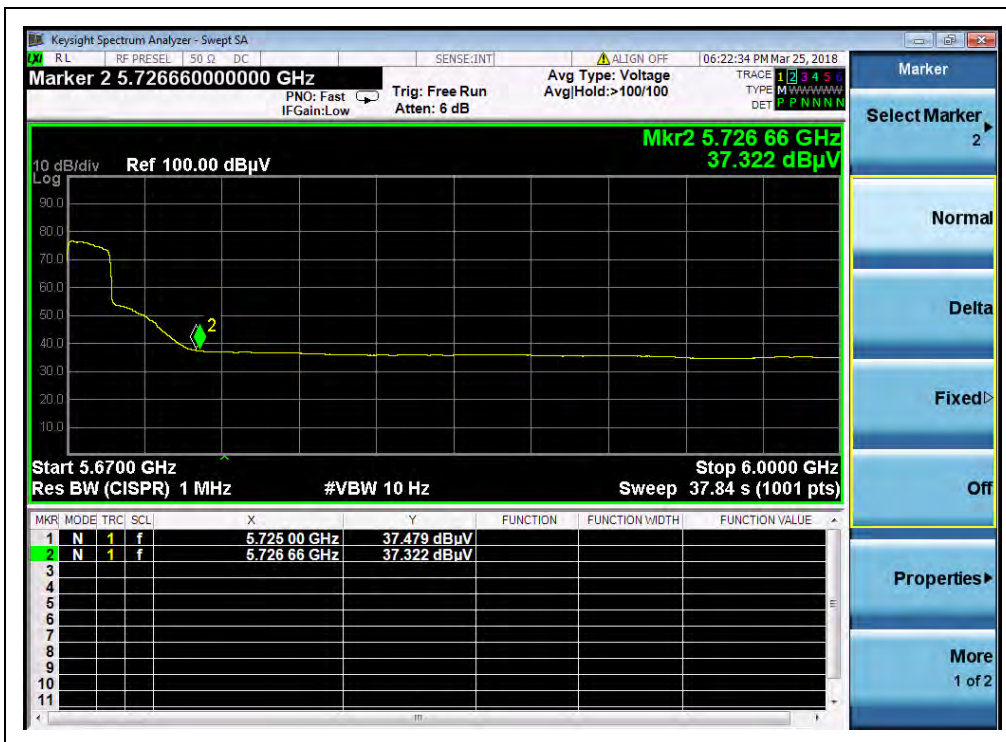
(Channel 134, AVG, 802.11n (HT40))
