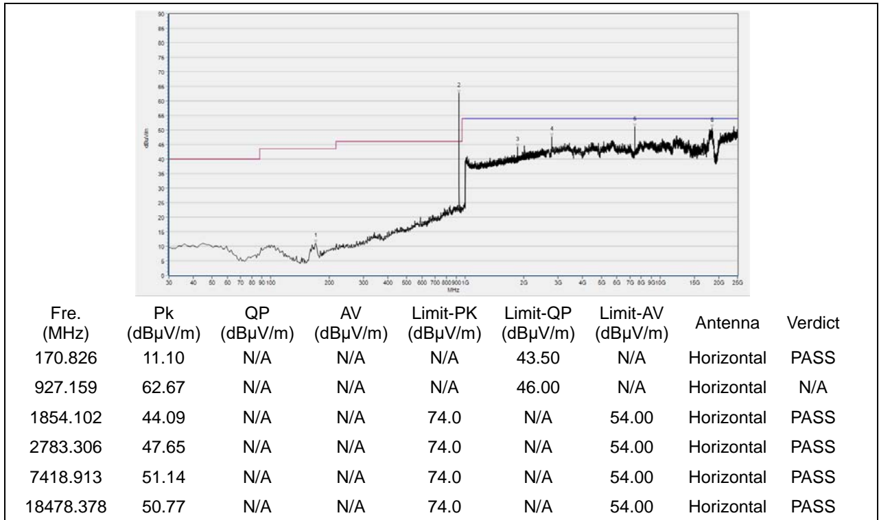
(30MHz to 25GHz, Antenna Horizontal, channel 78)
