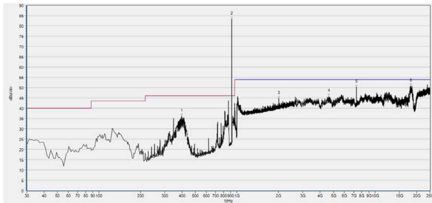
(30MHz to 25GHz, Antenna Horizontal, channel 39)
