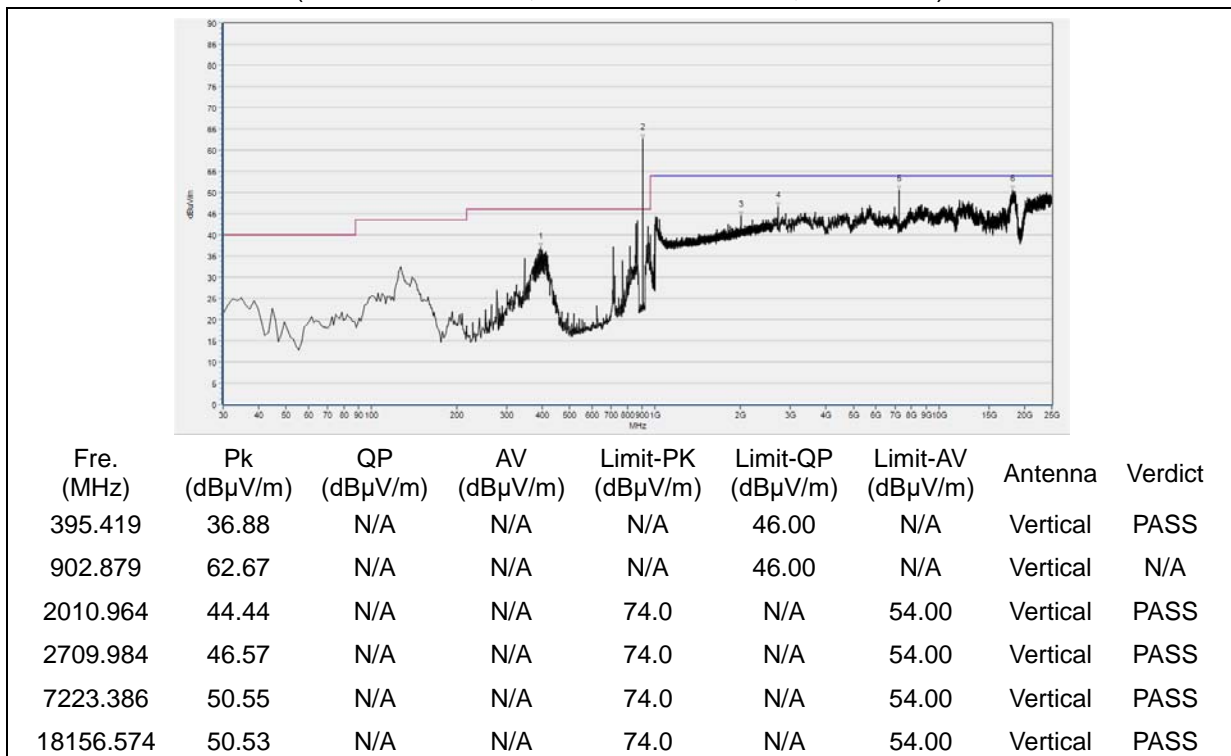
(30MHz to 25GHz, Antenna Vertical, channel 0)
