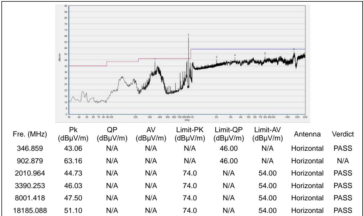
(30MHz to 25GHz, Antenna Horizontal, channel 0)
